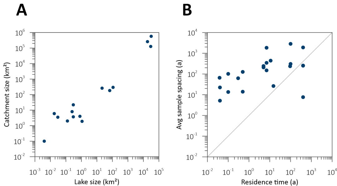
365 Figure 4. A) Depiction of corresponding lake and catchment sizes of the records compiled within this study. One lake may correspond to more than one record. Note that records from paleo-lakes and lakes with incomplete information on lake and catchment size were not considered for this figure (N=33). B) Depiction of corresponding sampling intervals and t_{res} . Note that records from lakes without information on t_{res} were not considered for this figure (N=37).
