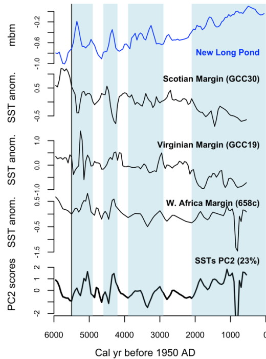
505 Figure 8. Comparison of the lake-level record from New Long Pond, Massachusetts (Fig. 3H), and three alkenone-inferred sea-surface temperature (SST) records (Adkins et al., 2006; Sachs, 2007). The SST records are shown after detrending and with the second principal component (PC2) scores of a PCA conducted on the non-detrended series; the first PC captures the trends. Blue bands represent the timing of wet phases identified from radiocarbon dated paleoshorelines at multiple lakes in coastal Massachusetts (Newby et al., 2014). “mbm” refers to meters below modern water level.
