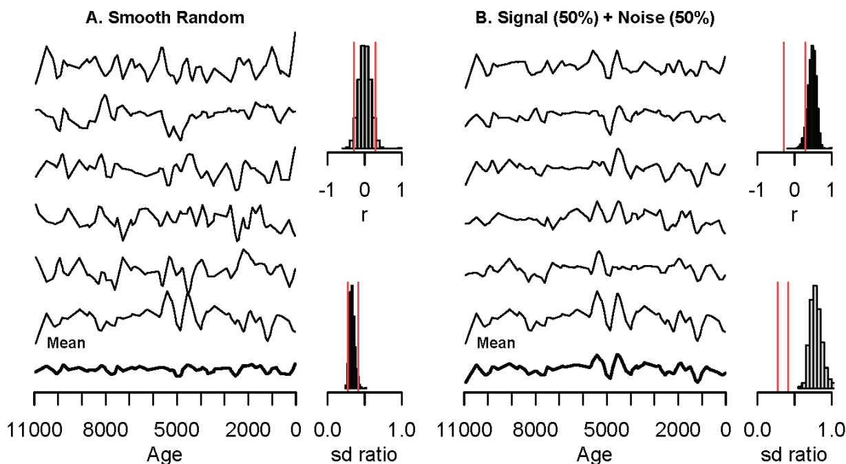
220 Figure 2 Simulated time series representing A) six white-noise series that have been smoothed to produce spurious oscillations with ~500-yr periods and B) six series as in A, but where the random series has been averaged with a common signal taken from the lower-most series in A. Bold lines at the bottom represent the means of the six series in each case. Histograms show (at the top) the Pearson's product moment correlation coefficients, r , between the means and 1000 similarly generated random (A) or non-random (B) time series, and (at the bottom) the ratio of the standard deviation (sd) of each mean and each of the 1000 simulated series. Red lines show the 95% distributions of the values for the random series.
