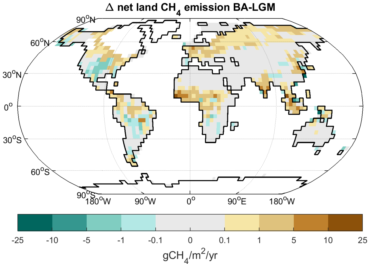
Figure 5. Change in net land CH 4 emissions between LGM (20 ka BP) and BA (13.2 ka BP) in MWM experiment. Shaded areas indicate LGM land points, continental outline is from 13.2 ka BP.
