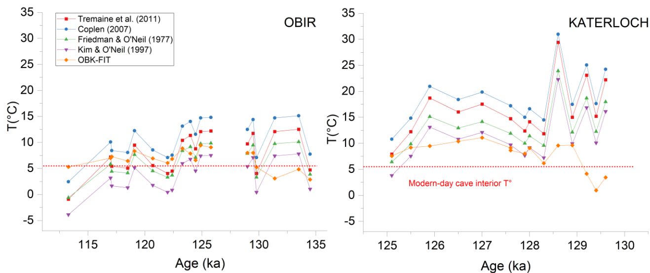
330 Figure 5: Results of paleotemperature calculations for Obir and Katerloch using the LMWL of Klagenfurt and Graz, respectively, based on \delta^2\text{H} data converted to \delta^{18}\text{O}_{\text{FI-Calculated}} using four different water-calcite isotope fractionation equations (in red, blue, green and purple). The orange data show the results of the water isotope-air temperature relationship \delta^2\text{H}/\text{T} (OBK-FIT). The red dashed line indicates the modern cave interior temperature.
