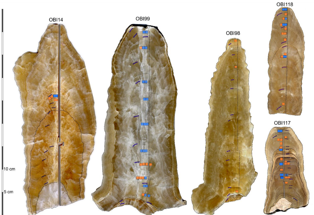
Fig. A4: Scans of the longitudinal cross-sections of the Obir cave stalagmites showing hand-drilled (thin black dotted lines) and micromilled traces for stable isotopes (vertical grey bars), samples for ^{230}\text{Th} dating (purple dots), and fluid inclusions (blue squares (data presented in Table 1) and orange squares (samples yielding <0.1 \mu\text{L} of water)). Note that the fluid-inclusions samples were taken on the opposite half of the respective stalagmite slabs.
