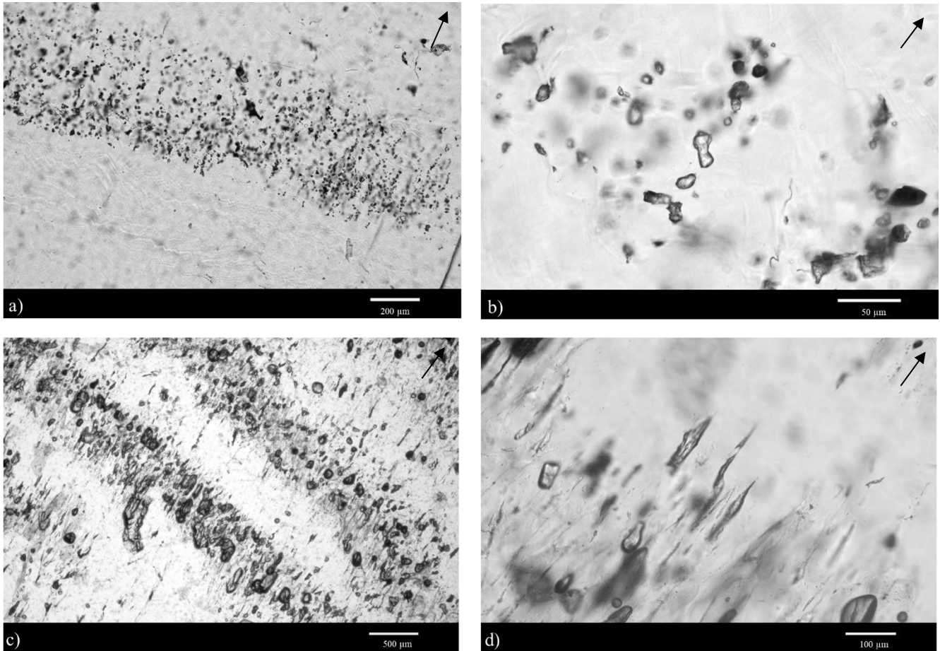
180 Figure 2: Transmitted-light images of fluid-inclusion assemblages in the studied speleothems. a) Primary fluid inclusions along growth layers in stalagmite OBI99, b) intracrystalline fluid inclusions in sample OBI99, c) primary inclusion-rich and inclusion-poor growth layers in stalagmite K2, d) inter-crystalline elongated inclusions in sample K2. The black arrows indicate the growth direction.
