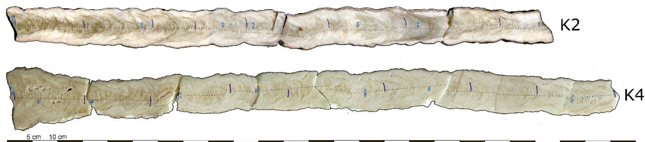
Fig. A5: Scan of the longitudinal cross-sections of the studied Katerloch stalagmites, with the sampling trace for stable isotopes (dotted black lines), ^{230}\text{Th} dating (purple dots), fluid inclusions (blue squares; data presented in Table 1). Note that the fluid-inclusion samples were taken on the opposite half of the respective slabs.
