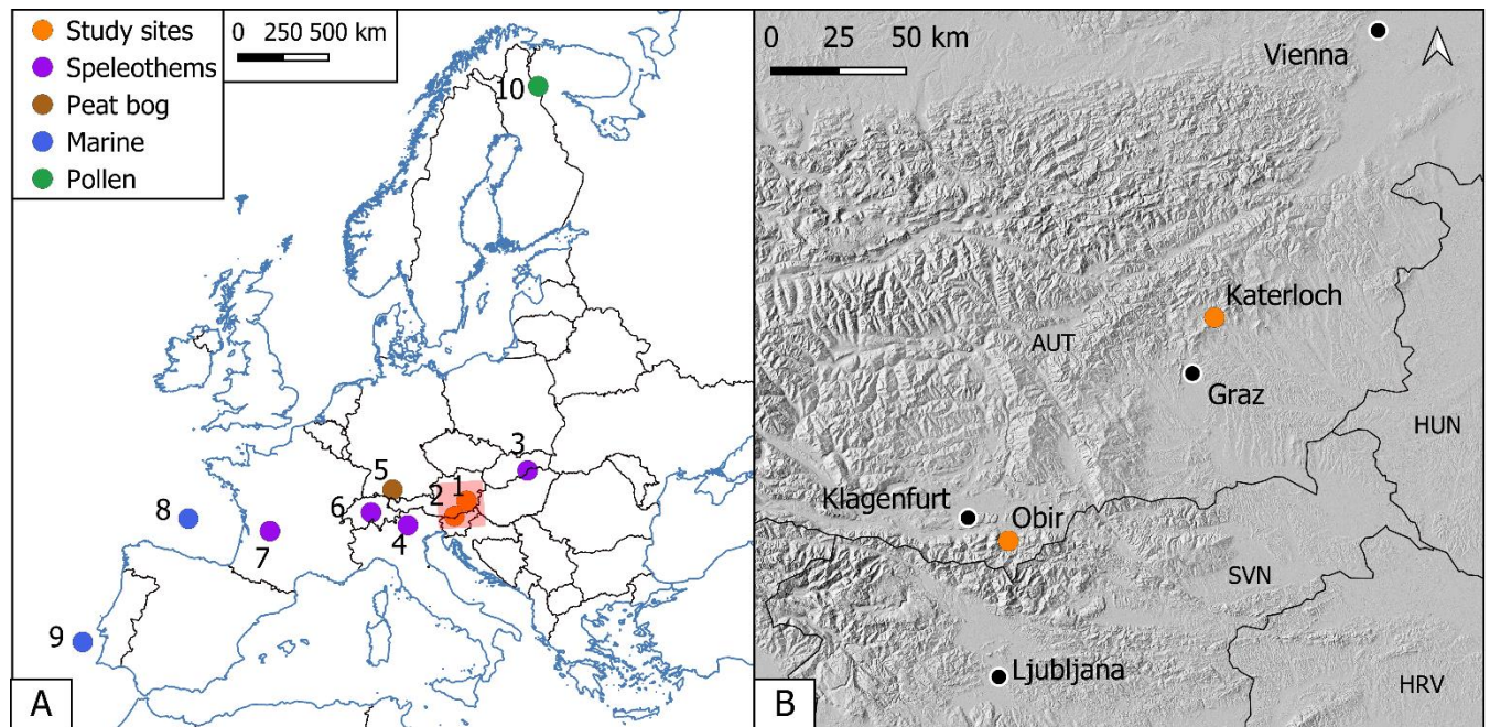
80 Figure 1: (A) Location of the study sites (1) Katerloch and (2) Obir and other sites from which paleoclimate data for the LIG are mentioned in the text: (3) Baradla cave (Demény et al., 2017, 2021), (4) Cesare Battisti cave (Johnston et al., 2018), (5) Fűramoos (Bolland et al., 2021), (6) Melchsee-Frutt caves (Wilcox et al., 2020), (7) Villars cave (Wainer et al., 2011), (8) deep-sea cores MD04-2845 (Sánchez Goñi et al., 2018; Salonen et al., 2021) and (9) MD01-2444 (Tzedakis et al., 2018), (10) pollen sequence from Sokli (Salonen et al., 2018). The transparent red square in A marks the enlarged digital elevation map shown in B.
