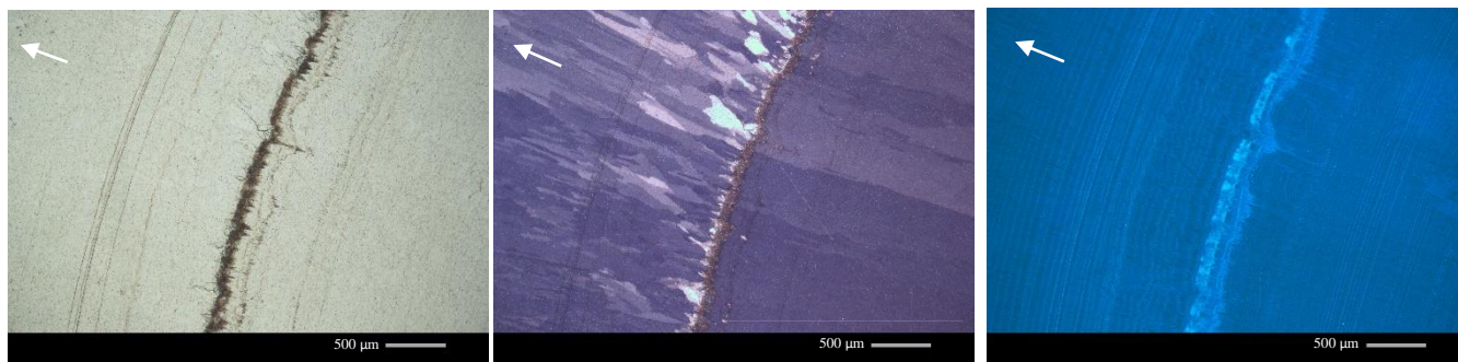
515 Fig. A6: Thin-section photomicrographs of the hiatus between 130.3 \pm 0.9 ka and 129.2 \pm 0.8 ka in stalagmite OBI117. Note nucleation event followed by re-growth of calcite crystals. Parallel (left) and crossed nicols (middle) and epifluorescence image (right). The white arrows indicate the growth direction.
