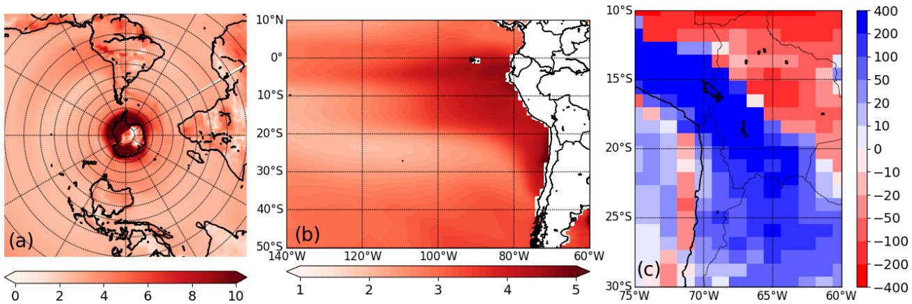
95 Figure 2: Changes (mid-Pliocene minus historical) for mean annual (a) near-surface air temperature (at 2m above ground in °C), (b) sea-surface temperature (in °C), and (c) rainfall (in mm·yr -1 ) as simulated by the global CESM2 model.
