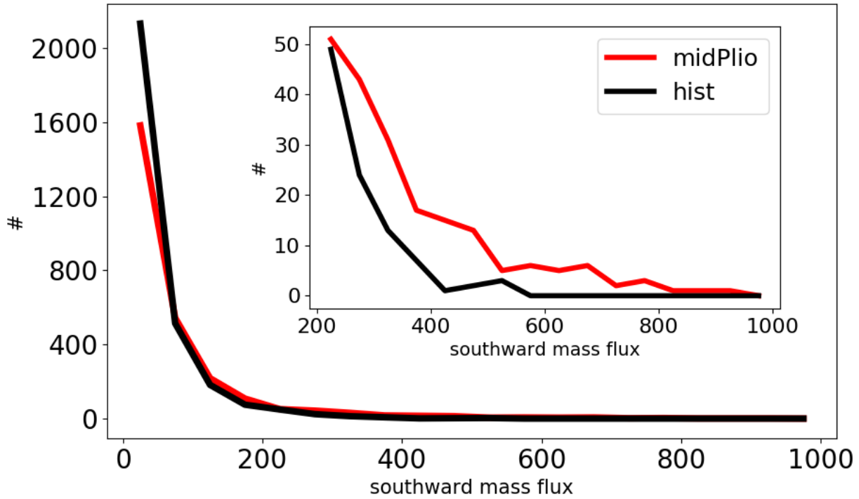
Figure 7: Probability density function (y-axis, in total number # of dates) of 12-hourly southward upper-level (above 2000m agl.) I WV mass fluxes (x-axis, in 10^6 \cdot \text{kg} \cdot \text{s}^{-1} ) integrated between 80^\circ\text{W} and 70^\circ\text{W} at 20^\circ\text{S} (see yellow line in Fig. 5a) in \text{WRF}_{\text{mP}} and \text{WRF}_{\text{hist}} (outer model domain with 50 km resolution) for Southern Hemisphere winter. The inset zooms into the results above 200 \cdot 10^6 \cdot \text{kg} \cdot \text{s}^{-1} .
