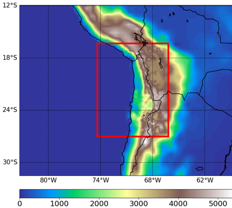
85 Figure 1: Map showing the outer (with 50 x 50km resolution) and inner WRF model domain (red box, with 10 x 10km resolution) and the topographic heights (shading, in m).
