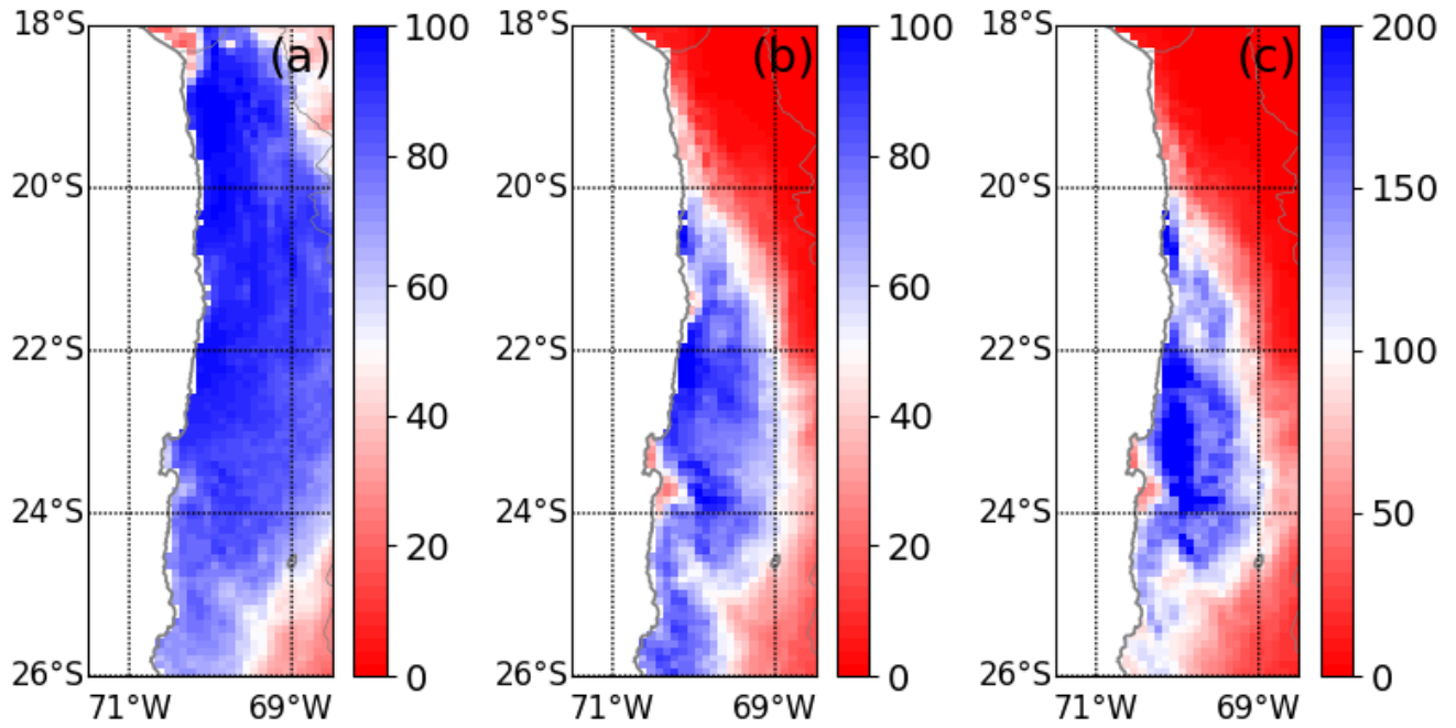
85 Figure 10: Fraction (in %) of the rainfall associated with MCB cluster 4 and 6 of WRF mP to (a) total winter rainfall in WRF mP , (b) total annual rainfall in WRF mP , and to (c) total annual rainfall in WRF hist (inner model domain with 10 km resolution).
