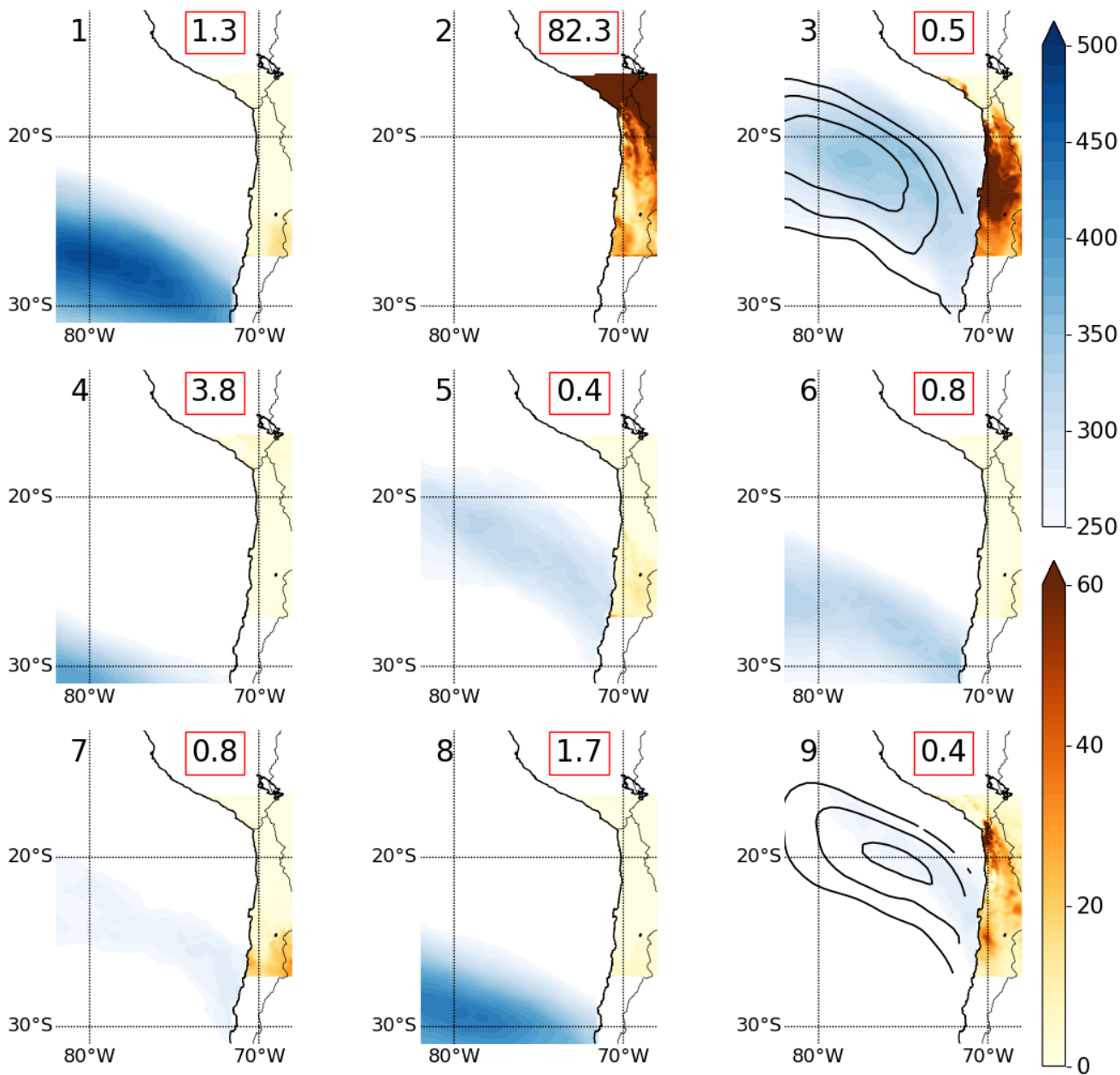
75 Figure 9: As Fig. 8, but for WRF_{hist} . The black contours in cluster 3 and 9 show the composite mean wind speed in 4000 m asl. (15, 17, and 19 m \cdot s^{-1} ).
