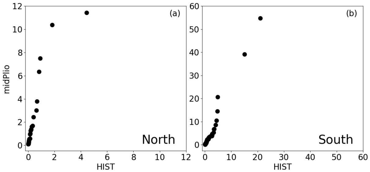
Figure 4: Percentile-percentage plots for daily winter rainfall (in \text{mm}\cdot\text{day}^{-1} ) in \text{WRF}_{\text{mP}} (y-axis) against \text{WRF}_{\text{hist}} (x-axis) as spatial means over (a) the northern box and (b) the southern box, marked in Fig. 3n.
