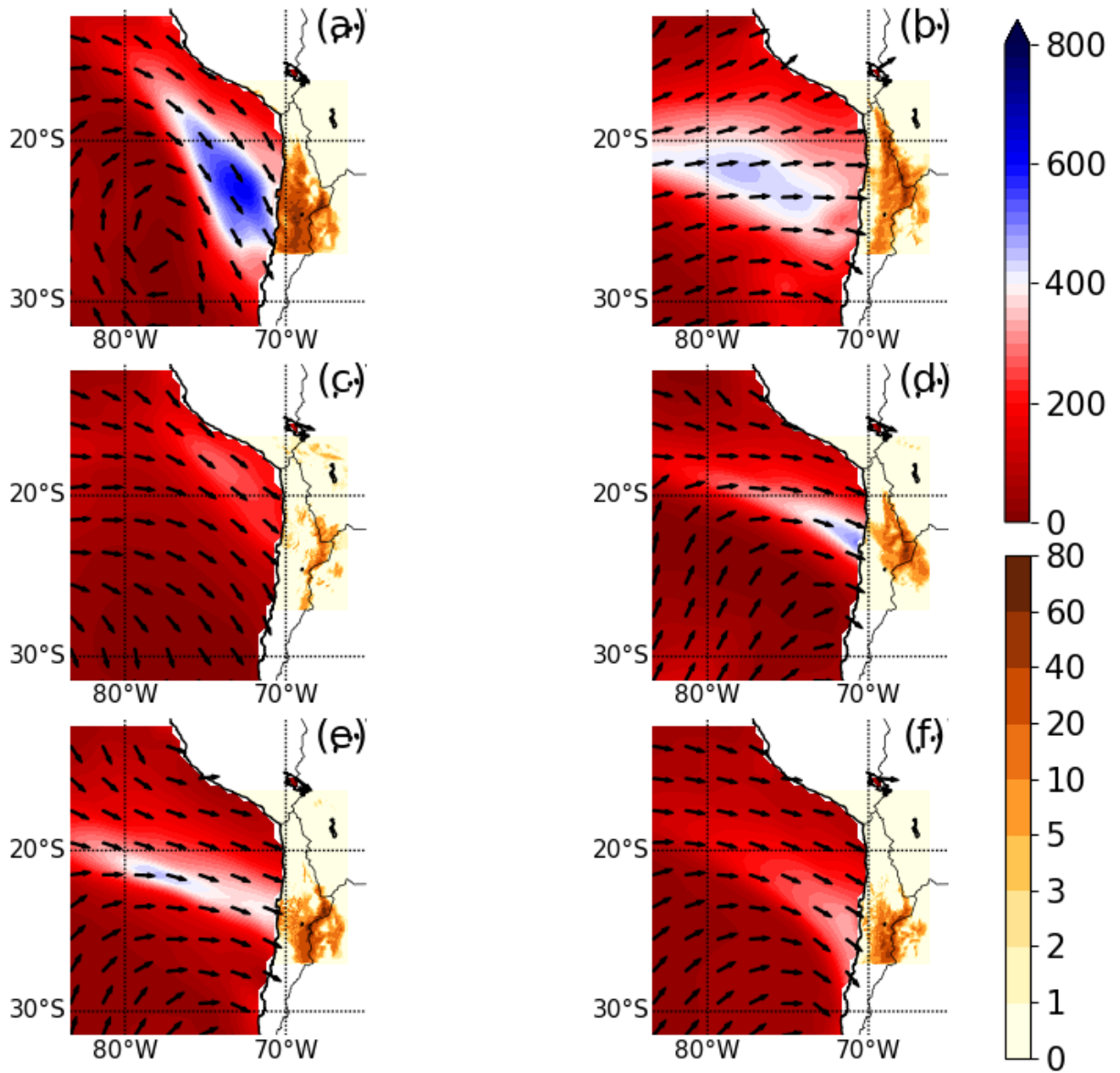
Figure 6: As Fig. 5, but for the top winter events in WRF_{\text{hist}} .
