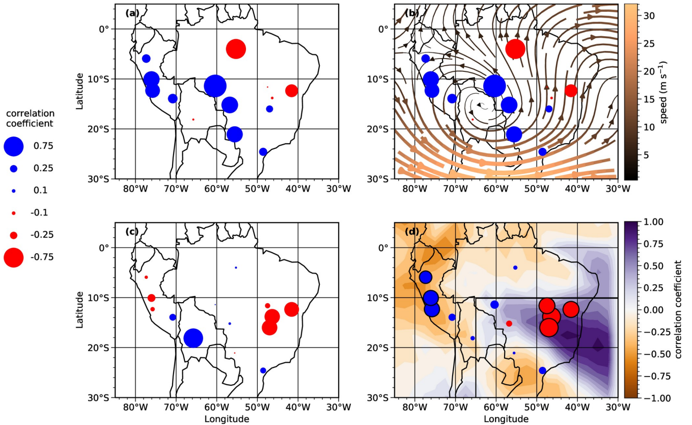
350 Figure 4: MCEOF patterns and their corresponding dynamic interpretations. a) MCEOF1 loadings; b) upper-level (200 hPa) DJF streamlines from ERA5 reanalysis (1979–2019); c) MCEOF2 loadings; d) spatial correlation of DJF OLR field with the PC1 of OLR variability derived from the SACZ region (black box). Colored circles indicate the correlation of local precipitation derived from station data with PC1 of the OLR decomposition over the SACZ region.
