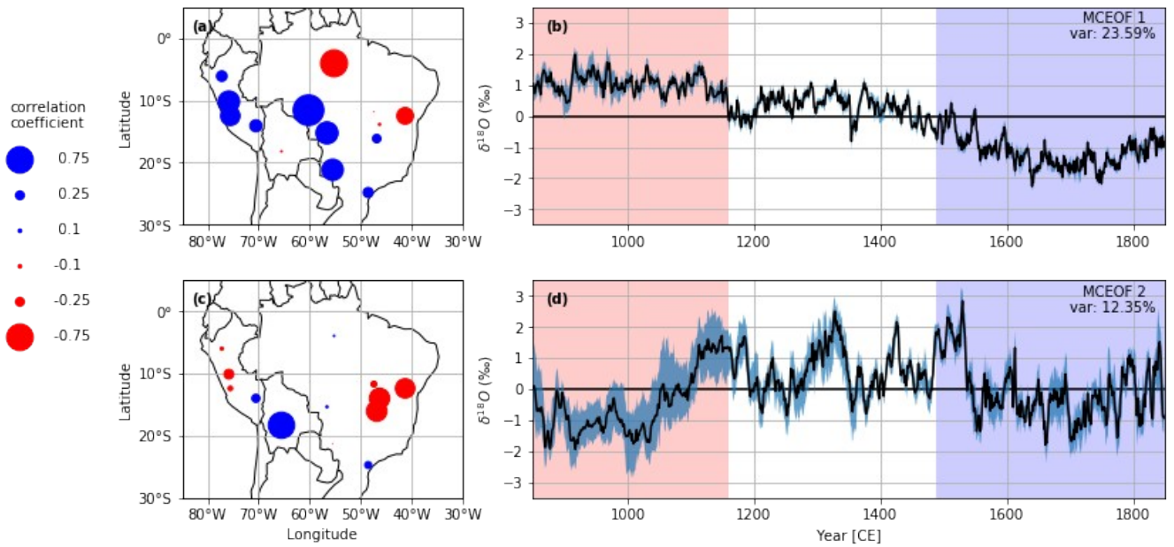
Figure 2: MCEOF decomposition of the oxygen isotope proxy network. a) MCEOF1. The magnitude of the loadings in the spatial patterns represent the correlation coefficient between the median of the Monte Carlo ensemble of proxy records at those locations and the corresponding principal component (PC) time series for that mode; b) PC1. Blue shading indicates the total envelope of ensemble variability; c) same as in a) but for MCEOF2; d) same as in b) but for PC2. Pink/blue shading in b) and d) highlight the MCA/LIA periods, respectively.
