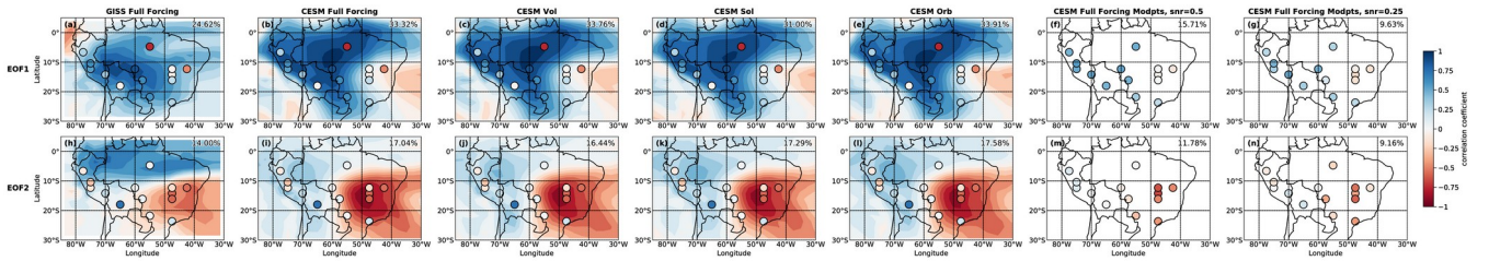
Figure 3: Comparison of model-derived modes (shading) overlaid with proxy-derived modes (circles) of isotopic variability. Color shading indicates the correlation of the EOF loadings with the corresponding PC time series. Models plotted are a) EOF1 from GISS full forcing experiment, b) as in a) but for iCESM full forcing experiment, c) as in a) but for iCESM volcanic forcing experiment, d) as in a) but for iCESM solar irradiance experiment, e) as in a) but for iCESM orbital forcing experiment, f) iCESM PPE EOF1 with signal-to-noise ratio = 0.5, g) as in f) but for signal-to-noise ratio = 0.25. h-n) as in a-e) but for EOF2. 315
