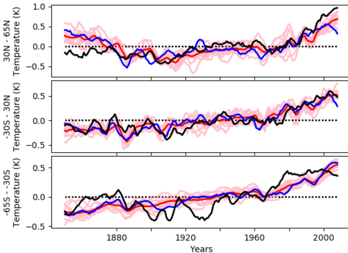
315 Figure 8 – Mean annual surface air temperature averaged over three latitudinal bands Assimilated model (green/blue), 10 forcing-only simulations (light pink), forcing-only ensemble mean (red), observations (HadCRUT5; black). All timeseries filtered using a 5-year running mean.
