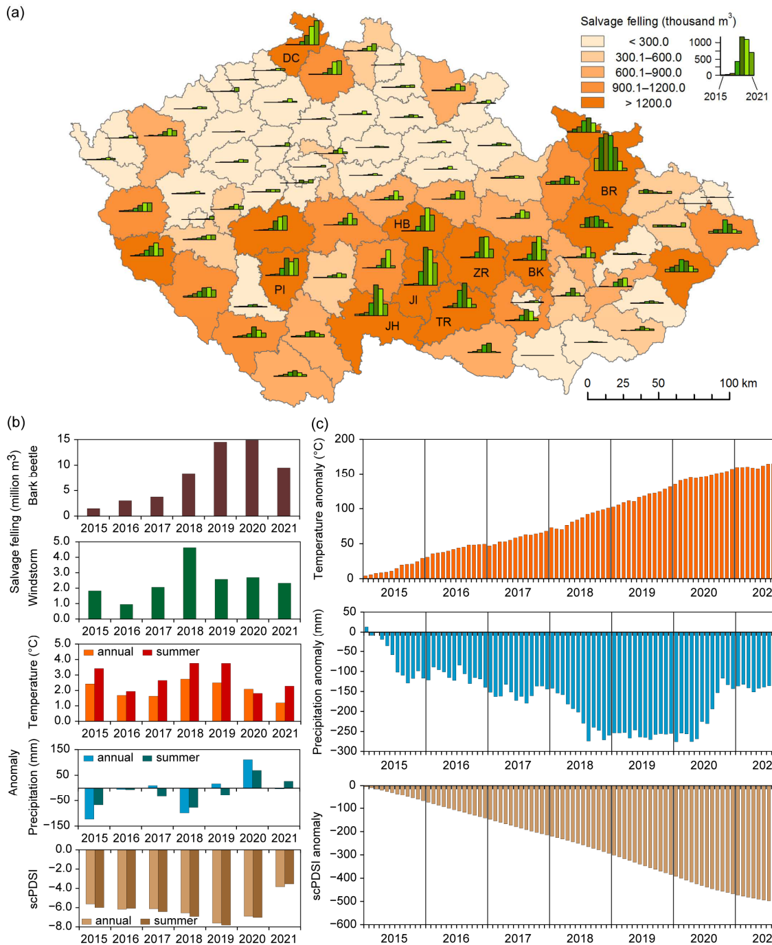
940 Figure 10: Bark beetle outbreak of the 2010s–2020s on the territory of the Czech Republic: (a) the volume of bark beetle salvage felling in 2015–2021 in individual districts; (b) annual bark beetle and windstorm salvage felling, annual and summer anomalies of temperature, precipitation, scPDSI-12 and scPDSI-3 in 2015–2021; (c) monthly cumulative anomalies of temperature, precipitation and scPDSI in 2015–2021 (1961–1990 reference period). Abbreviations of districts: BK – Blansko, BR – Bruntál, DC – Děčín, HB – Havlíčkův Brod, JH – Jindřichův Hradec, JI – Jihlava, PI – Písek, TR – Třebíč, ZR – Žďár nad Sázavou.
