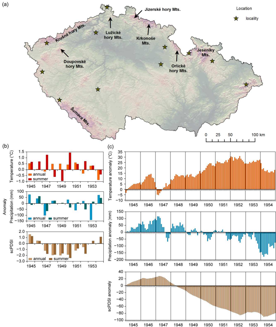
920 Figure 6: Bark beetle outbreak of the 1940s–1950s on the territory of the Czech Republic: (a) location of regions and localities with the occurrence of bark beetle; (b) annual and summer anomalies of temperature, precipitation, scPDSI-12 and scPDSI-3 in 1945–1954; (c) cumulative monthly anomalies of temperature, precipitation and scPDSI in 1945–1954 (1961–1990 reference period).
