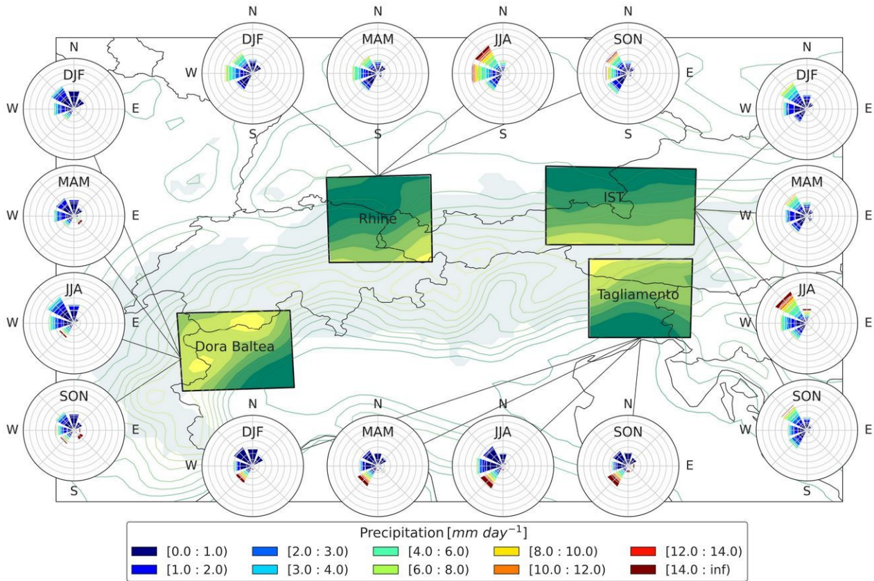
315 | Figure 5: 21 ka BP seasonal wind origins associated to with each of the 19 simulated years' precipitation events. This has been done for Rhine, Inn-Salzach-Traun (IST), Tagliamento and Dora Baltea glacier subdomains. Windroses show the main wind directions under the condition that precipitation events occur. Colours represent precipitation intensity in millimetres and colour-band width is the frequency of a given precipitation intensity per wind direction. The shadow in the map is the glacier extension (Ehlers et al., 2011), the colour lines, as well as the full colour in the boxes, represent the topography (yellow for higher elevation and green for the lowers), and the black line is the present-day political boundary.
