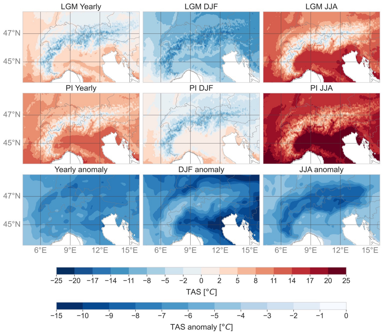
Figure 3: 21 ka BP and PI temperature and anomaly. Yearly, winter and summer averaged over 19 years-long RegCM4 bias-corrected temperatures data.
