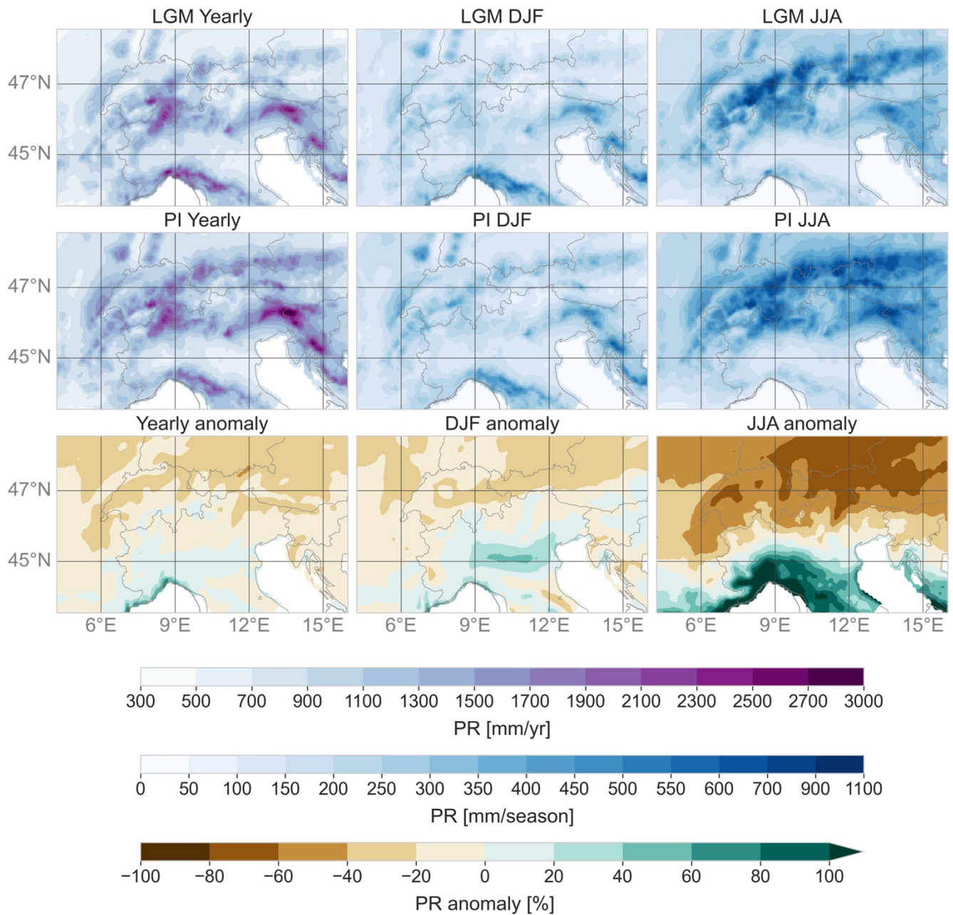
290 Figure 4: 21 ka BP and PI precipitation and anomaly. Yearly, winter and summer averaged over 19 years-long RegCM4 bias-corrected precipitation data.
