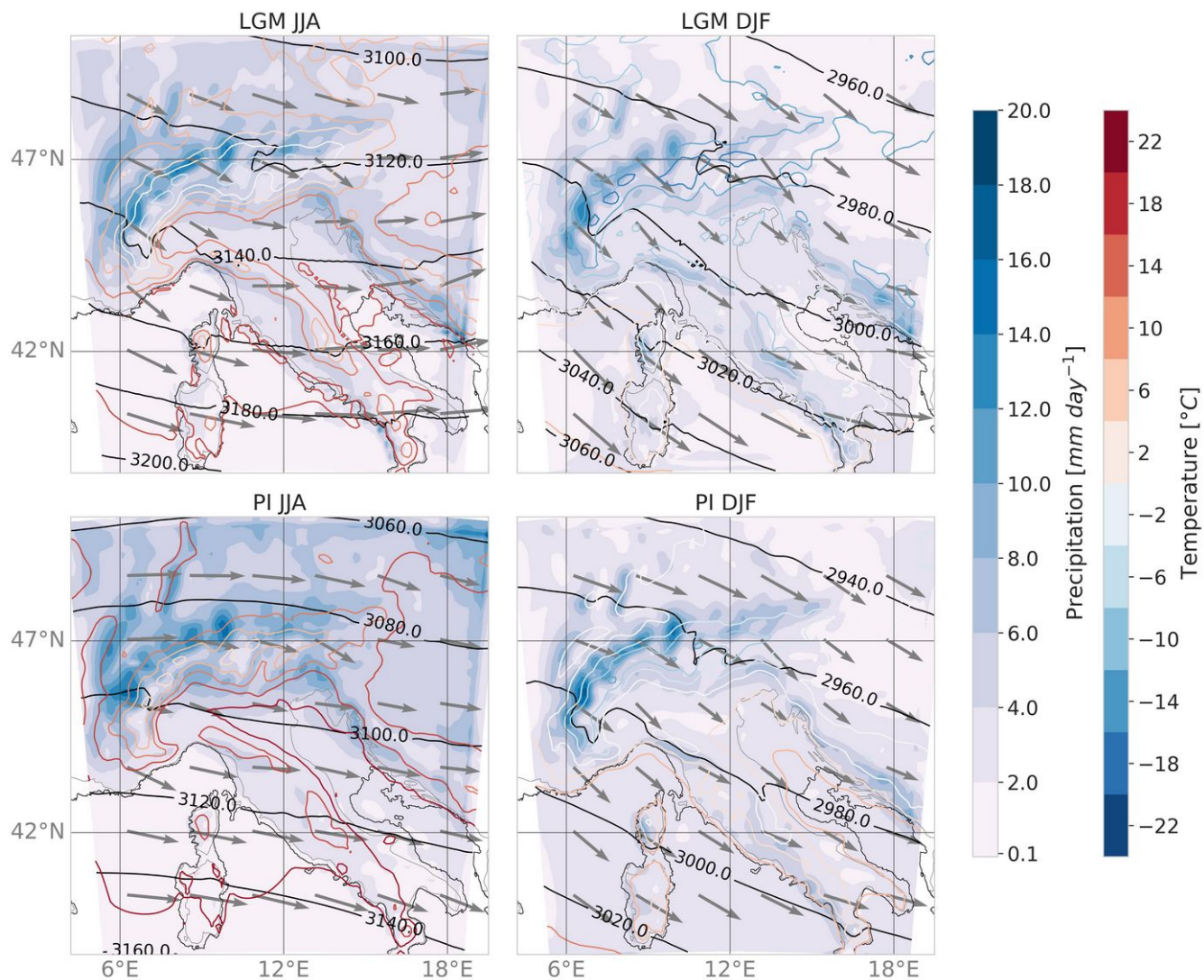
280 Figure 2: 21 ka BP and PI mean winter-summer and mean winter-summer synoptic conditions averaged over 19 years. In the first row: 21 ka BP 700 hPa average wind field (arrows) and, temperature (blue to red lines), precipitation (blue scale). In the second row: Temperature – and 700 hPa geopotential (black lines). Temperature and precipitation are not bias-corrected. These data represent the average summer and winter situation.
