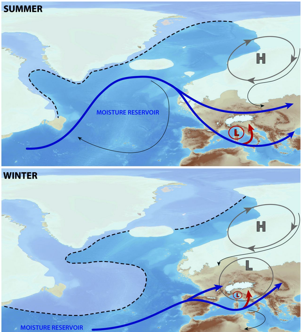
530 Figure 7: Conceptual model of the air masses yielding precipitation in the Alps at 21 ka BP. In white glaciers and ice sheets; the black line marks the 50% sea ice concentration extension (Paul et al., 2020; Rhines and Huybers, 2014); H and L stand for high-pressure and low-pressure system; blue and red arrows represent the air masses leading precipitation on the Alps; grey lines represent other air masses not leading precipitation on the Alps. Blue and grey arrows are extrapolated from the mean winter and summer MPI-ESM 850 hPa winds; while the red symbols show the elements that emerged from the RegCM4 simulations.
