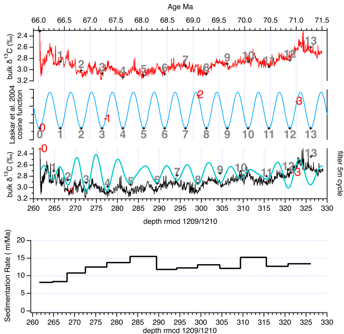
485 Figure 3: (top) Basic 405 kyr age model was first made by assigning Shatsky Rise Sites 1209 and 1210 composite bulk \delta^{13}\text{C} to known 490 tie points (red numbers). Then, 5 m filter (bandpass 0.2 \pm 0.06 ) of bulk \delta^{13}\text{C} composite was modelled to know the cosine function (cyan line). This cosine function was correlated to La2004 Cosine function (Laskar et al., 2004; blue line) minima for tuning the depth to the stable 405 kyr cycle for an age. New age is tie points in Supplement Table S4. (bottom) Sedimentation rate in meters per million years (m/Ma) of composite depth (rmcd).
