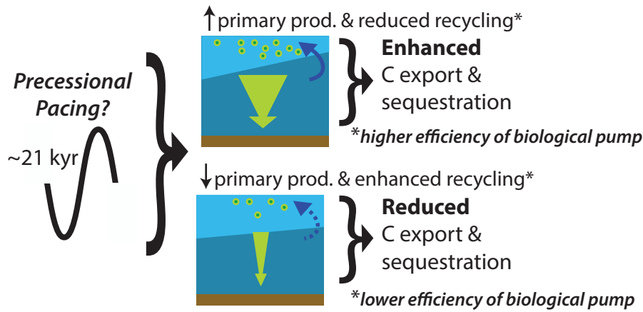
530 Figure 7: Cycles of enhanced and reduced carbon (C) export and sequestration result from precessional paced variations in primary productivity and recycling in surface waters (i.e., changes in the efficiency of the biological pump). A shallower thermocline (steeper boundary between light and dark blue waters) would result in increased primary production and reduced recycling in the surface waters due to changes in water column stratification, continental nutrient fluxes and upwelling intensity which increases nutrients (solid blue arrow) and enhances C export out of the surface waters (wide green arrow). A deeper thermocline (near horizontal boundary between light and dark blue waters) would result in reduced primary production and enhanced recycling in the surface waters due to reduced nutrient availability (dashed blue arrow) and reduces C export out of the surface waters (thin green arrow). 535 This ENSO-like variability could have controlled carbon export in the Maastrichtian.
