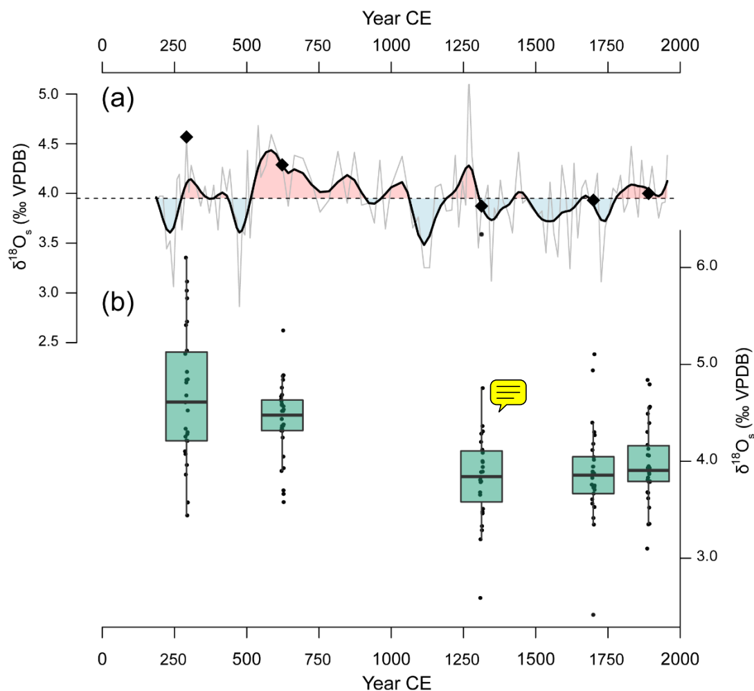
Figure 3: Arthritica helmsi oxygen isotope ratios from core C18 plotted against time. In (a) the grey line represents a bulk measurement ( n = 5 ) from each centimetre of C18. The dashed line indicates the mean of all values and the bold line is a smooth spline ( \text{spar} = 0.4 ). Blue shading indicates periods of below mean \delta^{18}\text{O}_s , while the red shading indicates periods of above mean \delta^{18}\text{O}_s . Black diamonds indicate where data from multiple individuals ( n \geq 27 ) are incorporated into the bulk curve. (b) Boxplots of oxygen isotope ratios of A. helmsi shells. Data are obtained from analyses of multiple individual shells from depths corresponding to age 300 ( n = 30 ), 631 ( n = 29 ), 1321 ( n = 27 ), 1708 ( n = 30 ) and 1899 years CE ( n = 27 ).
