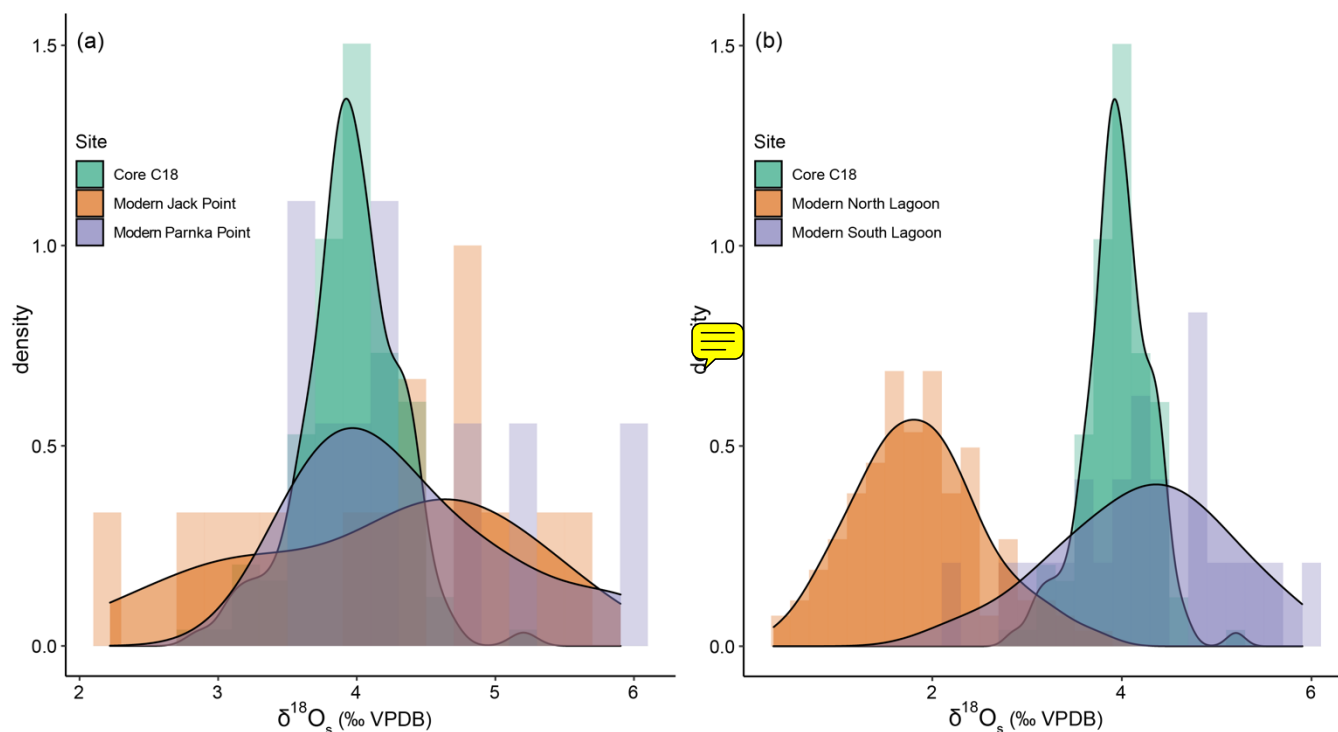
615 Figure 5: Density plots with histograms of A. helmsi \delta^{18}\text{O}_s comparing values from core C18 with (a) modern locations in the South Lagoon and (b) the North and South Lagoon. Modern \delta^{18}\text{O}_s values for the North Lagoon are sourced from Chamberlayne et al. (2021). \delta^{18}\text{O}_s values for the modern South Lagoon sites Jack Point and Parnka Point are calculated from temperature and \delta^{18}\text{O}_w values from Chamberlayne et al. (2021) using the oxygen isotope fractionation equation developed in that study.
