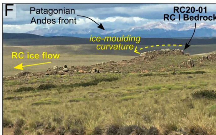
Figure 2. Field photographs of: (A-D) proglacial outwash plains and outwash surface cobbles sampled for TCN exposure dating and; (E, F) the ice-moulded bedrock surface sampled (RC20-01). Ages displayed are ^{10}\text{Be} exposure ages \pm 1\sigma analytical uncertainties. Further sample coordinates and characteristics are presented in Table 1.
