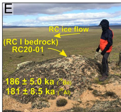
Figure 2. Field photographs of: (A-D) proglacial outwash plains and outwash surface cobbles sampled for TCN exposure dating and; (E, F) the ice-moulded bedrock surface sampled (RC20-01). Ages displayed are ^{10}\text{Be} exposure ages \pm 1\sigma analytical uncertainties. Further sample coordinates and characteristics are presented in Table 1.
