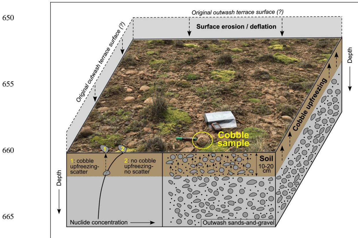
670 Figure 5. Illustration of the impact of combined outwash-plain surface deflation and near-surface turbation on exposure-age scatter for outwash surface cobbles sampled. The relationship between depth and nuclide concentration is illustrated by the decay curve (purely schematic) on the bottom left-hand corner of the diagram, which demonstrates that radionuclide production in rock minerals is reduced with depth below surface due to cosmic-ray attenuation. The attenuation effect causes cobbles that have experienced some exhumation post-deposition, due to the effect of upfreezing (dashed vertical arrows; scenario 1), to display exposure-age scatter causing landform deposition age underestimation. Cobbles that remained near the outwash surface since deposition (scenario 2) will display less/no scatter and better estimate the true minimum outwash deposition age. Cobble upfreezing is considered to mainly occur within the soil horizon (brown-coloured) due to the impact of potential permafrost formation. Soil thickness is locally estimated to reach a maximum of ~20 cm. The outwash surface photograph focuses on one of 675
