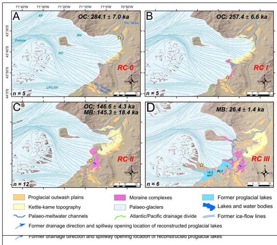
Figure 7. Palaeo-glacial reconstructions for the RC, RH, RF and Lago Palena/General Vintter (LP/LGV) valleys, for each advances/stillstands and deglacial events interpreted in this investigation (A-C). Panel D displays the ice extent associated with the RC III moraine complex, described in detail in companion publication (Leger et al. , 2021a). The latter reconstruction includes the formation of glaciolacustrine phase one (here termed PL1; Leger et al. , 2021a). Ice-sheet and mountain glacier models were digitised manually in ArcGIS. Apart from when delineated by confidently-mapped moraine limits ( e.g. the RC, RH and LP/LGV moraine sequences), the geographical location of ice margins are inferred from topography. Topographic data is from the AW3D30 DEM. “OC” and “MB” denote the type of rock samples used for TCN exposure dating of the represented event, and stand for “outwash cobbles”, and “moraine boulders”, respectively. Yellow stars indicate the approximate sample locations for TCN exposure dating of each represented event, while each panel features the number of ^{10}\text{Be} exposure ages produced ( n = x ) on the bottom left-hand corner (this excludes ^{26}\text{Al} ages). There are no previously published glacier chronologies in the RH, RF and LP/LGV valleys. Relative ice extents in those neighbouring valleys are thus inferred from our RC chronology and cross-valley comparisons of moraine set numbers, preservation and morphostratigraphy. Hence, these inferences yield some uncertainties. Proglacial lake volume estimates were computed from DEM data (AW3D30).
