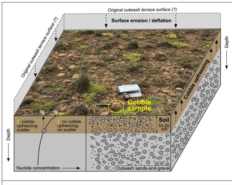
670 Figure 5. Illustration of the impact of combined outwash-plain surface deflation and near-surface turbation on exposure-age scatter for outwash surface cobbles sampled. The relationship between depth and nuclide concentration is illustrated by the decay curve (purely schematic) on the bottom left-hand corner of the diagram, which demonstrates that radionuclide production in rock minerals is reduced with depth below surface due to cosmic-ray attenuation. The attenuation effect causes cobbles that have experienced some exhumation post-deposition, due to the effect of upfreezing (dashed vertical arrows; scenario 1), to display exposure-age scatter causing landform deposition age underestimation. Cobbles that remained near the outwash surface since deposition (scenario 2) will display less/no scatter and better estimate the true minimum outwash deposition age. Cobble upfreezing is considered to mainly 675
