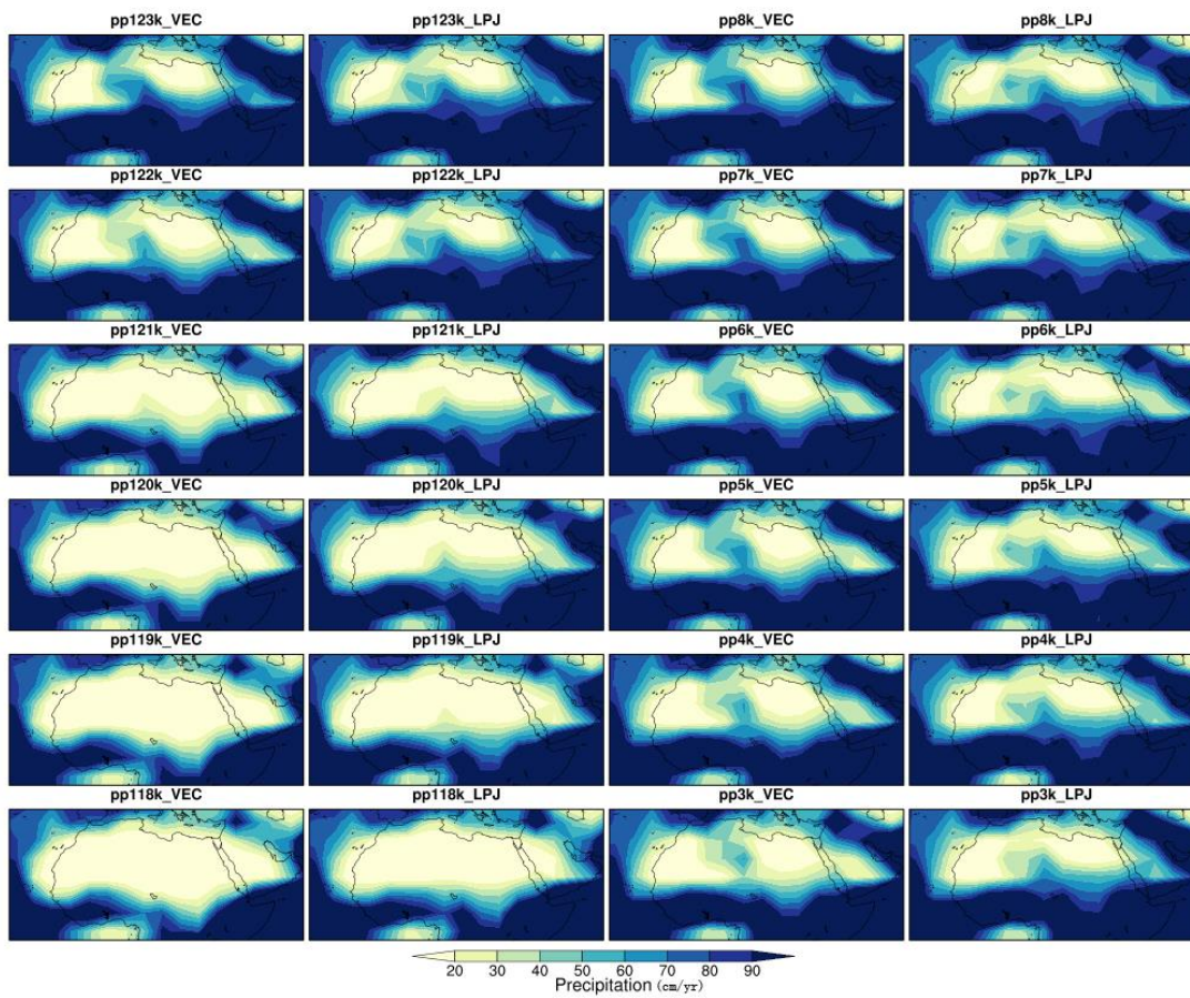
Figure S4. Precipitation during the LIG (left two columns) and Holocene (right two columns) from VECODE (left) and LPJ-GUESS (right).
