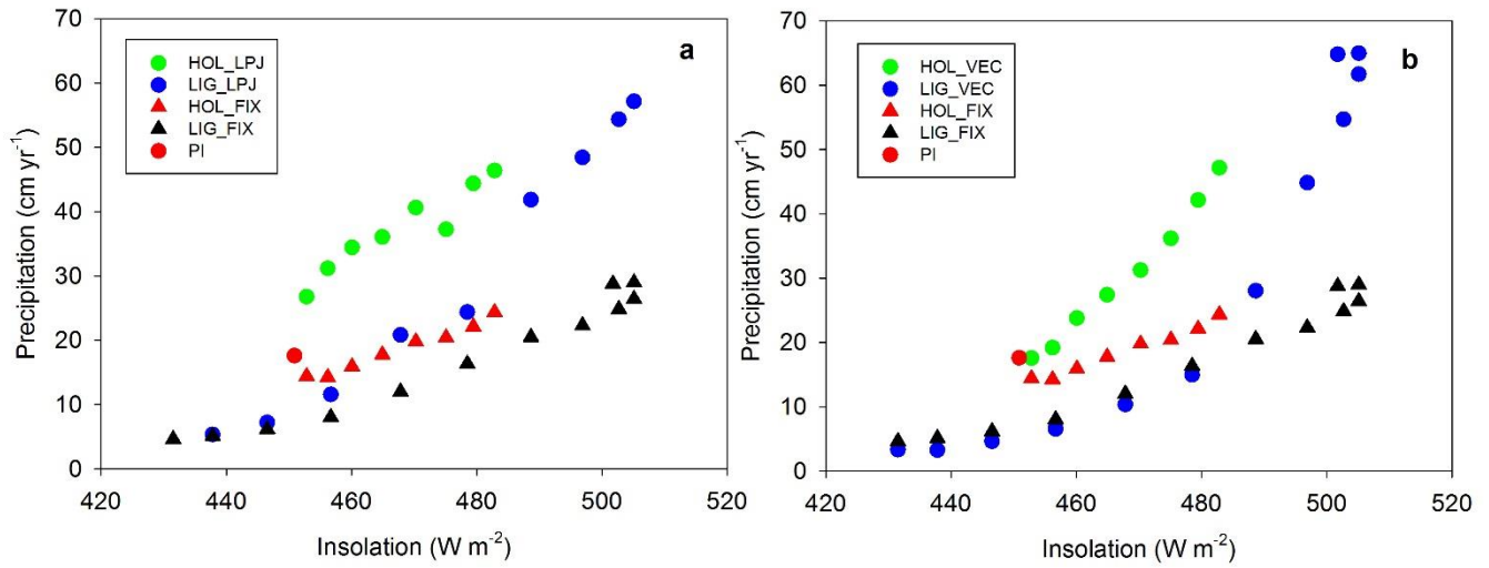
755 Figure 6: The relationship between insolation at 20°N and precipitation with dynamic vegetation from LPJ-GUESS (a) and VECODE (b) during two interglacials, with blue dots representing the LIG and green dots representing the Holocene. For reference, the results of HOL_FIX, LIG_FIX and PI are also included.
