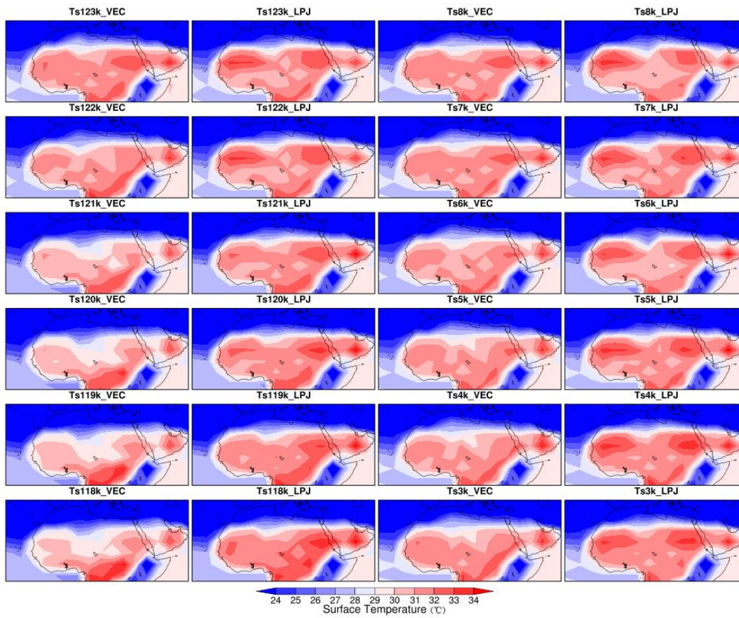
770 Figure S2. Surface temperature during the LIG (left two columns) and Holocene (right two columns) from VECODE (left) and LPJ-GUESS (right).
