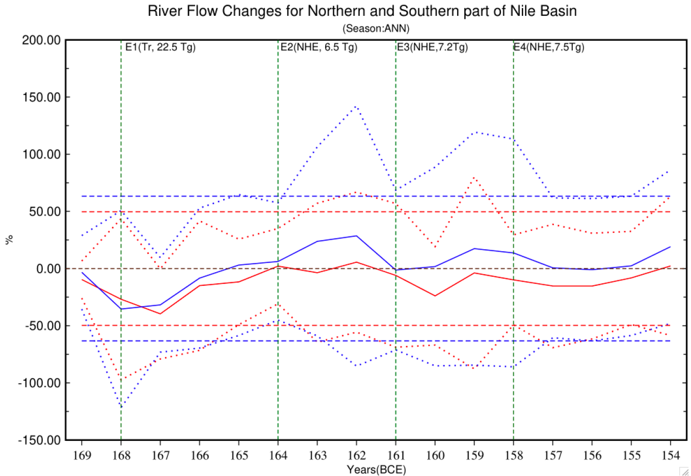
745 Figure 13. Annual Nile River flow changes averaged over the northern (red) and southern (blue) parts of the basin (divided at 10° N) for the entire simulation period. The solid lines represent the ensemble mean for each part of the basin; the dotted lines are \pm 1.95\sigma , where \sigma is derived from across all the ensembles, and the horizontal dashed lines parallel to x-axis are the \pm 1.95\sigma_{ctrl} where \sigma_{ctrl} is the standard deviation across the 100-year control run. Red and blue lines correspond to the northern and southern parts of the Nile basin, respectively.
