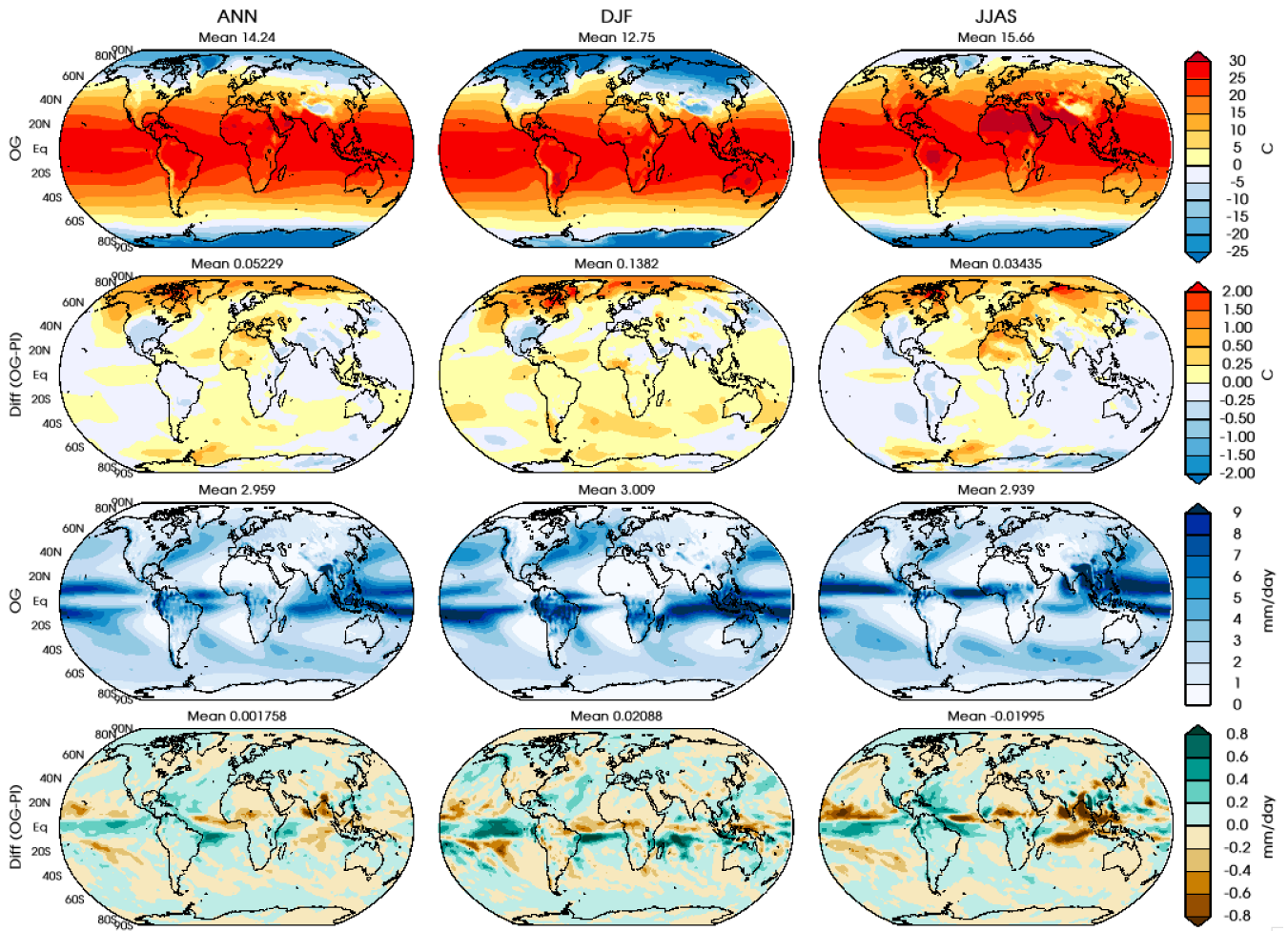
320 Figure 1. Seasonal mean (Annual, DJF & JJAS) surface air temperature (top row) for the 2.5ka period equilibrium run, differences from the preindustrial period (2.5ka-preindustrial) for all three seasons (2 nd row from top) and seasonal (Annual, DJF & JJAS) mean precipitation (3 rd row from top) and the difference (bottom row) from the preindustrial period (2.5ka-preindustrial). The equilibrium run for the 2.5ka period includes the orbital and GHG concentration changes for the 2.5ka period (referred to as OG), the preindustrial period (as PI), and their difference (OG-PI) as simulated by GISS ModelE2.1.
