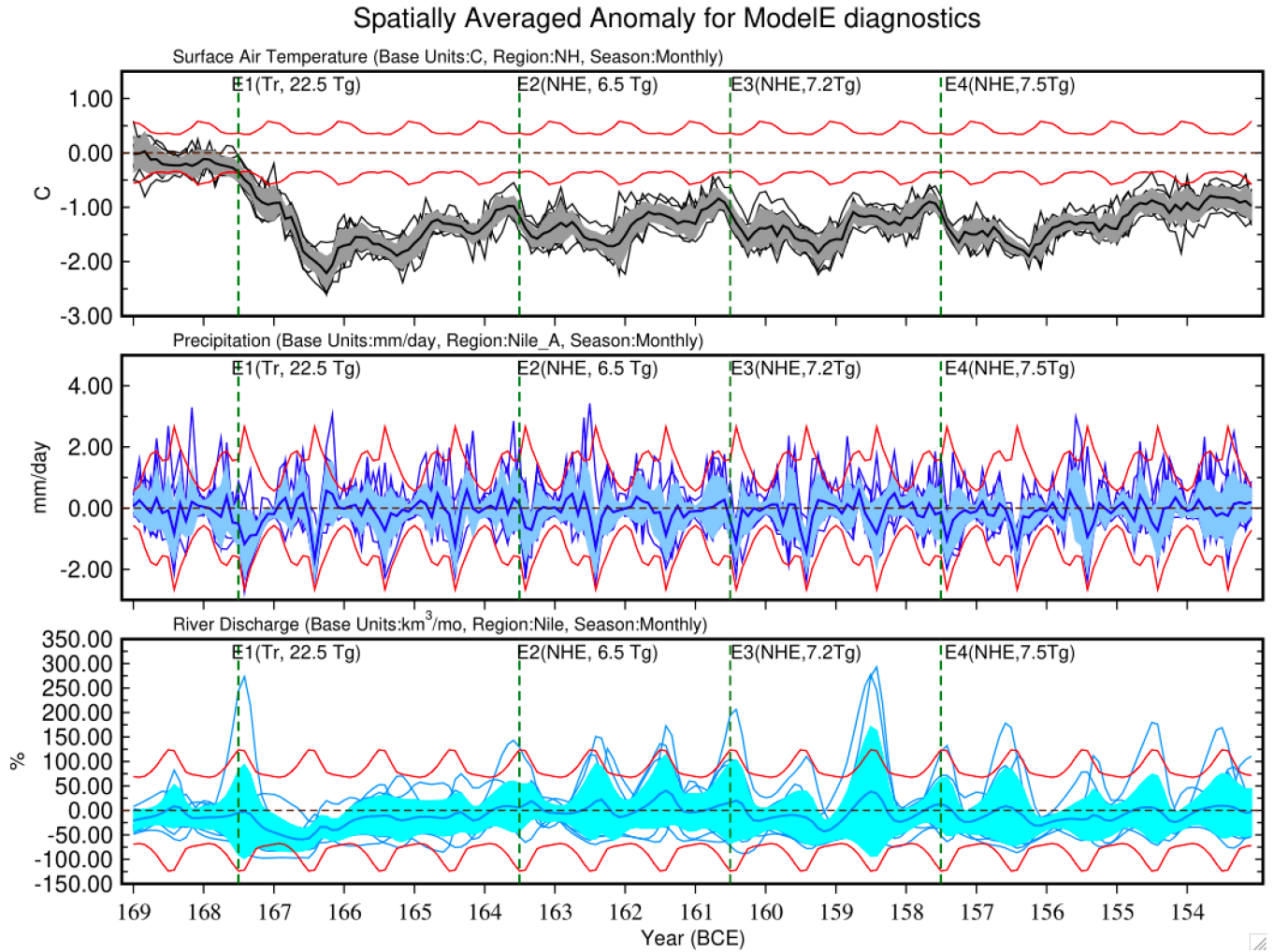
Figure 12: Monthly time series of individual ensemble and mean of surface temperature response ( ^{\circ}\text{C} ) averaged over northern hemisphere (NH) (top panel), rainfall change (mm/day) for the model's spatial box representing the Nile River watershed (Latitude: (5N, 18N), Longitude: (30E, 42E)) (middle panel)
