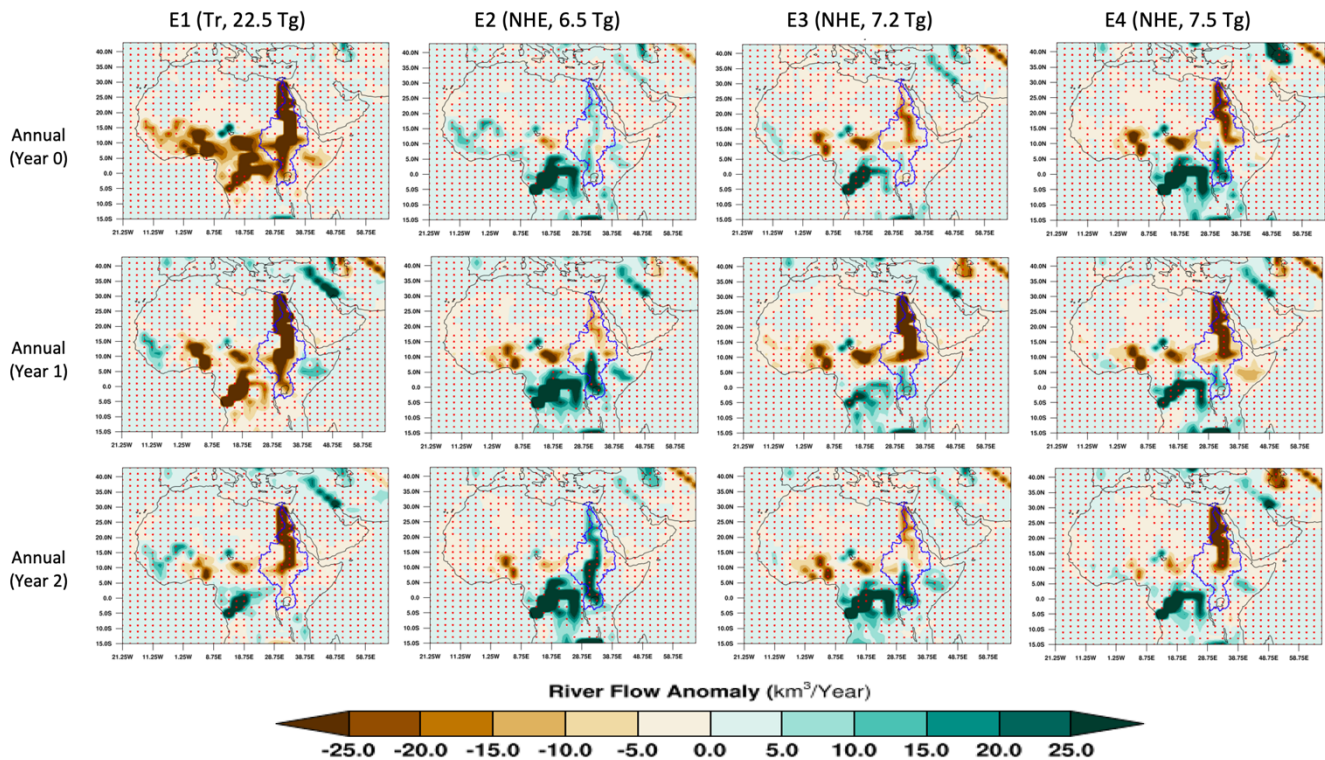
680 Figure 11. Annual river flow anomaly ( \text{km}^3/\text{year} ) relative to the control climatology for 3 consecutive years after each eruption (columns) over North Africa. Other details as per Fig. 10.
