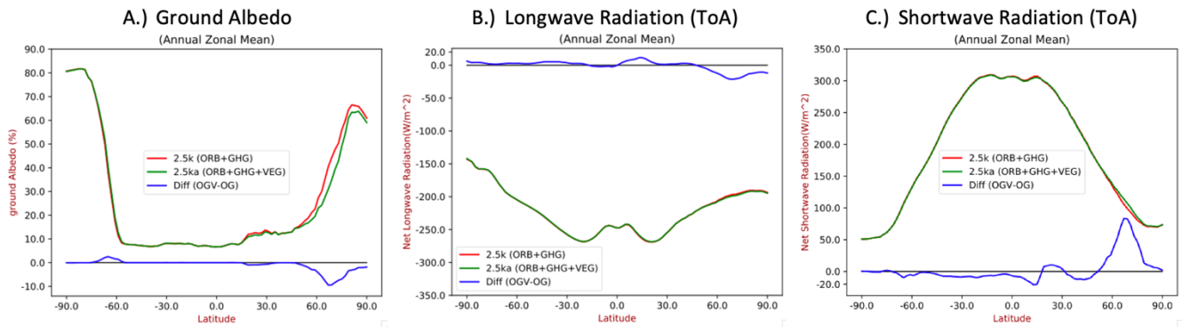
Figure 3. Annual zonal mean of ground albedo (A), longwave & shortwave radiation at the top of the atmosphere (ToA; B and C) for 2.5ka climates with ORB+GHG and ORB+GHG+VEG (red and green lines), respectively. The blue line shows the difference between them. The blue line in panel B & C is exaggerated 10-fold (x10) to show the difference more clearly on the same vertical axis.
