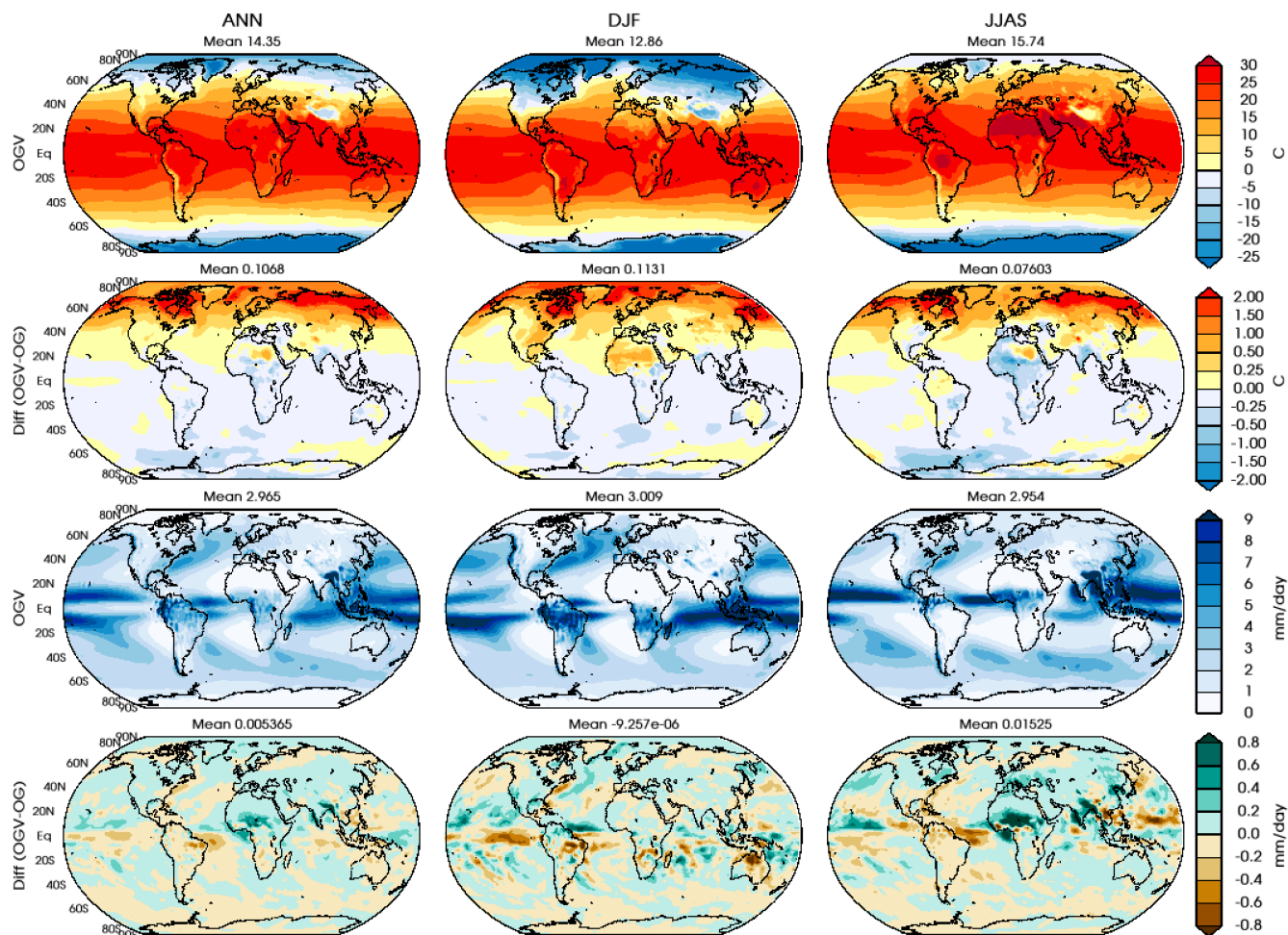
Figure 2. Mean surface air temperature for Annual, DJF and JJAS seasons (top row) and seasonal mean precipitation (3 rd row from top) for the equilibrium runs with the PMIP4 vegetation for the 2.5ka period and surface temperature difference (2 nd row from top) plus the seasonal precipitation differences (bottom row) for the 2.5ka period as simulated by GISS ModelE2.1. We have used a short initial notation for our 335 forcings to denote the difference (ORB+GHG+VEG = OGV and ORB+GHG= OG)
