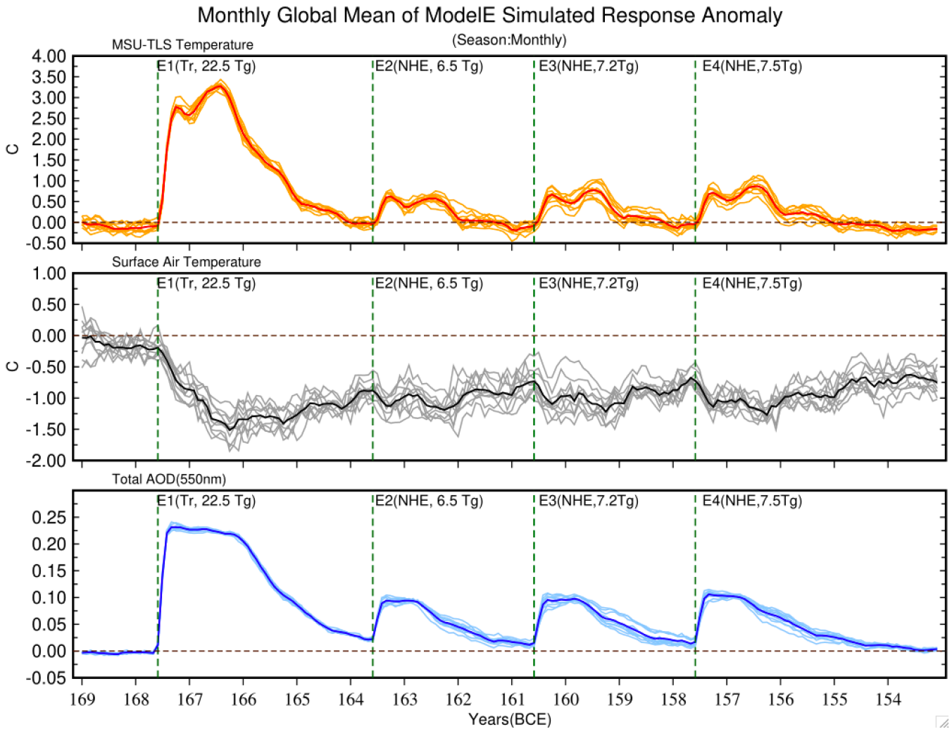
Figure 5. Globally averaged changes in MSU TLS (top panel), surface air temperature (middle panel) and total atmospheric column AOD at 550 nm for each month for the entire simulation period. The light-colored solid lines represent individual ensemble members, and the solid dark colors show the ensemble means. The green vertical dashed lines show when the modelled eruptions happened.
