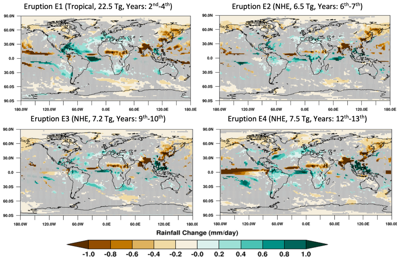
555 Figure 9. Mean change (mm/day) in northern hemisphere monsoon season (JJAS) rainfall averaged for three consecutive years after eruption E1 (including the eruption year) and two years each after E2, E3 and E4 (including the eruption years) (left to right and top to bottom). The caption over each panel shows the eruption characteristics. A gray color is painted over the grid boxes for which rainfall change is not significant at the 95% confidence level. Years indicated in parentheses follow the order of the eruptions 560 in our simulation period, i.e., E1 occurs in the 2 nd simulation year, and E2-E4 occur in the 6 th , 9 th and 12 th years, respectively.
