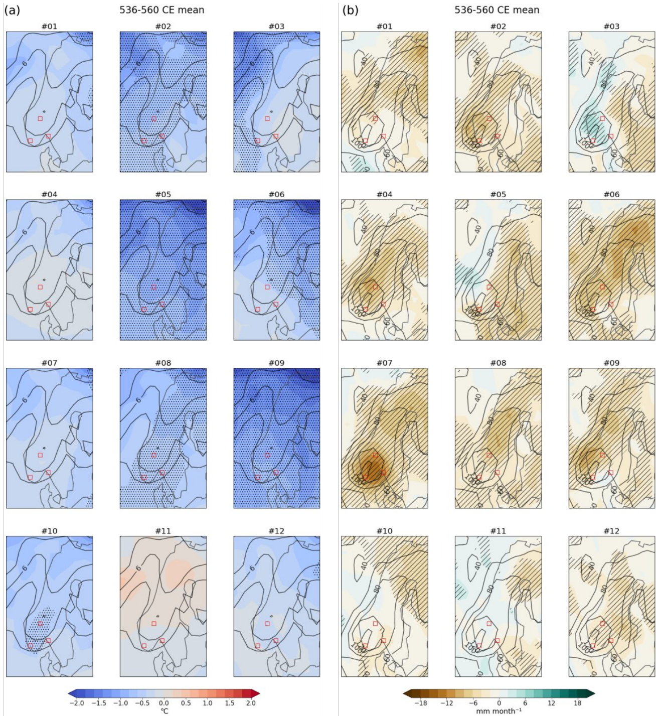
Figure 5. a) temperature and b) precipitation anomaly maps for the mean growing season (536-560 CE) for the individual ensemble members. Anomalies are calculated with respect to 0-1850 CE. 0-1850 CE climatology in contours. The red squares indicate the locations of the local sites used for the GDD modelling. The 1 \sigma (2 \sigma ) significant areas are hashed (stippled) for precipitation (2m air temperature).
