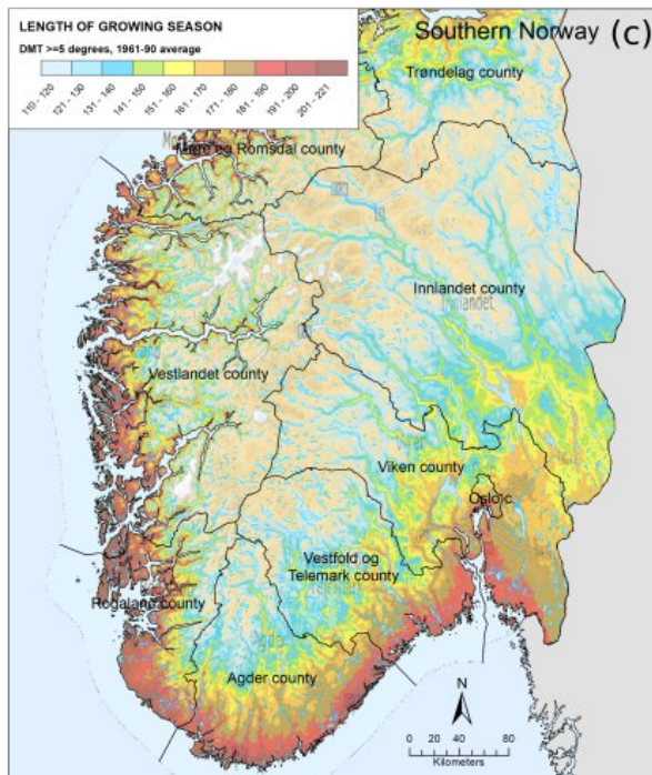
290 Figure 1. a) The three areas and sites for the case study. Red outline indicates the regions, bold names are the areas and the stars indicate the locations and names of the bogs analysed for pollen. DEM map from ESRI 2020. b) The summer precipitation and c) average length of the growing season (days) for Southern Norway during 1961-1990, for days with a daily mean temperature (DMT) at or above 5 °C (adapted from Hanssen-Bauer et al., 2017).
