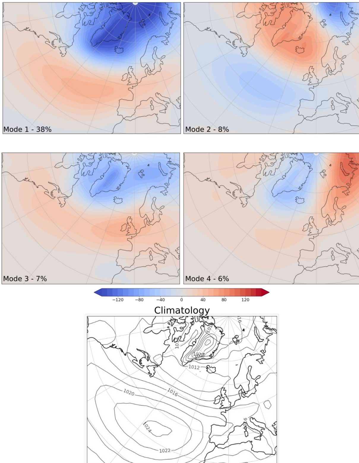
1300 Figure A4. The SLP EOF first four modes of atmospheric circulation patterns for the past2k #1 for a) DJF (see also van Dijk et al., 2022) and b) the mean growing season (AMJJAS) during 0-1850 CE. The SLP climatology for 0-1850 CE is given in the lowest panel; contours are given in 2 hPa intervals.
