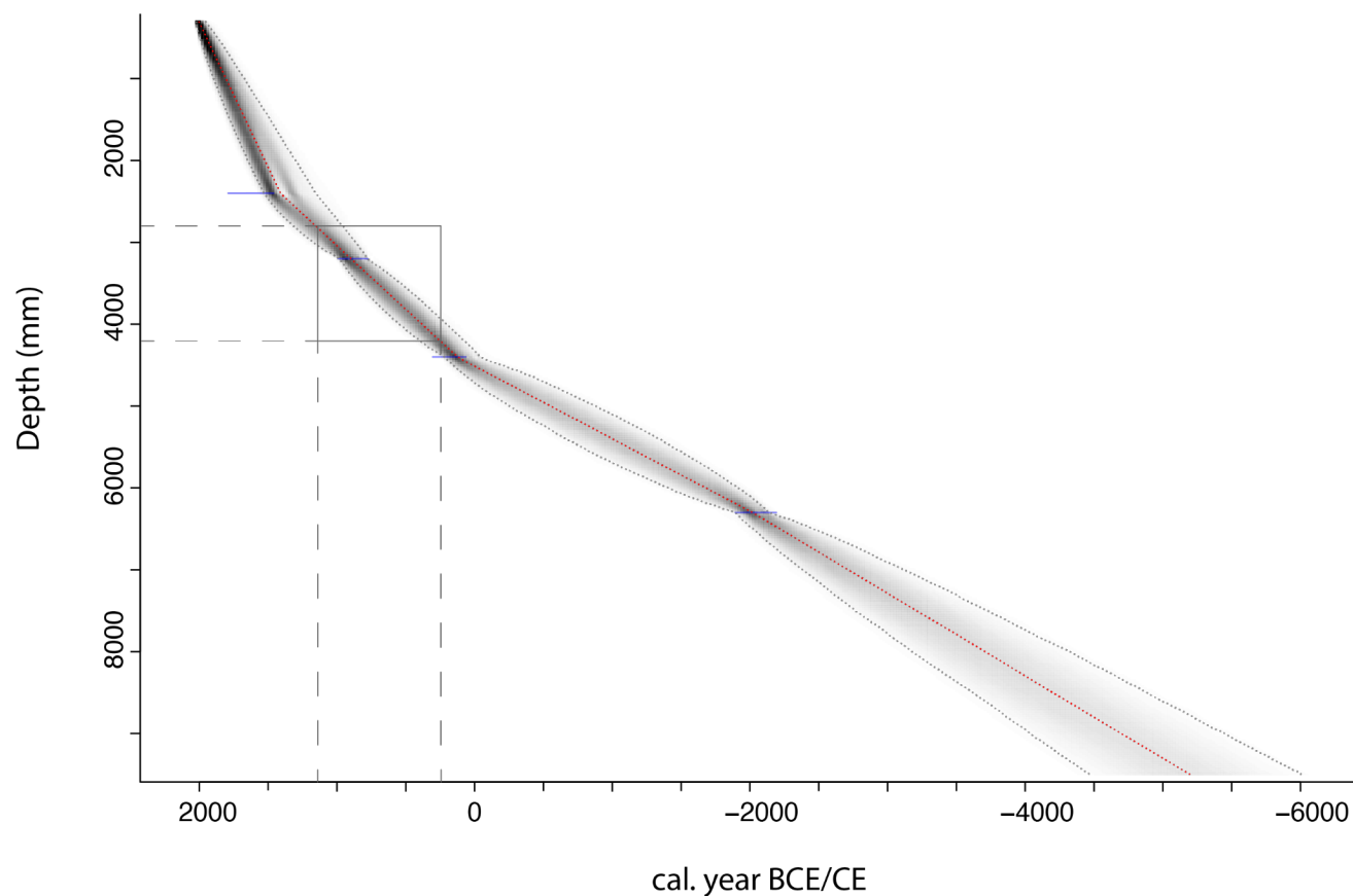
Figure A8: Age-depth model Åsheimmyr peat sequence represented with the RBacon package. The section in the rectangle indicates the study period 250-1150 CE.
