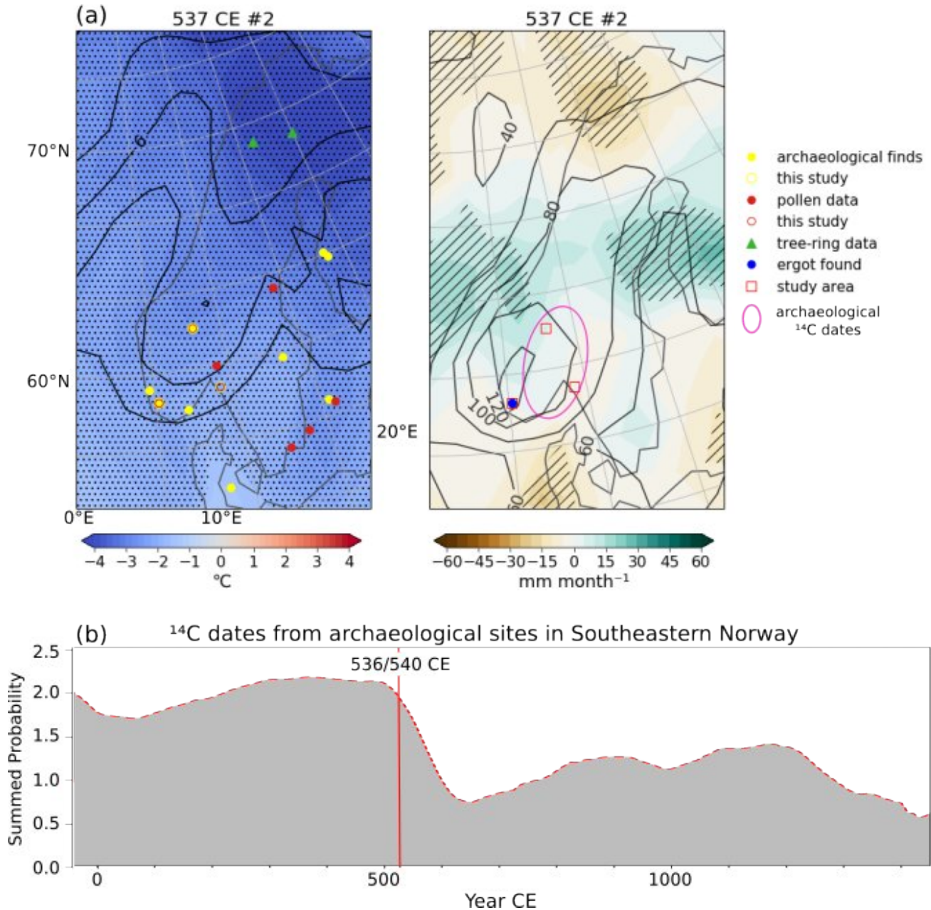
Figure 9. Synthesis figure. a) temperature and precipitation anomaly maps of Scandinavia from one realisation of the MPI-ESM model (ensemble member #2), with markers for archaeological, historical, and pollen proxy data supporting this model simulation. Pollen data showing reduction in agriculture in the mid-500s, archaeological finds indicating abandonment, and tree-ring reconstructions with a 3.5 °C cooling in Northern Scandinavia 1-2 years after the 536 CE eruption. The data used for this figure are listed in Table A4. b) Summed probability distribution of 4012 14 C dates (Loftsgarden and Solheim, in press) from archaeological sites in Southeastern Norway.
