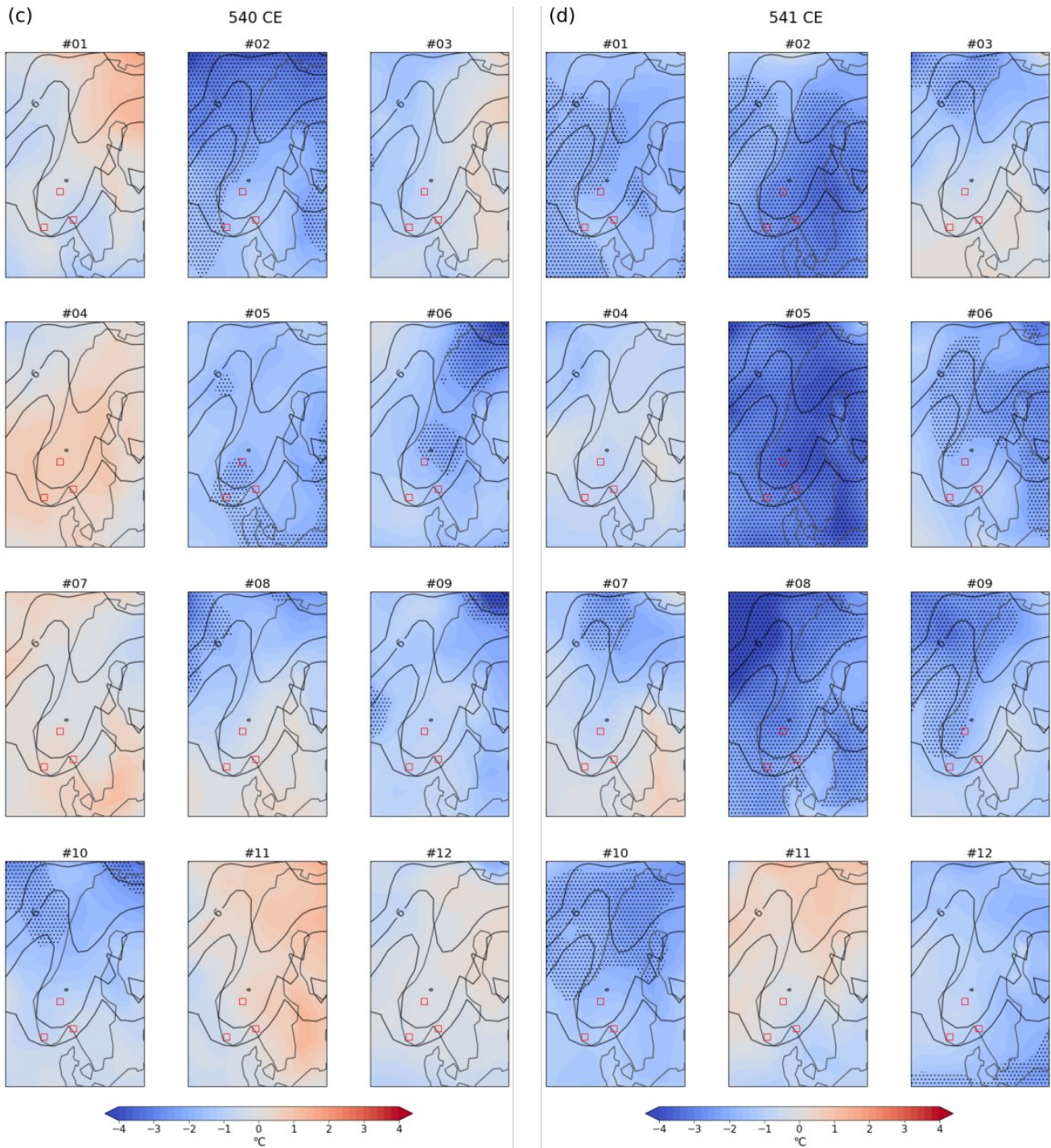
Figure A1. 2m air temperature anomaly for the individual ensemble members of a) 536 CE, b) 537 CE, c) 540 CE, and d) 541 CE. Anomalies are calculated with respect to 0-1850 CE. 0-1850 CE climatology in contours (1 °C intervals). The red squares indicate the areas used for the growing degree day calculations. The 2 \sigma significant level is stippled.
