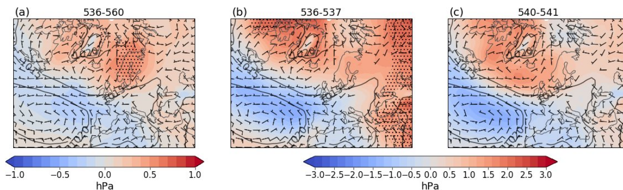
Figure 4. Maps of the North Atlantic ensemble mean sea level pressure anomalies and absolute wind for the mean growing season (AMJJAS) for a) 536-560 CE, b) 536-537 CE, and c) 540-541 CE.
