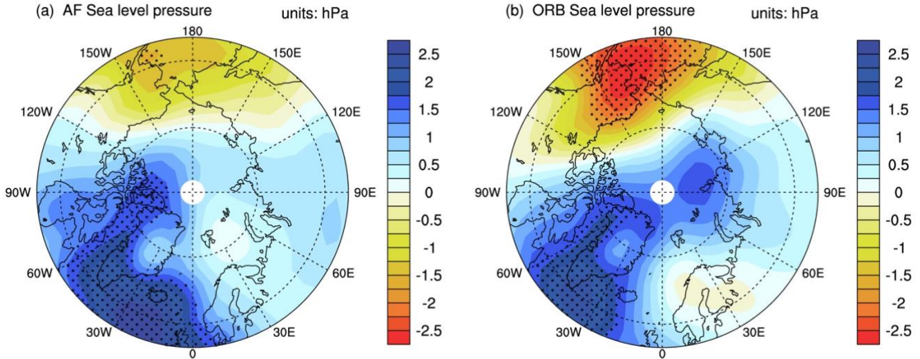
Figure 5: (a) The DJF sea level pressure changes between two period (0-2 ka BP and 5-8 ka BP) in NNU-Holocene All forcing simulation; (b) Same as (a) but for ORB forcing simulation; Areas that are dotted are significant at the 90% confidence level.
