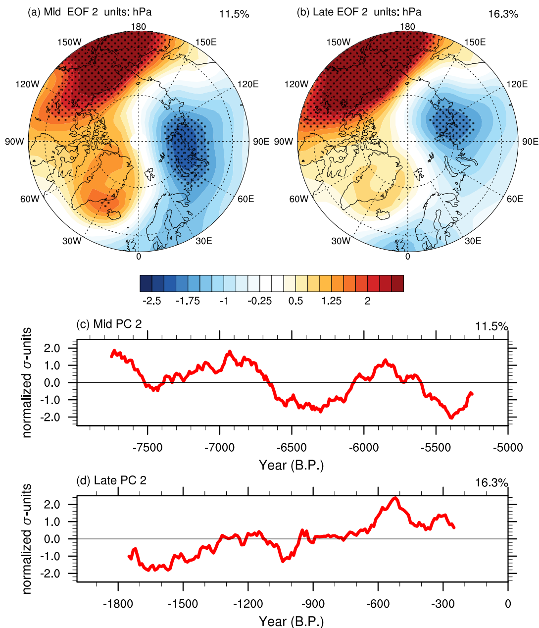
285 Figure 6: The second EOF (EOF2) pattern of the Sea level pressure in NNU-Holocene All forcing simulations during 5-8 ka BP (a) and 0-2 ka BP (b); The second Principal Component time series of the EOF during 5-8 ka BP (c) and 0-2 ka BP (d) after 50yr smoothed; Areas that are dotted are significant at the 90% confidence level.
