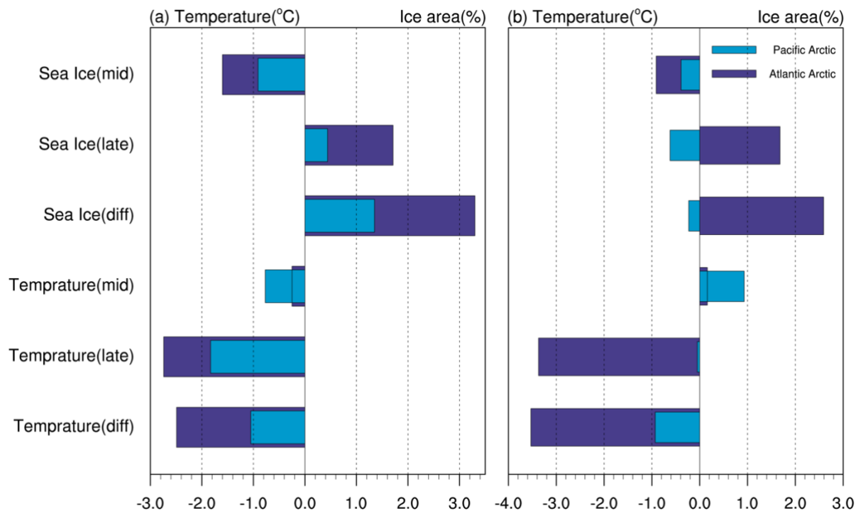
320 Figure 8: 1) Average change in the regression of Sea ice on the PC2 of the SLP in early-mid Holocene; 2) same as 1) in late Holocene; 3) Differences in the regressions of Sea ice on PC2 of SLP between two period; 4) The regression of temperature average change in early-mid Holocene; 5) same as 4) in late Holocene; 6) Differences in the regressions of temperature on PC2 of SLP between two period (a: AF simulation, b: ORB simulation); the difference in sea ice and temperature between two period are statistically significant at the 90% confidence level.
