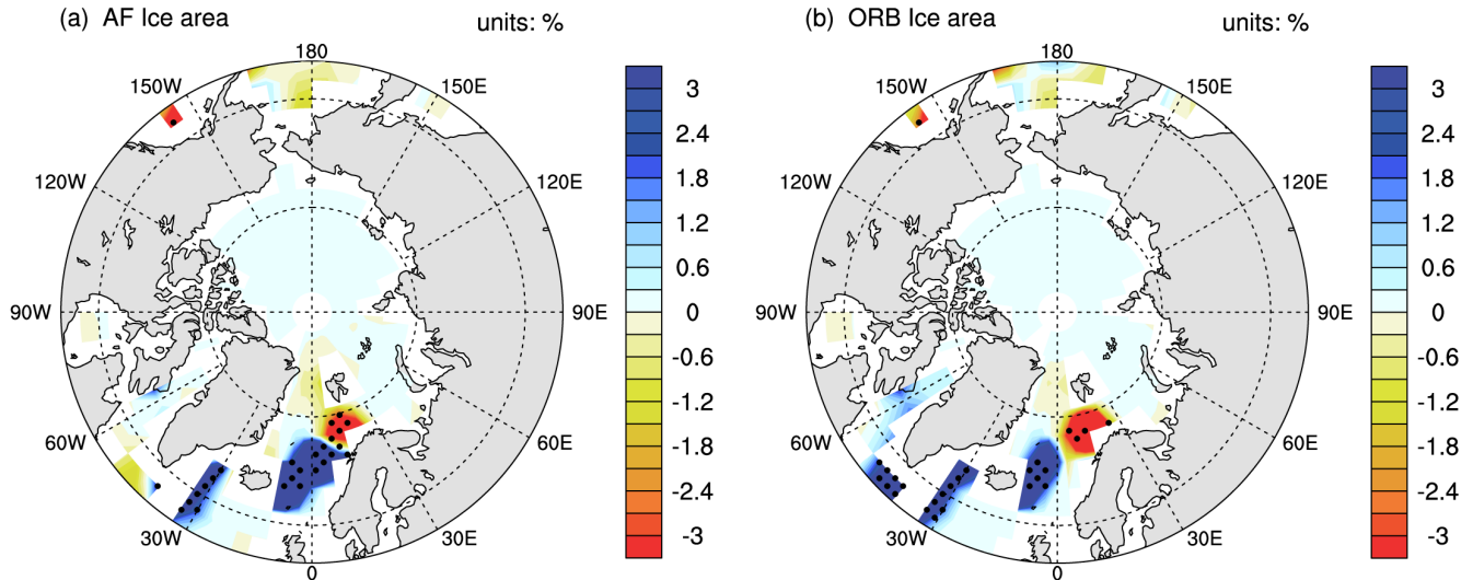
245 Figure 4: (a) The March sea ice area (aice) changes between two period (0-2 ka BP and 5-8 ka BP) in NNU-Holocene All forcing simulation (regional average on Pacific Arctic:0.02% and Atlantic Arctic:0.29%); (b) Same as (a) but for ORB forcing simulation (regional average on Pacific Arctic:0.04%, Atlantic Arctic:0.29%); Areas that are dotted are significant at the 90% confidence level. The difference of the means sea ice area changes in the two regions is significant at the 90% confidence level in both AF and ORB.
