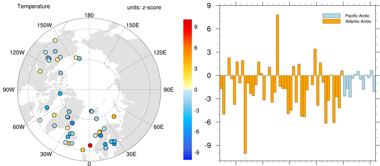
Figure 1: (a) The annual temperature changes between two period (0-2 ka BP minus 5-8 ka BP) in Reconstructions (Temperature 12k); (b) Histogram of temperature change for each proxy site
