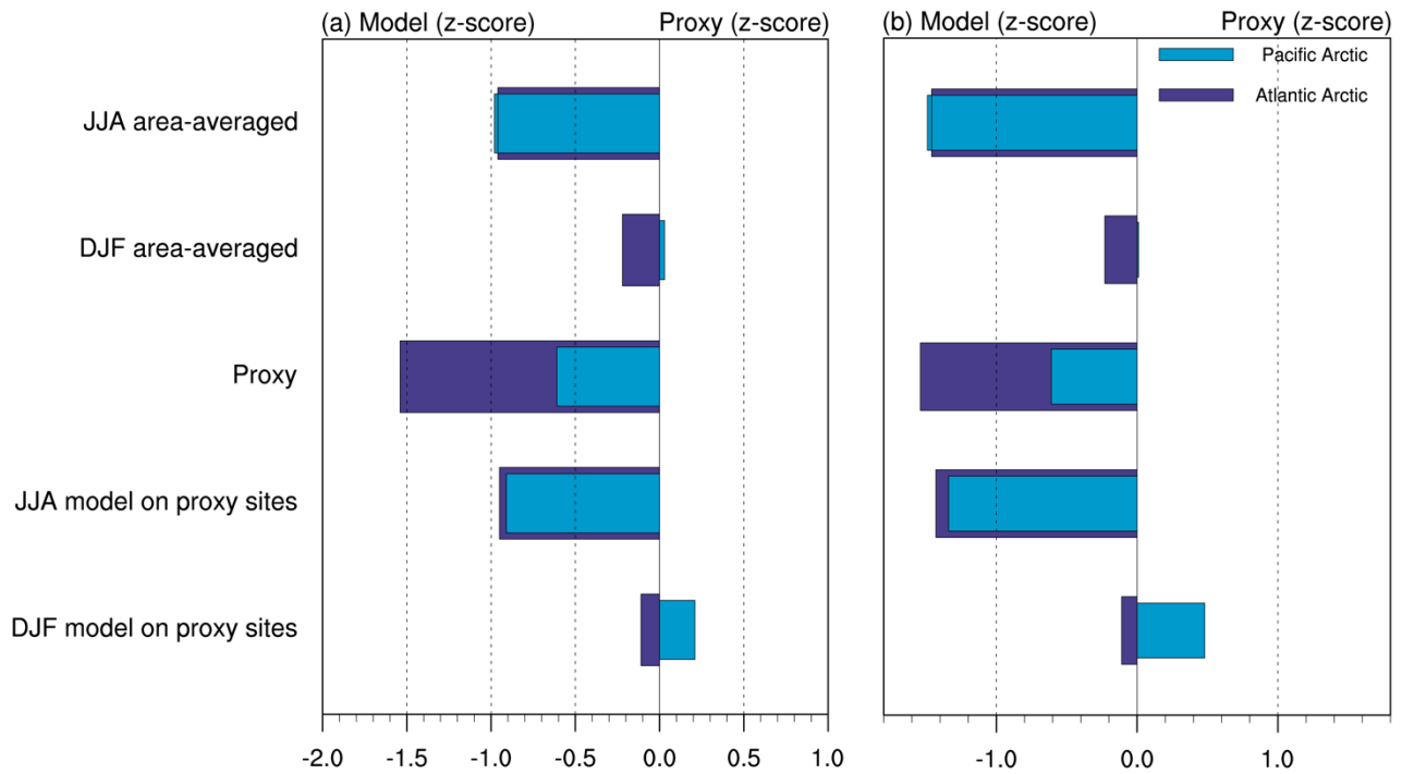
220 Figure 3: 1) Model area average temperature change in JJA; 2) Model area average temperature change in DJF; 3) Annual temperature change in Proxy; 4) Model JJA average temperature change on proxy sites; 5) Model DJF average temperature change on proxy sites (a: AF simulation, b: ORB simulation);
