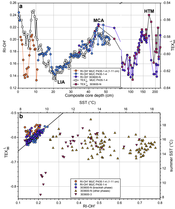
Figure 5: The relationship between the RI-OH' and \text{TEX}_{86}^L indices for the Gotland Basin for the studied sedimentary record. (a) RI-OH' (filled circles) and \text{TEX}_{86}^L (filled squares) plotted versus composite core depth for the section covering the Littorina Sea phase. The data of the multicore P435-1-4 are plotted in orange, light blue and white symbols, those from piston core 303600-N are plotted with purple circles and pink squares. The plot shows the overall good correspondence of variations in the RI-OH' index and \text{TEX}_{86}^L records, suggesting that the RI-OH' index in the Littorina Sea phase records SST changes. Note that in the upper part of the section (1-11 cm; orange circles for RI-OH') the overall correlation is distorted; the values of the RI-OH' index seem ca. 0.04 too low. The scale of the composite core depth axis is broken at ca. 60 cm and the scale of the second part of the depth scale is more compressed. For core 303600-N only data points are shown for which both RI-OH' and \text{TEX}_{86}^L values were obtained. Key: MCA = the medieval climate anomaly, LIA = little ice age, HTM = Holocene thermal maximum. (b) RI-OH' index values plotted vs. \text{TEX}_{86}^L values for the complete Gotland basin record. In the left upper corner of the plot the correlation ( R^2 = 0.76 ) between the values of the RI-OH' index and \text{TEX}_{86}^L for the P435-1-4 MUC core (light blue circles) except for the 1-11 cm section (orange circles) is shown. The sediment horizons from multicore 303600-N are plotted with purple circles (Littorina Sea phase) and gold upper triangles. Those from the Littorina Sea phase plot in line with the linear correlation line. Those from the 303600-3 core are plotted with pink lower triangles. The sediments from the other phases (especially in the Ancylus Lake phase, see Fig. 2) show much higher values for the RI-OH' index, translating into much higher annual mean SSTs (upper scale) using the Baltic Sea calibration (equation 9), whereas those of the \text{TEX}_{86}^L are similar or slightly lower and show much less variation in July-November SSTs as estimated with the Baltic Sea calibration (equation 8; Kabel et al., 2012). Note that the Yoldia Sea sediments from around ca. 410 cm plot together with those from the Littorina Sea phase. The other Yoldia Sea sediments with relatively low RI-OH' index values (470-530 cm; Fig. 2f) show much lower \text{TEX}_{86}^L values than all other sediments.
