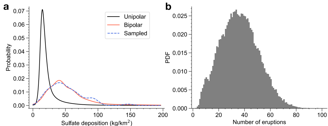
Figure 4. a Kernel density estimate of the Antarctic sulfate deposition in the unipolar and bipolar LIN22 data sets, as well as a large number of samples from the resampling method described in Appendix B (dashed blue line), where subsamples from the unipolar data set are drawn such that they follow the distribution of the bipolar population. b Histogram of the number of eruptions contained in each unipolar subsample after 50,000 iterations of the resampling method.
