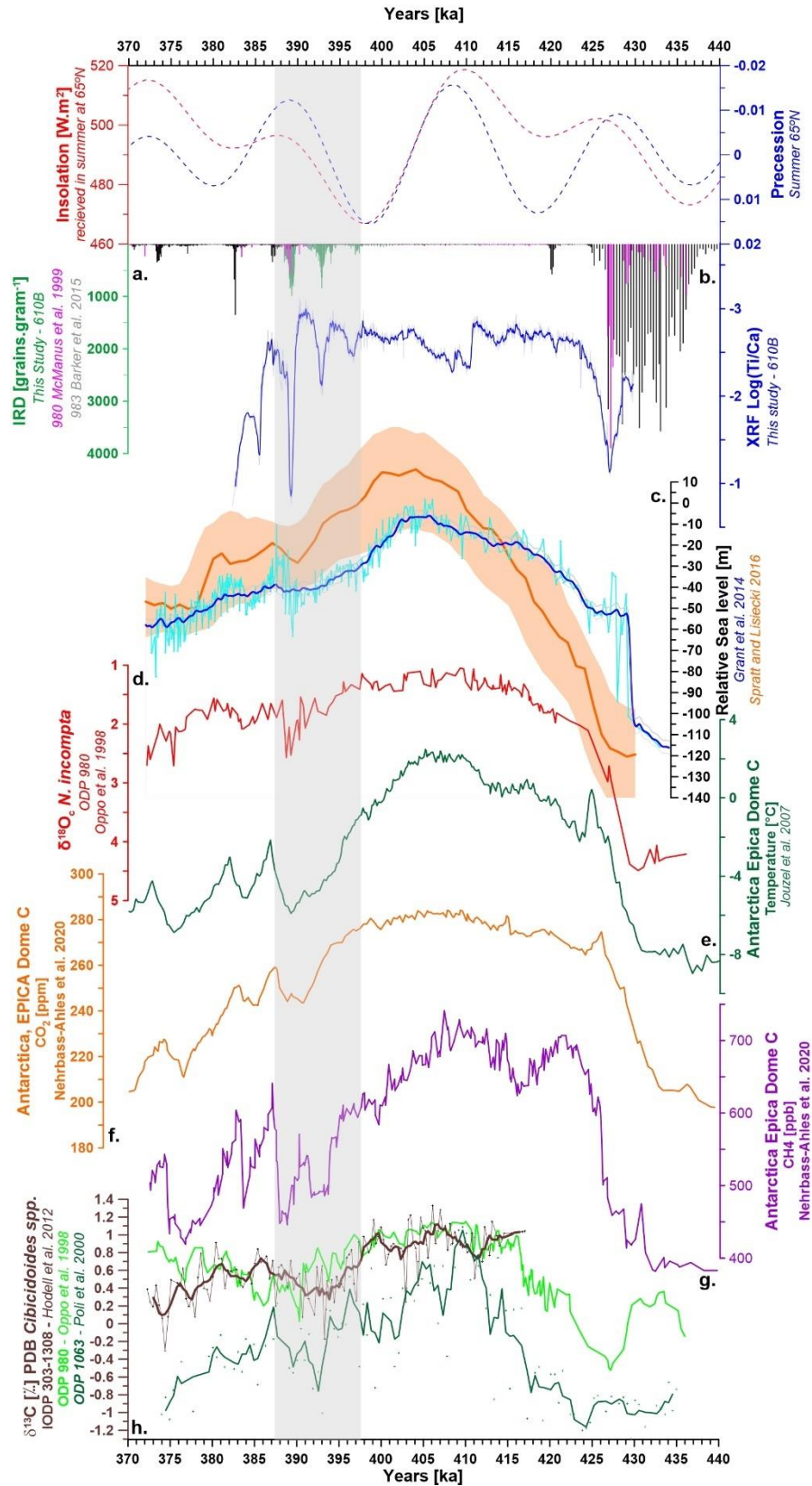
Figure 5 | Age model development for DSDP 610B (370-430 ka ago). a. IRD per gram records from DSDP 610B (green), ODP site 980 (pink), and ODP 983 (black); b. log (Ti/Ca) record for DSDP 610B (blue); c. global relative sea-level curve (blue and orange); d. ODP 980 \delta^{18}O_c N. incompta (red); e. EDC Antarctic ice core temperature (green); f. Carbon Dioxide (CO 2 ;
