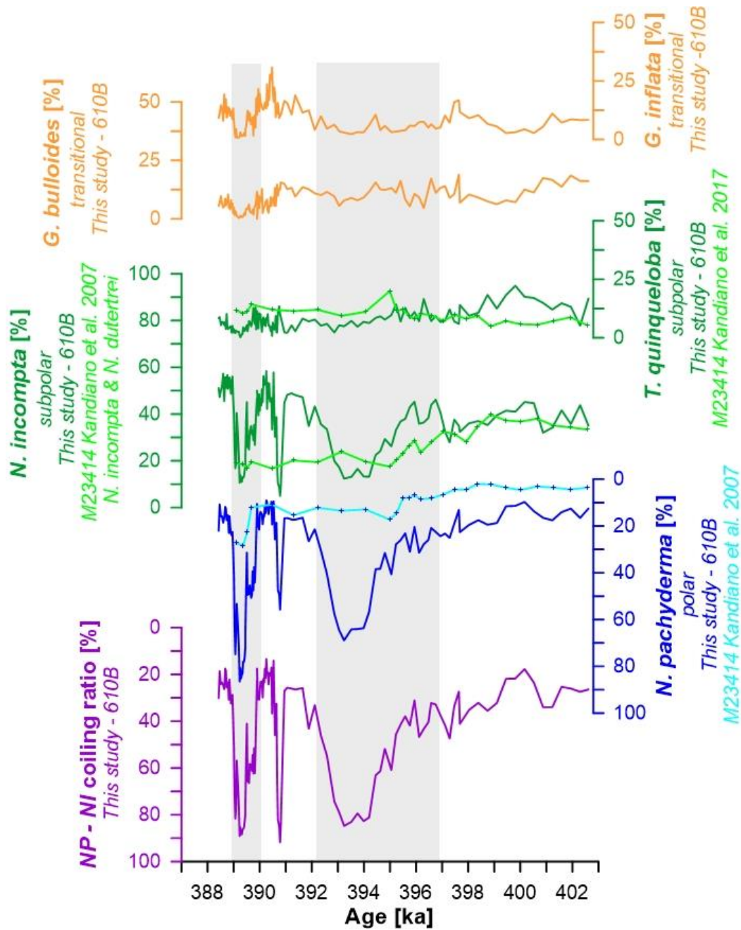
Figure 2 | The evolution of planktic foraminifera over the MIS 11 glacial inception. From top-to-bottom, the relative abundances of G. inflata (transitional, orange), G. bulloides (transitional, orange), T. quinqueloba (subpolar, green), N. incompta (subpolar, green), N. pachyderma (note reversed axis, polar, blue), and coiling ratio (%) of N. pachyderma to N. incompta (note reversed axis, purple). Also shown are assemblage counts for T. quinqueloba , N. incompta , and N. pachyderma from nearby site M23414 (Kandiano et al. 2007).
