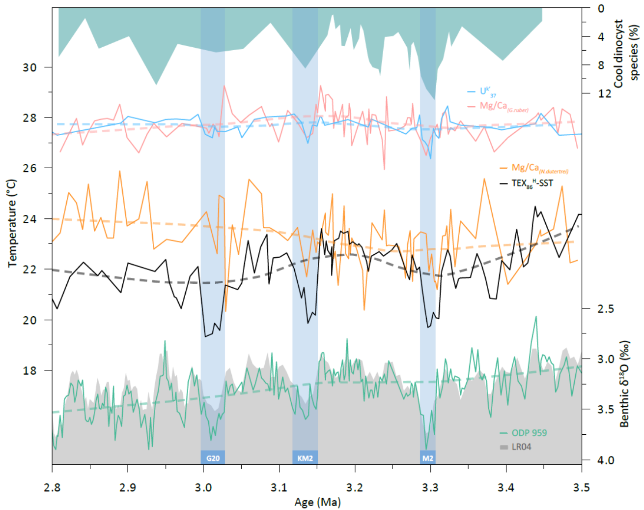
595 Figure 5. Compilation of late Pliocene multi-proxy temperature data and benthic \delta^{18}\text{O} at Site 959. \text{Mg}/\text{Ca}_{(G.ruber)} (pink) and \text{Mg}/\text{Ca}_{(N.dutertrei)} (yellow) from van der Weijst et al. (2022), benthic \delta^{18}\text{O} from van der Weijst et al. (2020) and LR04 \delta^{18}\text{O} stack (Lisiecki and Raymo, 2005) for reference. Dashed lines in are LOESS smoothed trends and vertical bands indicate the M2, KM2 and G20 glacial stages.
