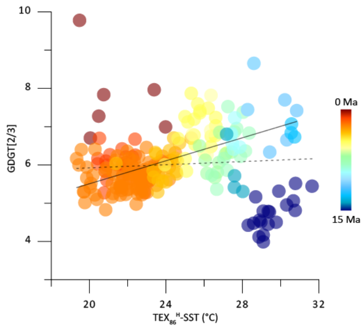
Figure 7. Cross-plot of TEX 86 H -SST and GDGT[2/3]. The oldest (>13.6 Ma; dark blue) and youngest (<1.7 Ma; dark red) samples largely stand out from the majority of the data. Linear regression lines determined from full dataset (stippled line) and samples dated between 13.6 and 1.7 Ma (solid line; 88% samples, R 2 =0.37, p<0.001).
