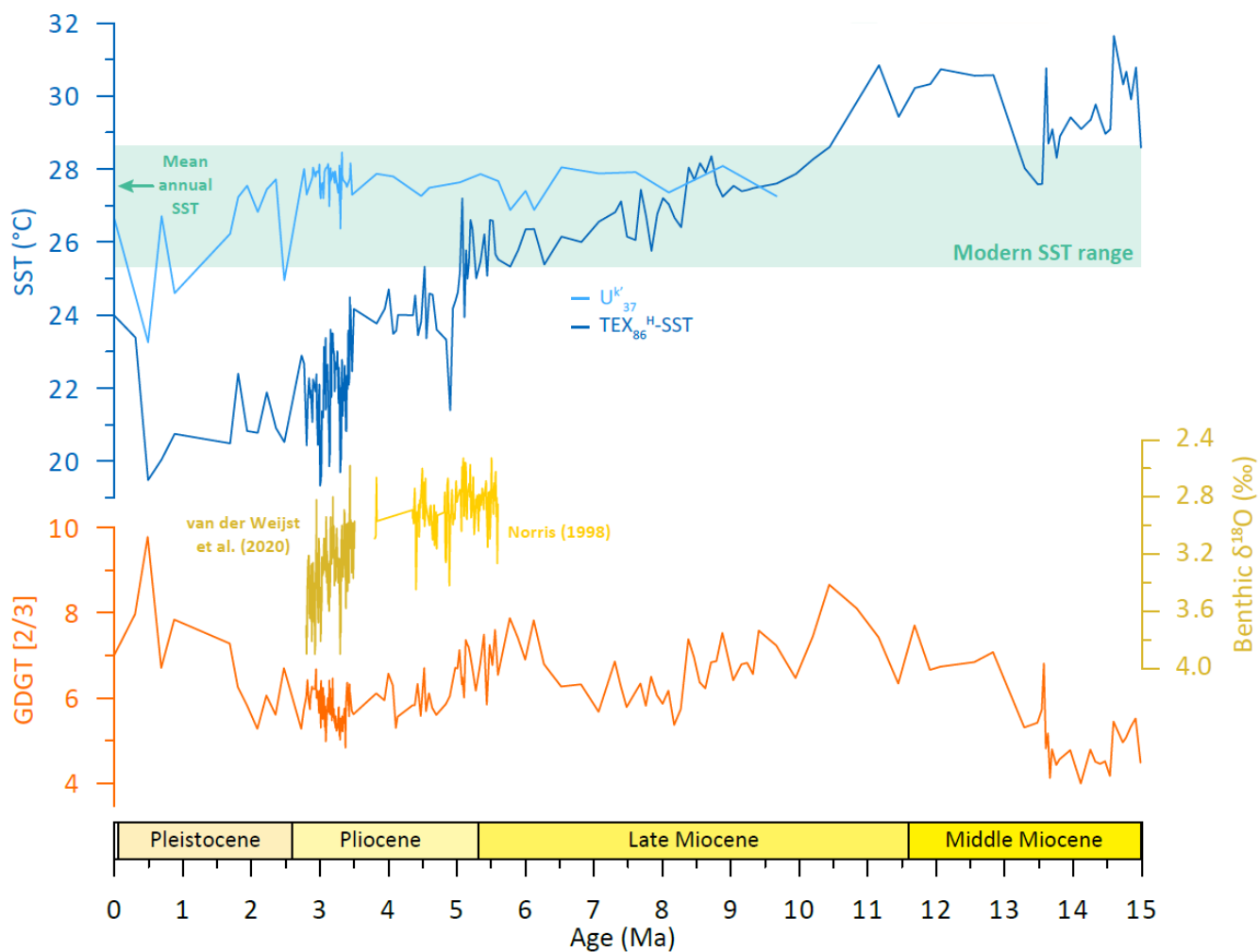
Figure 3. New TEX_{86}^H -SST (Kim et al., 2010 calibration), U^{k}_{37} -SST (Müller et al., 1998 calibration) and GDGT[2/3] records at Site 959, compared to benthic \delta^{18}\text{O} records from Norris (1998a) and van der Weijst et al. (2020). Shaded interval and arrow indicate annual SST range and mean annual SST in the Gulf of Guinea, respectively (Locarnini et al., 2013).
