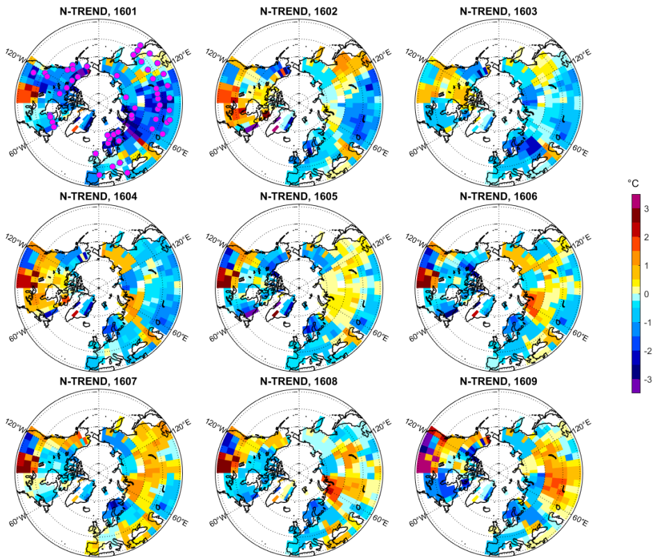
330 Figure 56. N-TREND temperature anomaly in each year of the period 1601-1609 with respect to the average over the period 1550- 1590. The purple dots in top-left plot indicate sites of tree-ring width and maximum latewood density used for the spatial reconstruction. The size of reconstructed grid cells is 5x5° lat/long. The instrumental data used as target field for the reconstruction are May to August monthly temperature anomalies w.r.t. the 1961-1990 period extracted from the HadCRUruT4 (Cowtan and Way, 2014). The spatial reconstruction was developed using a point-by-point regression (Cook et al., 1999) which accounts for the spatial 335 distribution and relationship of the proxy predictor network to the target field.
