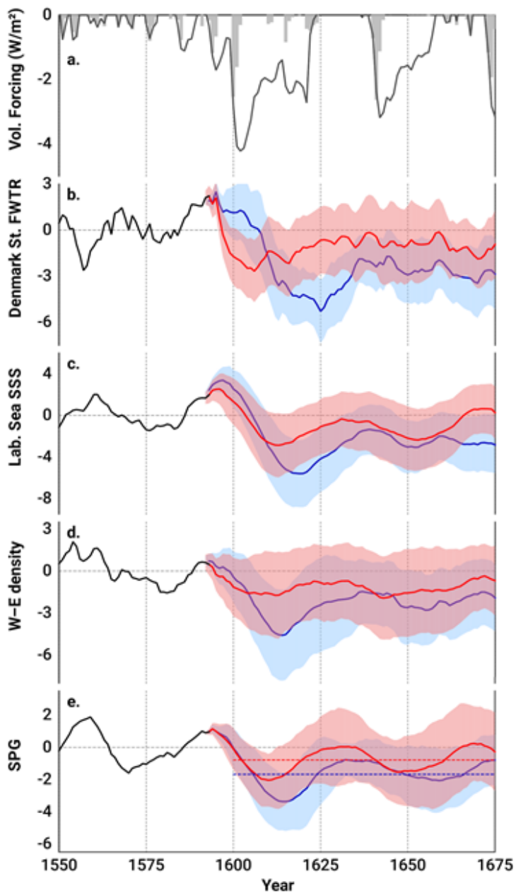
155 Figure 1: Evolution of North Atlantic climate around the 1600 Huaynaputina eruption from ensemble simulations with MPI-ESM-P (after Moreno-Chamarro et al., 2017a). Blue: realizations with a subpolar gyre (SPG) shift around 1600; red: realizations with no SPG shift. Continuous lines: means of realizations; shadings: standard deviation across realizations; dashed lines: post-1600 temporal averages showing the change in regime in the SPG. From top: (a) Accumulated global top-of-the-atmosphere radiative volcanic forcing (line) and the contribution of each individual eruption (bars), both in W/m^2 ; (b) Denmark Strait freshwater transport (FWTR), as the sum of the liquid and the sea-ice contributions (a larger negative value reflects a stronger southward export); (c) Labrador Sea sea-surface salinity (SSS); (d) West–east gradient in upper-ocean densities in the subpolar North Atlantic; and (e) SPG strength. (b–e) Time series normalized with respect to the pre-eruption period 1550–1590.
