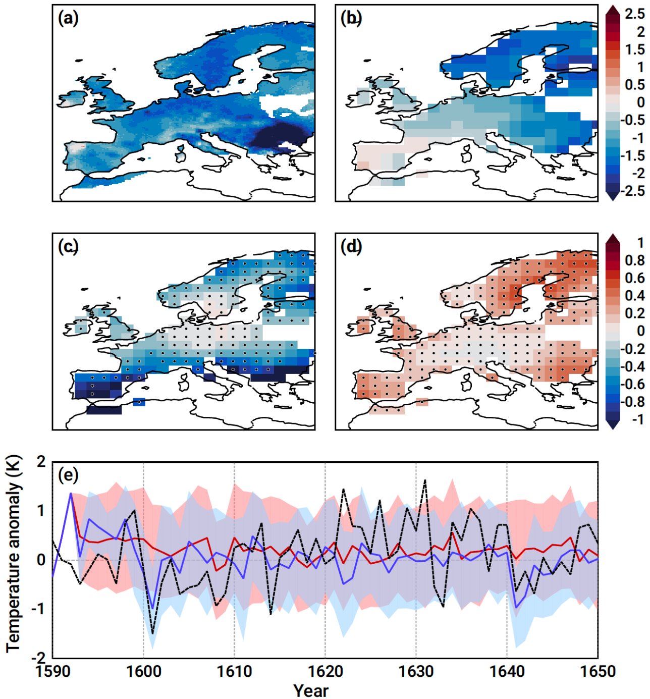
340 Figure 6: (a,b) Spatial pattern of the 1601-1602 anomaly in summer (JJA) temperature (in K; wrt 1540-1590) in (a) the NVOLC v2 reconstruction and (b) the MPI-ESM-P ensemble member r3i8, for which the spatial correlation coefficient is the largest (0.17) with the reconstruction in (a). The r3i8 is a sensitivity simulation branched in 1600 from the original simulation r3i1p1 through a slight, temporary perturbation in one atmosphere model's parameter (Moreno-Chamarro et al., 2017b). (c) Summer temperature anomaly (in K; wrt 1540-1590) of the NVOLC v2 reconstruction (black, dashed line; shifted +0.5 K) and of the ensemble with (blue) and without (red) volcanic forcing between 1593-1640 (for which thick lines are the ensemble mean and the shading is the ensemble standard deviation).
