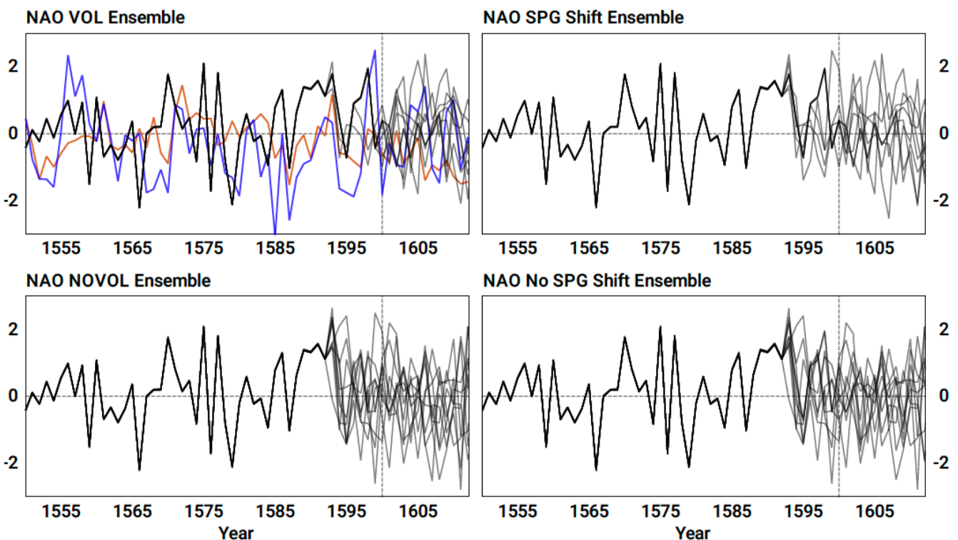
195 Figure 2: North Atlantic Oscillation (NAO) time series (defined as the first principal component of winter, DJF, sea-level pressure over the North Atlantic, 20°N–90°N and 80°W–40°E) in the MPI-ESM-P ensemble with and without volcanic forcing (left) and with and without subpolar gyre (SPG) shift (right). Two NAO reconstructions are plotted from Ortega et al. (2015; red) and Michel et al. (2020; blue).
