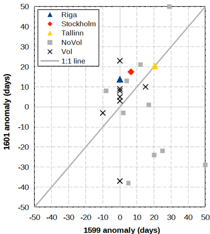
370 Figure 78. Anomaly in the sea ice breakup date in 1601 and 1599, w.r.t. the 1550-15980 period. In the MPI-ESM-P simulations, breakup dates are defined as the first day of the year when sea-ice concentration in the Baltic Sea (averaged between 10°E-30°E and 50°N-60°N) is lower than 1%, after smoothing with a 7-day running mean. This threshold ensures similar dates in the model and historical records, around early April. A breakup anomaly equal to 50 indicates that the simulation does not show a breakup date 375 in a year. Note that 6 simulations have the same 1599 anomaly, since the ensemble begins in 1600.
