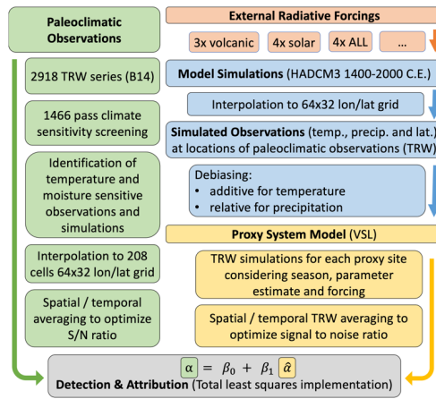
135 Figure 1: Schematic overview of the performed analysis. General steps are indicated in bold, study-specific procedures in normal text. B14 refers to the Breitenmoser et al. (2014) data set, S/N stands for signal to noise ratio, T for temperature and PREC for precipitation.
