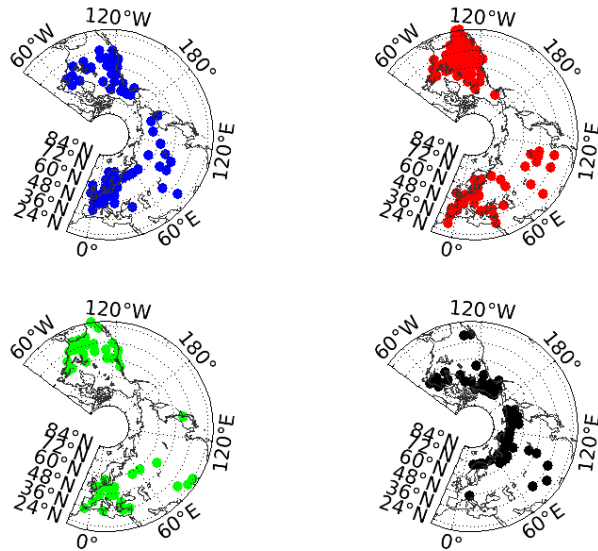
Figure 2: Limitations determined for all TRW chronologies with valid parameter sets, separated into temperature sensitive (top left), moisture sensitive (top right), both T and M sensitive (bottom left) and neither T nor M sensitive (bottom right). (Maps created with Matlab mapping package M_map (Pawlowicz, 2022))
