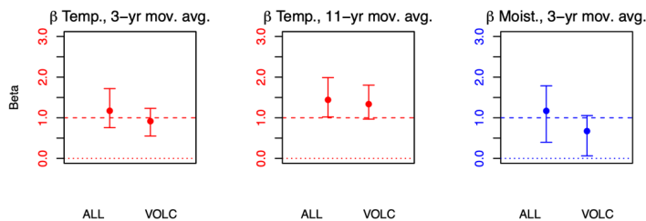
Figure 7: Left: Beta values and uncertainties for 3-year moving averages (following DelSole et al., 2019) in the TLS D&A analysis for temperature-sensitive TRW (Fig 2, top panels). ALL and VOLC indicate regression on the all-forcing and volcanic-only based TRW simulations, respectively. Middle: as in left panel, except for 11-year running means; uncertainties adjusted for serial autocorrelation. Right: as in left panel, except for moisture-sensitive TRW (Fig 2, bottom panels) but with the aggregate mean response grouped by the two regions based on the positive or negative response of the TRW simulations (Fig 6, bottom right). Uncertainty ranges are based on 90% confidence intervals of scaling factors.
