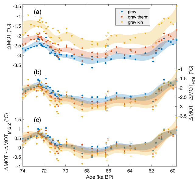
Figure A1. Comparison of mean ocean temperature (MOT) anomalies between three methods of fractionation correction. Results are for the average of the three MOT proxies (Kr/N 2 , Xe/N 2 , and Xe/Kr). Panel (a) shows results if the noble gas ratios are corrected for fractionation and no reference interval is used. Panel (b) shows the results when the noble gas ratios are reported relative to Holocene data, using the same method of fractionation correction. Panel (c) is the same as panel (b) but MOT is reported relative to MIS 2. Individual MOT data from Taylor Glacier are shown as filled symbols and the 1\sigma confidence envelope from a spline with a 2500-year cutoff period, and bootstrapping is shown using shading. WAIS Divide data are shown as open symbols.
