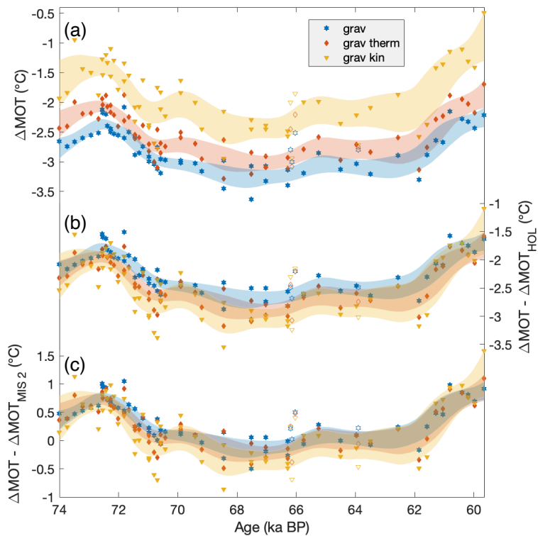
675 Figure A1: Comparison of mean ocean temperature (MOT) anomalies between three methods of fractionation correction. Results are for the average of the three MOT proxies ( \text{Kr}/\text{N}_2 , \text{Xe}/\text{N}_2 and \text{Xe}/\text{Kr} ). The top panel shows results if the noble gas ratios are corrected for fractionation, and no reference interval is used. The middle panel shows the results when the noble gas ratios reported relative to Holocene data, using the same method of fractionation correction. The bottom panel is the same as the middle, but MOT is reported relative to MIS 2. Individual MOT data are shown with x's and the 1\sigma confidence envelope from a spline with a 2500 year cutoff period.
