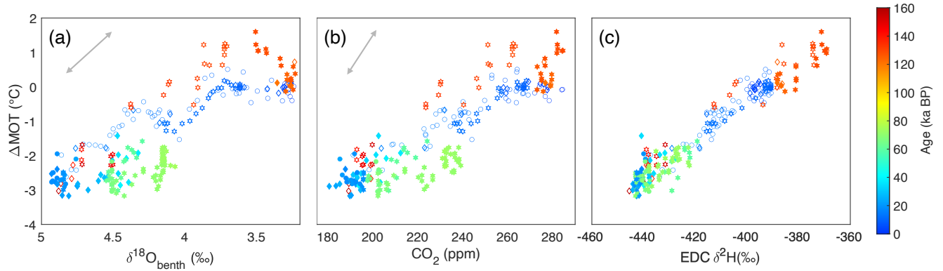
Figure 3: \Delta\text{MOT} plotted against coeval (a) \delta^{18}\text{O}_{\text{benth}} (Lisiecki and Stern, 2016), (b) atmospheric \text{CO}_2 (Bereiter et al., 2015), and (c) EDC \delta^2\text{H} (Jouzel et al., 2007) corrected for changes in seawater \delta^2\text{H} . The \delta^{18}\text{O}_{\text{benth}} , \text{CO}_2 , and EDC \delta^2\text{H} , records were linearly interpolated in order to plot against contemporaneous MOT. Additionally, the EDC \delta^2\text{H} was smoothed using a gaussian filter with a 500-year window to remove high frequency variability. Gray arrow in (c) shows the \Delta\text{MOT} - \delta^{18}\text{O} scaling from (Shackleton, 1974). Gray arrow in (b) shows \Delta\text{MOT} - \text{CO}_2 relationship for the solubility pump from the carbon cycle model. Filled symbols include data from the last interglacial through glacial maximum (129 – 18 ka) to highlight the glacial inception, while open symbols indicate data from the last and penultimate deglaciations and the Holocene. Diamonds indicate MOT data constructed from the EDC record (Baggenstos et al., 2019; Shackleton et al., 2020), circles show data from WAIS Divide ((Bereiter et al., 2018a) and this study)), and stars show MOT data from Taylor Glacier ((Shackleton et al., 2019, 2020) and this study). Color of data indicate the age.
