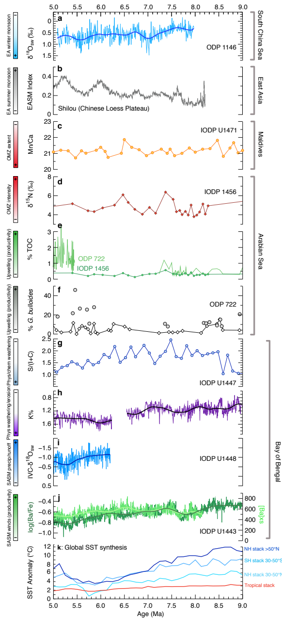
Figure 11: Compilation of late Miocene (9-5 Ma) Asian monsoon reconstructions, showing representative records from different regions and their published interpretations (bars on left).
