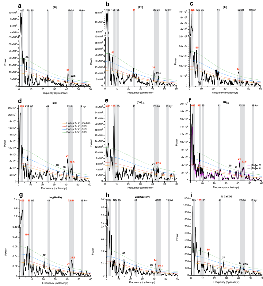
Figure 8: Spectral analyses for over the 9 to 5 Ma interval (log ratios and % CaCO 3 ) or 8.15 to 5 Ma interval (calibrated element concentrations and [Ba] xs ). a: [Ti], b: [Fe], c: [Al], d: [Ba], e: [Ba] cfb (carbonate free basis), f: [Ba] xs , g: log(Ba/Fe), h: log(Ca/Terr), i: % CaCO 3 . Grey bands denote primary orbital periods based on the La04 astronomical solution. The 22-24 kyr band covers two peaks centred at 23.5 and 22.3 kyr.
