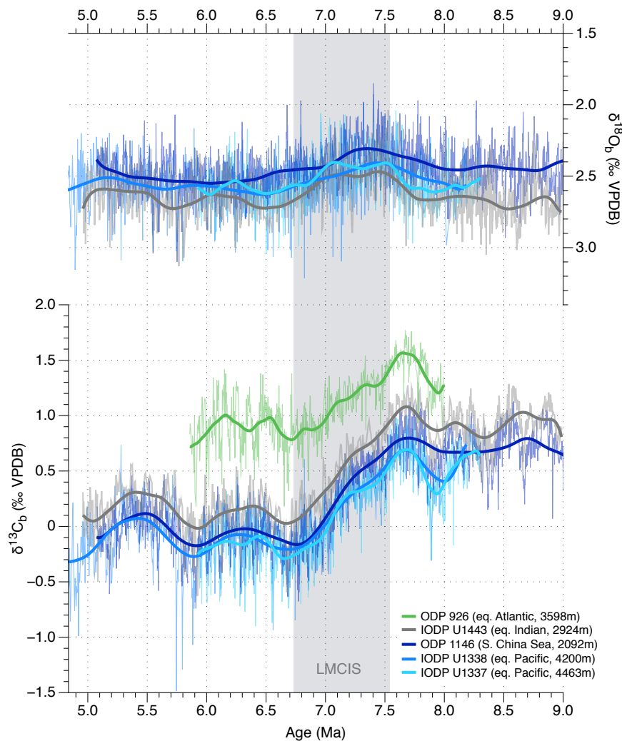
930 Figure 5: Late Miocene evolution of low-latitude deep-ocean inter-basin benthic \delta^{13}\text{C} and \delta^{18}\text{O} gradients. South China Sea ODP Site 1146 (Holbourn et al., 2018) with age model revised in Holbourn et al. (2021), equatorial Pacific IODP Sites U1338 (Drury et al., 2018; 935 Drury et al., 2016) and U1337 (Drury et al., 2017), and ODP Site 926 (Shackleton and Hall, 1997; Drury et al., 2017; Zeeden et al., 2013). All records are shown on their latest independent orbitally tuned chronologies. We have excluded Caribbean ODP Site 999 from this figure because it is bathed in intermediate water masses due to basin geometry and sill depths (Bickert et al., 2004). Deep South Atlantic Site 704 (Müller et al., 1991) data are not plotted due to clear age model discrepancies when compared to orbitally tuned records. All \delta^{18}\text{O} records are based on Cibicidoides wuellerstorfi or C. mundulus therefore no corrections 940 are applied, following (Jöhneck et al., 2021). The Site 926 record includes \delta^{13}\text{C} corrections for some samples due to the multispecific nature of the record (Drury et al., 2017). No correction was applied to C. wuellerstorfi or C. mundulus \delta^{13}\text{C} values.
