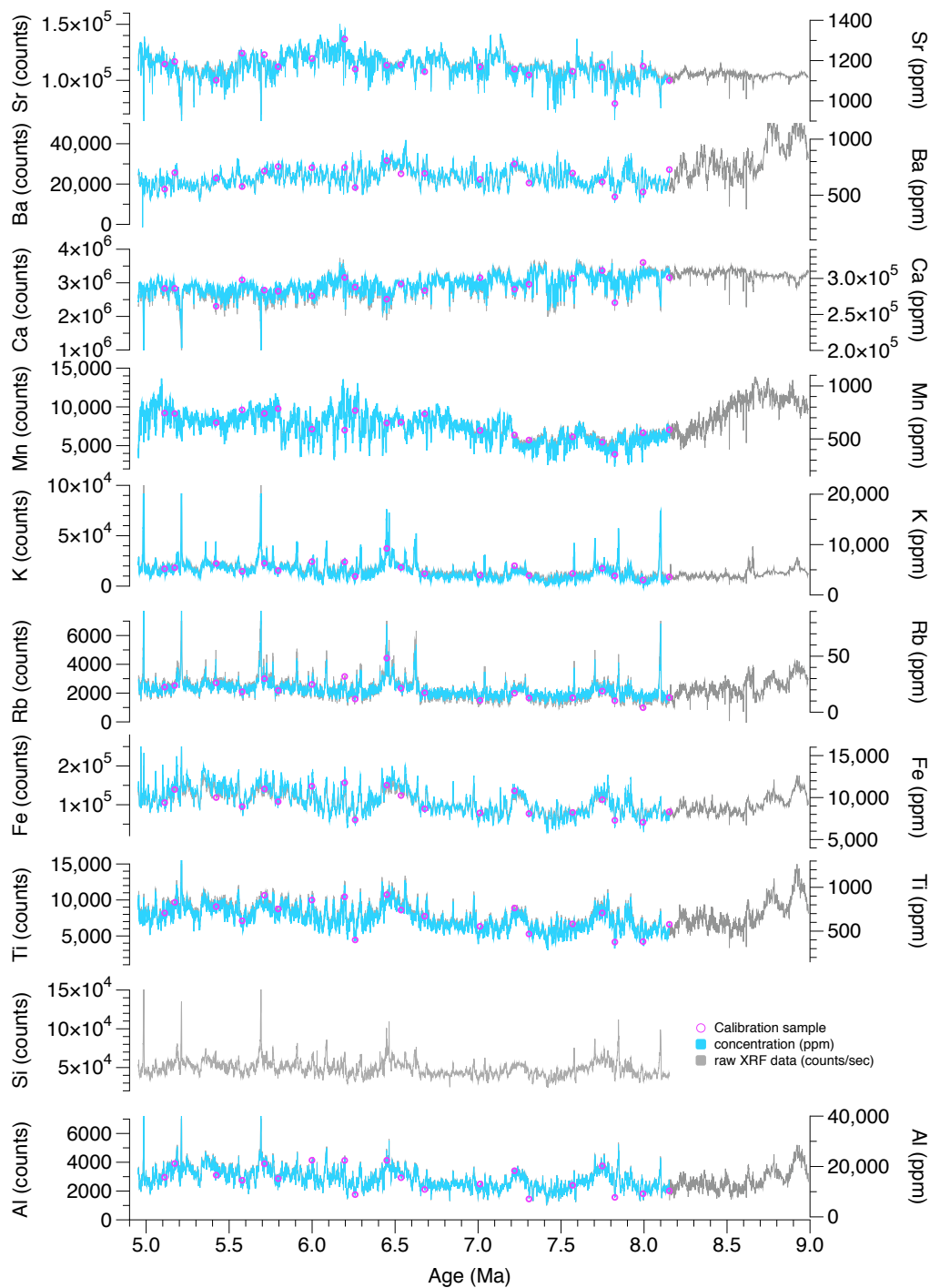
Figure 6: Raw counts/sec (grey lines) and calibrated concentration (blue lines) scanning XRF elemental data over the late Miocene interval. Pink circles show samples used for calibration (See Fig. S3).
