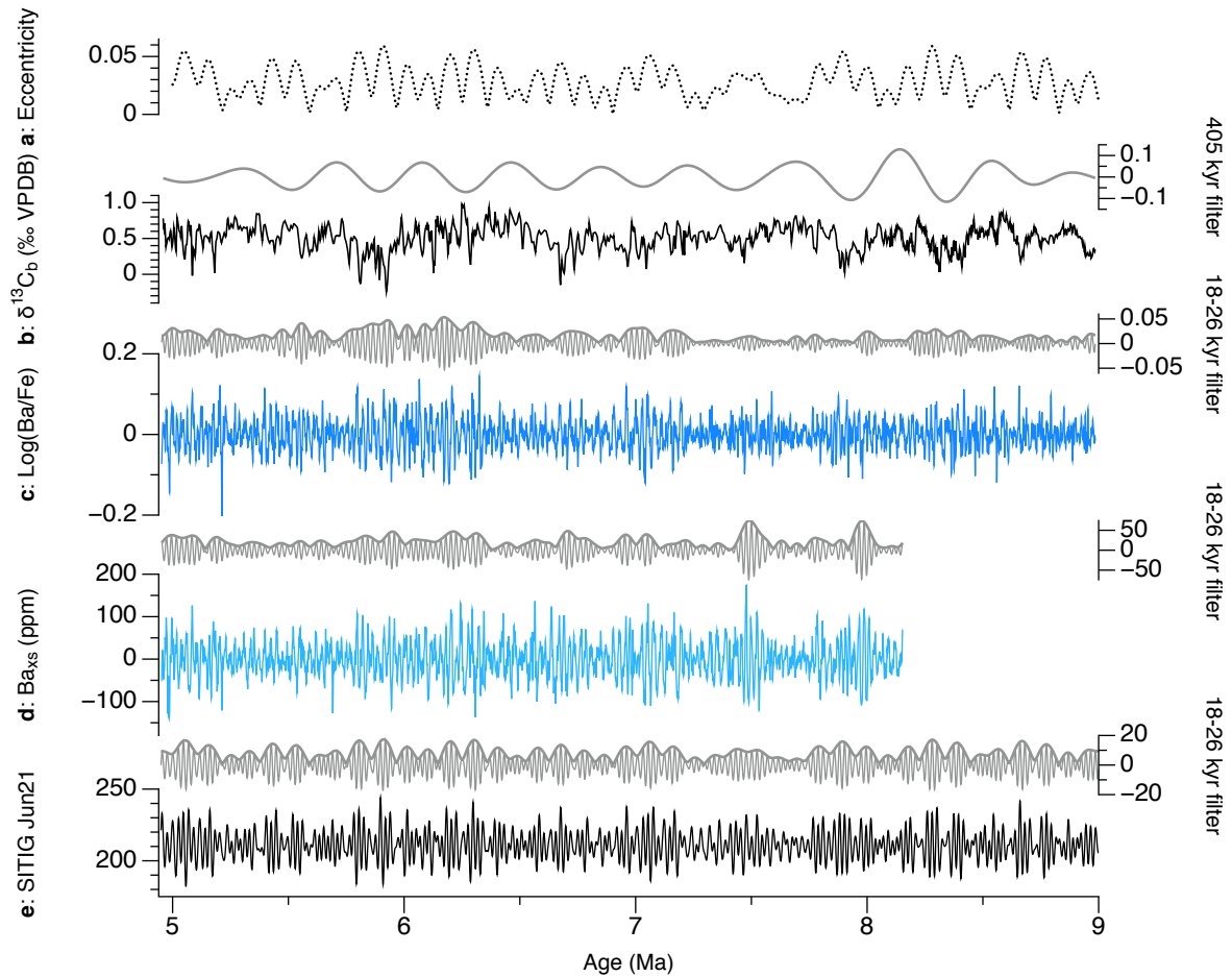
Figure 10: Detrended and filtered late Miocene U1443 records to illustrate precession-band variance and amplitude modulation. a: eccentricity (Laskar et al., 2004), b: benthic \delta^{13}\text{C} (bandpassed as in Fig. 9) and its 405-kyr filter (above) (note reversed y-axes). c: Lowess-detrended \log(\text{Ba}/\text{Fe}) (window = 0.1 Ma) and 18 to 26 kyr filter (above), d: Lowess-detrended \text{Ba}_{\text{xs}} (window = 0.1 Ma) and its 18 to 26 kyr filter (above), e: The summer inter-tropical insolation gradient (SITIG, calculated as the insolation difference between 23^\circ\text{N} and 23^\circ\text{S} on 21 st June using orbital solution of Laskar et al. (2004)) and its 18 to 26 kyr filter and amplitude modulation (above); For panels c-e , raw datasets were filtered using a Tanner-Hilbert filter centred on 46.5 cycles/Myr with bandwidth \pm 8 (designed to include all precession terms with periods between 18 and 26 kyr). For panel b , a Tanner-Hilbert filter centred on 2.47 cycles/myr with bandwidth \pm 0.8 was applied.
