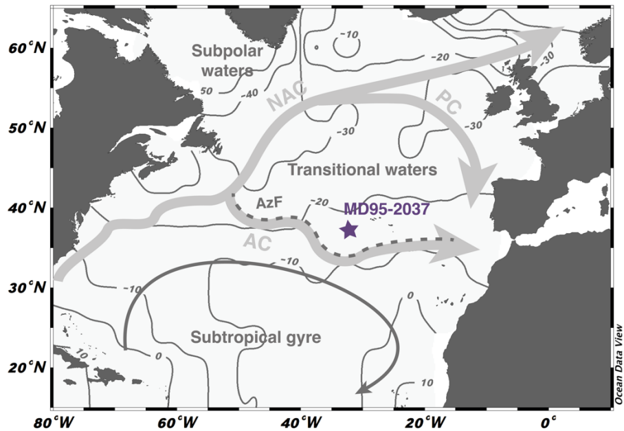
700 Figure 1: Location and hydrological settings of core MD95-2037. The core lies north of the Azores Current (AC) and the associated Azores Front (AzF), a branch of the North Atlantic Current (NAC). It is located in the transitional waters delimited to the north by the Portugal Current (PC). Site location overlays a map of mean annual \Delta p\text{CO}_2 (in ppm, Takahashi et al 2011) compiled with the Ocean Data View software (Schlitzer, 2018, http://odv.awi.de ). Regions with positive (negative) values are sources (sinks) for atmospheric \text{CO}_2 .
