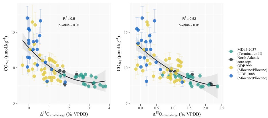
Figure 5: Coccolith differential vital effect sensitivity to changes in aqueous \text{CO}_2 since the Miocene. Differential vital effects are more important in the Late Pleistocene and modern-day ocean than during the Miocene. The correlation between aqueous \text{CO}_2 and differential vital effects in carbon ( R^2 = 0.5 ) or oxygen ( R^2 = 0.52 ) suggests that an increase in carbon limitation might be responsible for the observed change. Coccolith vital effect datasets are from (Bolton et al., 2012) for the Miocene and Pliocene, and Candelier et al. 2013 and Hermoso et al. 2015 for the North Atlantic core-tops. The \text{pCO}_2 records used to compute aqueous \text{CO}_2 for the Miocene and Pliocene datasets are from Rae et al., 2021. SST data for site 1088 are from Herbert et al. 2016. For site 999 we took the composite SST record from Rae et al., 2021, as no SST dataset spanned the whole of the differential vital effect record for site 999. Core-top \text{CO}_2 concentrations were calculated using a pre-industrial \text{pCO}_2 of 280 ppm and SST data from WOA13 (Locarnini et al., 2013).
