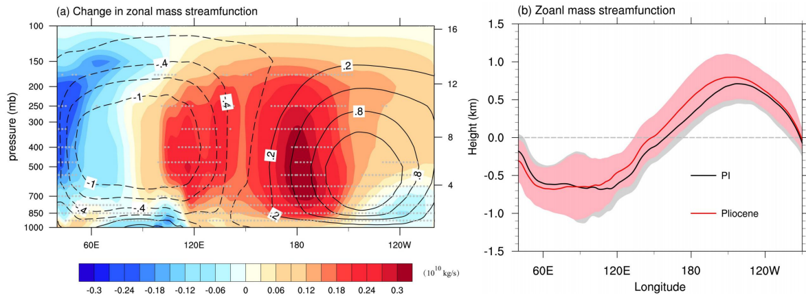
Figure 11: (a) Changes in ZMS (shading, unit: 10^{10} \text{ kg s}^{-1} ) averaged between 10^{\circ}\text{S/N} for the mid-Pliocene with respect to the PI simulation, overlaid by the climate mean ZMS for the PI simulation (contours). The zonal wind \vec{V}_Z is used to calculate ZMS, which is decomposed from the 3P-DGAC method. The contours represent the climate mean ZMS for the PI simulation. Solid curves indicate a positive value, and dashed curves show a negative value. Stippling indicates regions where at least 10 of 13 simulations in the model group agree on the sign of the ensemble mean. (b) is the vertical integrated ZMS in (a). The gray and pink shading indicates 1 standard deviation of individual models departure from the MMM mean of MSF for the PI and mid-Pliocene simulations, respectively.
