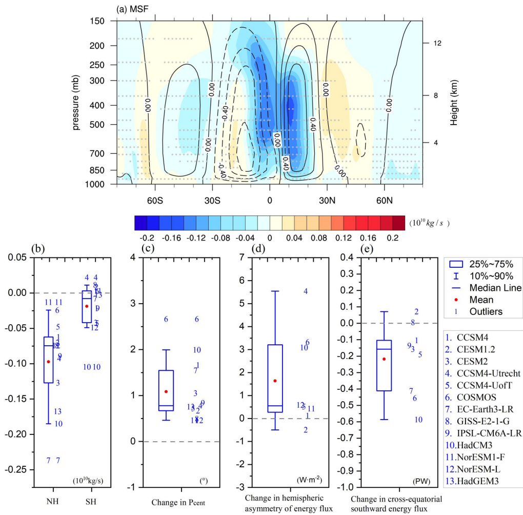
435 Figure 8: (a) Changes in annual mean MSF (shading; units: 10^{10} \text{ kg} \cdot \text{s}^{-1} ) of meridional circulation for mid-Pliocene with respect to the PI simulation, overlaid by the climate mean MSF for the PI simulation (contours). The meridional wind \vec{V}_M is decomposed from the 3P-DGAC method. Solid curves indicate positive values, and dashed curves indicate negative values. Stippling indicates regions where at least 10 of 13 simulations in the model group agree on the sign of the ensemble mean. (b) Changes in annual mean intensities (unit: 10^{10} \text{ kg/s} ) of meridional circulation in the NH and SH. (c) The latitudes of the center of annual mean precipitation between 20^\circ\text{S} and 20^\circ\text{N} (unit: ^\circ ). (d) Hemispheric asymmetry (NH minus SH) of energy flux into the atmosphere (unit: \text{W} \cdot \text{m}^{-2} ). (e) Changes in the integrated atmospheric meridional heat transport across the equator (unit: PW).
