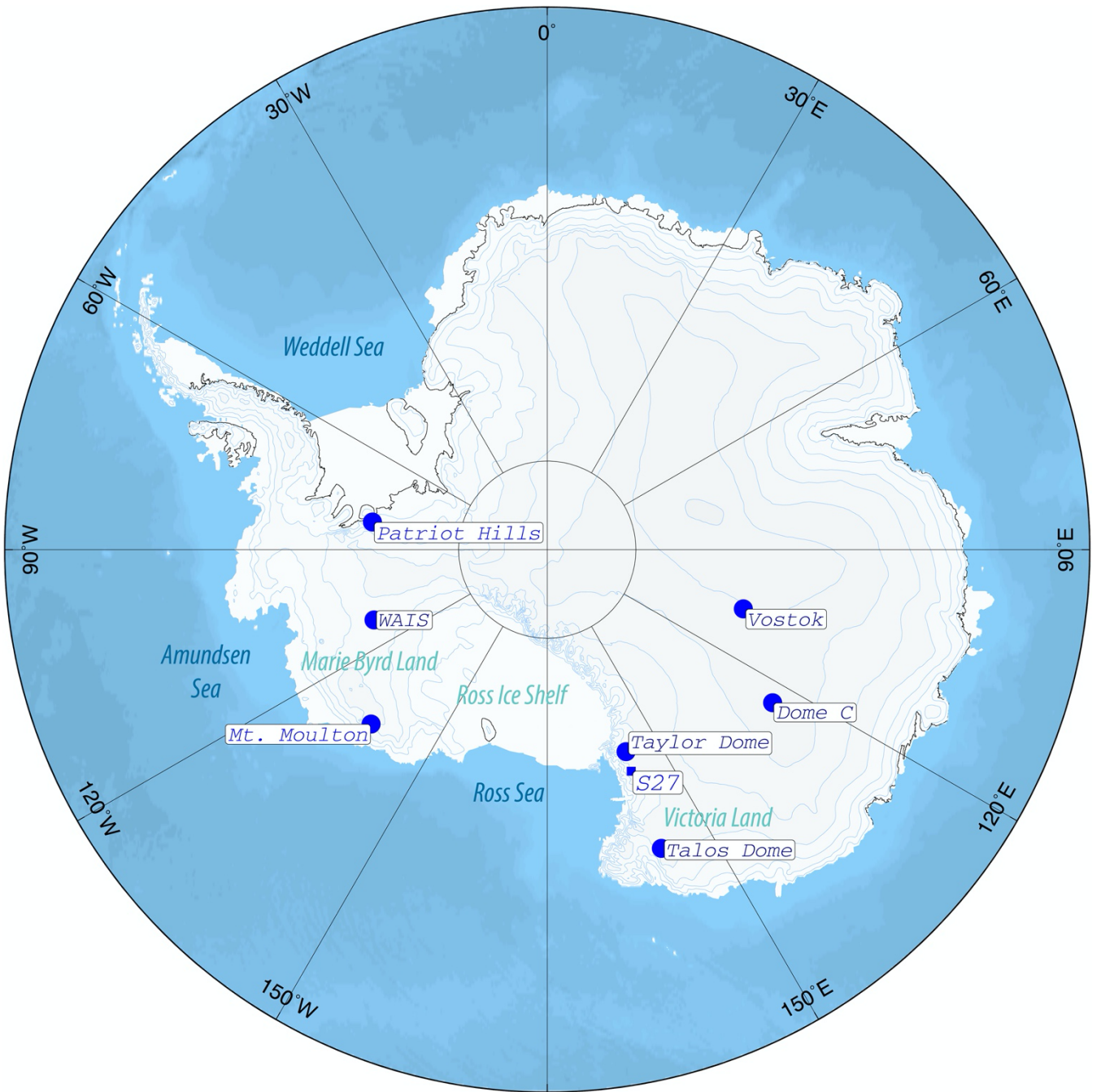
Figure 1: Locations of key ice coring sites and geographic features of Antarctica. The square indicates the location of Site 27 (S27). Other ice coring sites mentioned in this study are marked with blue circles (map source: Bindshadler et al, 2011).
