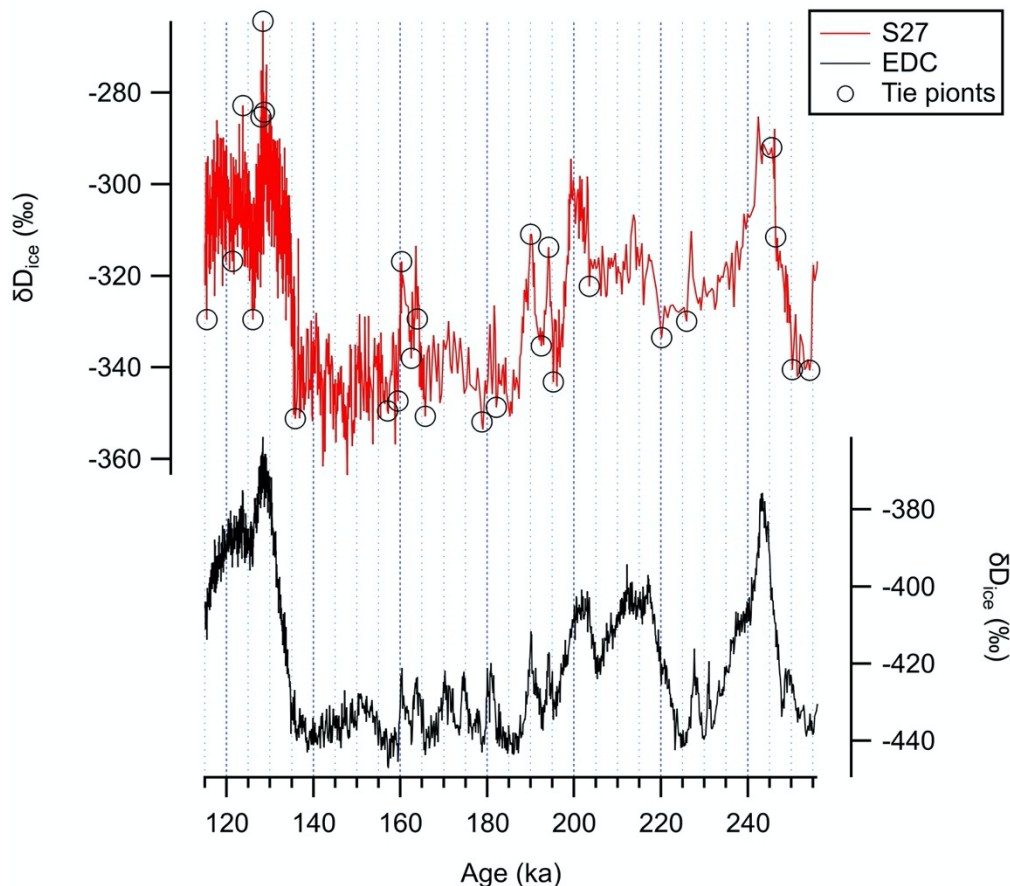
Figure 2: Stable water isotope records in S27 (red; Spaulding et al, 2013) and EDC (black; Jouzel et al, 2007) between 115 and 255 ka. Tie-points in S27 \delta\text{D}_{\text{ice}} used by Spaulding et al (2013) are marked as circles.
