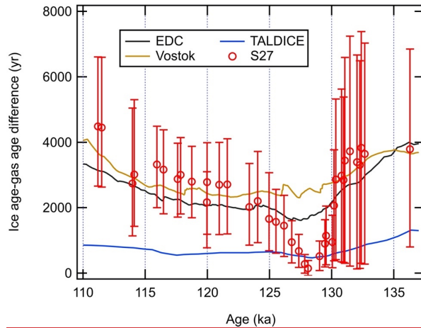
375 Figure 7: Ice age-gas age difference ( \Delta age) between 110 and 136 ka in S27 (red), Talos Dome (TALDICE; blue), Vostok (brown), and EDC (black). This age interval corresponds to the depth range of 10.05 to 134.55 m in S27, where the measured samples are free from any visible fractures . TALDICE, Vostok, and EDC \Delta age data are from Bazin et al (2013) and references therein. All four \Delta age records show similar pattern during the Termination II, with minimum values reached around ~128 ka. Error bars in S27 data represent the 95% confidence interval of the \Delta age estimates. Note that the Age values are plotted on the gas age scale and the confidence intervals of the S27 \Delta age points are asymmetrical .
