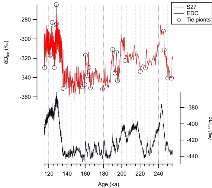
85 Figure 2: Stable water isotope records in S27 (red; Spaulding et al, 2013) and EDC (black; Jouzel et al, 2007) between 115 and 255 ka. Tie-points in S27 \delta D_{ice} used by Spaulding et al (2013) are marked as circles.
