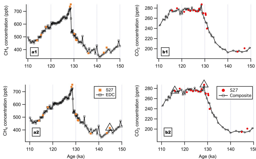
345 Figure 5: CH 4 and CO 2 measured in S27 plotted on the timescale developed solely on \delta^{18}\text{O}_{\text{atm}} (a1 and b1) and on the chronology after greenhouse gas synchronization (a2 and b2). Tie points and anchor points are marked in triangles. EDC CH 4 data are from Loulergue et al (2008), composite CO 2 data from multiple ice cores are from Bereiter et al (2015) and references therein, and the timescale (AICC2012) is from Veres et al (2013) and Bazin et al (2013).
