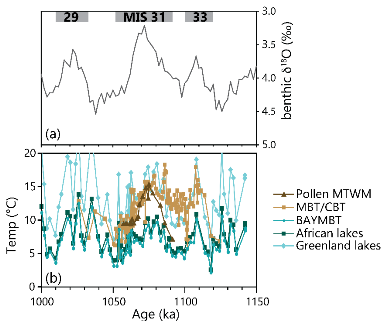
340 Figure 5: Comparison of brGDGT calibration during MIS 31 with pollen-derived temperature estimates (Melles et al., 2012). A) The global benthic oxygen isotope stack (Lisiecki and Raymo, 2005) with the different marine isotope stages (MIS) is indicated at the top for reference. B) Lake El'gygytgyn brGDGT temperature estimates using the calibrations of Zhao et al. (2021) based on Greenland lakes, the African lakes MBT' 5ME calibration of Russell et al. (2018), the MBT/CBT calibration of Sun et al. (2011) (this is the previously published dataset from de Wet et al. (2016)), the BayMBT calibration (Martínez-Sosa et al., 2021) and pollen mean temperature of the warmest month (MTWM) from Melles et al. (2012). Additional brGDGT calibrations are shown in Fig. S8. Note 345 how the BayMBT and African lakes calibrations yield similar results and nearly plot on top of each other.
