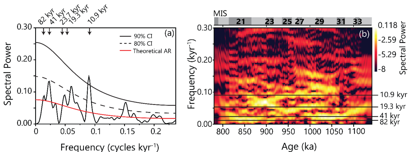
250 Figure 4: Frequency analysis of Lake El'gygytyn MBT' 5ME data from 1142 to 752 ka. A) Lomb-Scargle periodogram, with the 80% and 90% confidence levels as well as the theoretical autoregression levels. B) Short-time Fourier transformation showing the evolutionary power spectrum, with the dominant peaks from (A) indicated with horizontal lines. Marine Isotope Stages (MIS) are indicated along the top. Both analyses were performed using PAST3 (Hammer et al., 2001).
