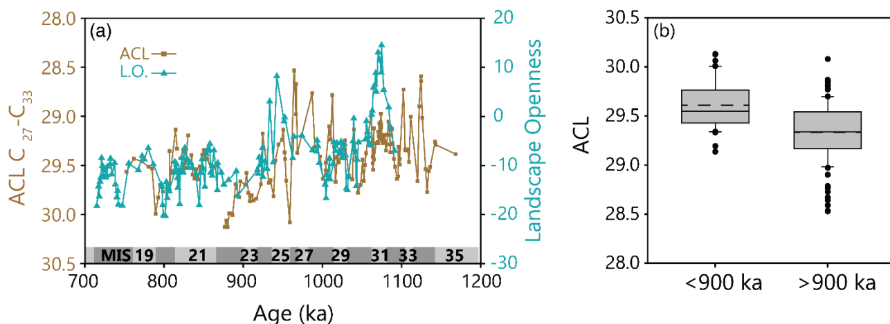
195 Figure 2: Comparison of Lake El'gygytgyn n -alkane and pollen data. A) The ACL of the C 27 -C 33 n -alkanes plotted along with the
