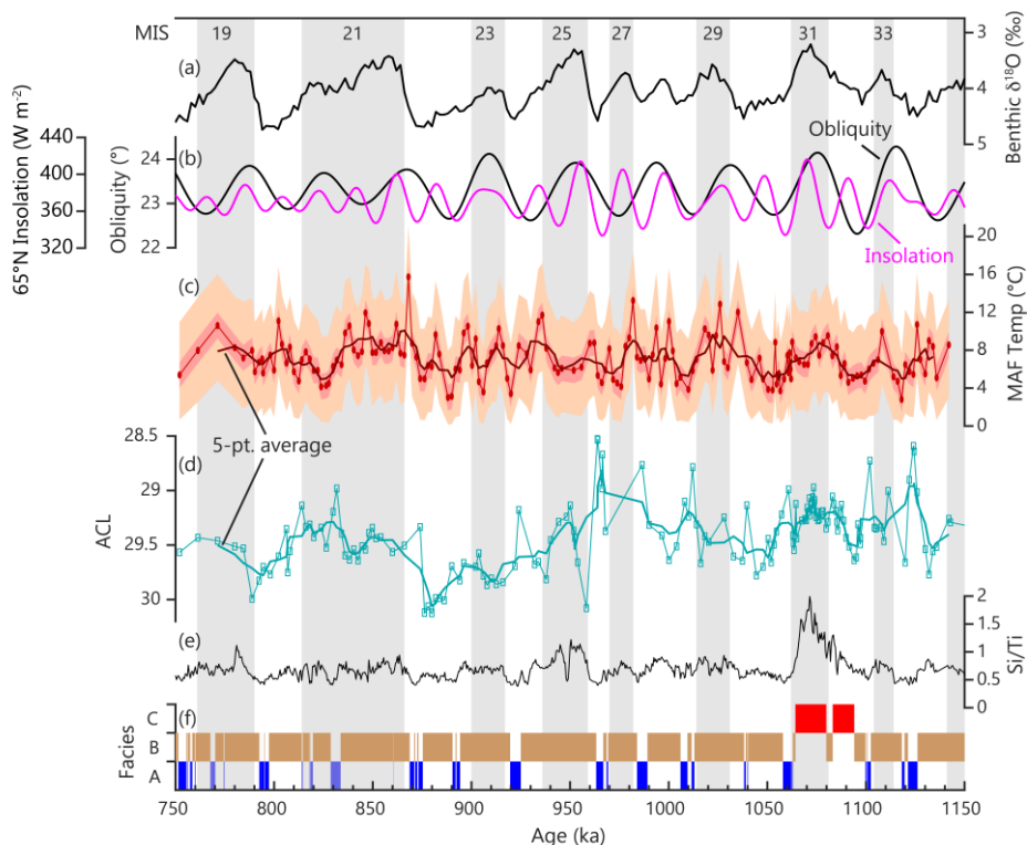
225 Figure 3: Lake El'gygytyn data with Marine Isotope Stages (MIS) notated at the top and with interglacials indicated by the grey shading. A) The global benthic oxygen isotope stack (Lisiecki and Raymo, 2005). B) Astronomical forcing, including obliquity and summer insolation (June 21-Sept 21) at 65 °N latitude (Laskar et al., 2004). C) brGDGT-inferred temperature of the months above freezing (MAF Temp). Dark shading represents the 1 \sigma analytical uncertainty based on triplicate MBT' 5ME analyses converted to temperature using BayMBT (1 \sigma = 1.35 °C, n=12), while light shading represents the calibration uncertainty (Martínez-Sosa et al., 2021). D) n -alkane ACL based on C 27 -C 33 . E) Lake El'gygytyn silica (Si) to titanium (Ti) ratio (Melles et al., 2012; Wennrich et al., 2013); F) Summary of lithological facies in core 5011-1. Facies A (blue bars) represents glacial intervals. Facies B (brown bars) is cosmopolitan, occurring during both glacials and interglacials. Facies C (red bars) represents superinterglacials. 230
