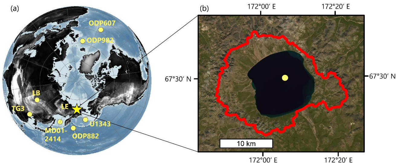
Figure 1: Study location. a) Map showing the location of Lake El'gygytyn (star) and other key sites discussed in the text (yellow circles) including Ocean Drilling Program (ODP) Sites 882 (Martínez-García et al., 2010), 607 (Sosdian and Rosenthal, 2009), 982 (Lawrence et al., 2009) and International Ocean Discovery Program (IODP) Site U1343 (Kender et al., 2018), MD01-2414 (Lattaud et al., 2018), and Tianjin-G3 loess profile (Zhou et al., 2018). B) Satellite image of Lake El'gygytyn. The yellow dot represents the coring location of ICDP Site 5011-1 in the central lake basin and the red outline designates the lake's watershed. World imagery sources: Esri, Maxar, GeoEye, Earthstar Geographics, CNES/Airbus DS, USDA, AeroGRID, IGN, and the GIS User Community.
