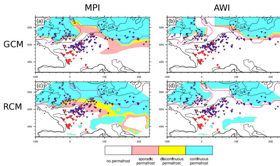
Figure 6. Permafrost distribution based on the surface frost index (SFI) in approximately 70 cm depth as simulated by the global MPI ( a ) and the global AWI simulation ( b ) and their respective regional counterpart ( c and d ). Ice wedge pseudomorphs, composite, and sand wedges from Andrieux et al. (2016) and Isarin et al. (1998) are denoted by purple, grey, and red triangles respectively. Black line: LGM coastline, pink line: LGM ice sheet.
