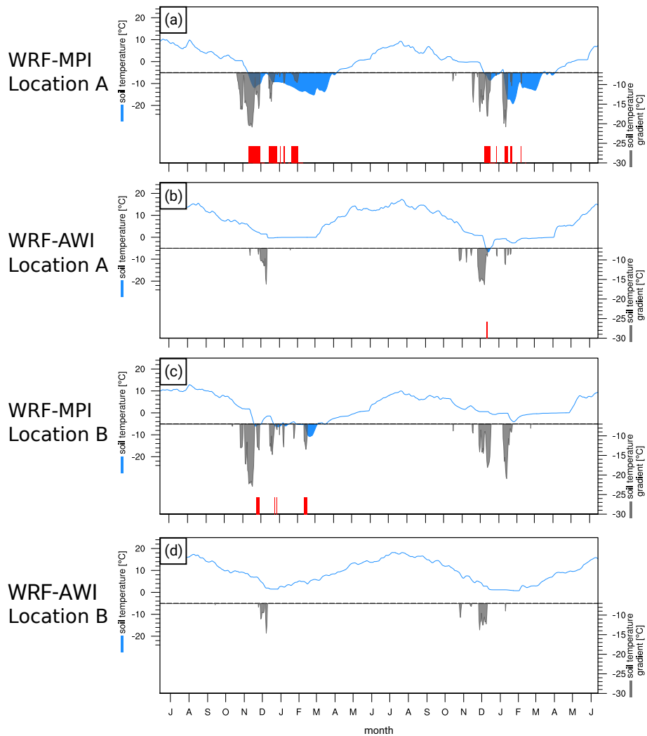
Figure 7. Time series of the daily mean soil temperature and soil temperature gradient in location A and B as denoted in Fig. 1 (A: model grid point 49.8° N, 2.49° E; B: model grid point 46.1° N, -0.33° E) as simulated in WRF-MPI (a and c) and in WRF-AWI (b and d) for two consecutive years. Blue lines show the development of the soil temperatures in layer 3 (70 cm). When the temperatures fall below -5 °C, the first condition for thermal contraction cracking after Matsuoka et al. (2018) is fulfilled, marked with blue shading and the reference line. The soil temperature gradient between the first layer (5 cm depth) and the third layer (grey shading) is only depicted when condition two after Matsuoka et al. (2018) is fulfilled, with a gradient below -7\text{ }^{\circ}\text{C m}^{-1} . Red lines indicate the coincidence of the two conditions.
