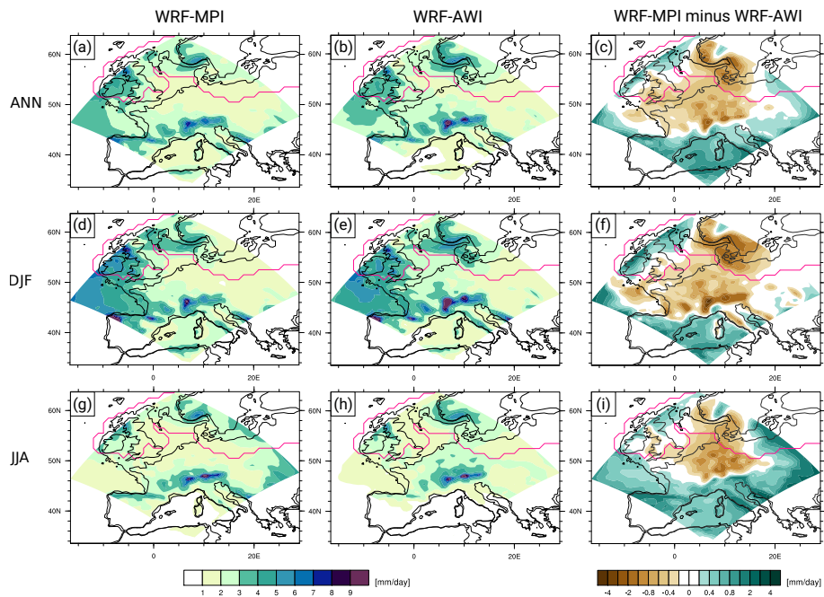
Figure 4. Distribution of total precipitation in annual ( a-c ) and seasonal winter ( d-f ) and summer ( g-i ) means as simulated with the regional WRF model with MPI forcing ( a, d and g ) and with AWI forcing ( b, e and h ) and their differences ( c, f and i ). Black line: LGM coastline, pink line: LGM ice sheet.
