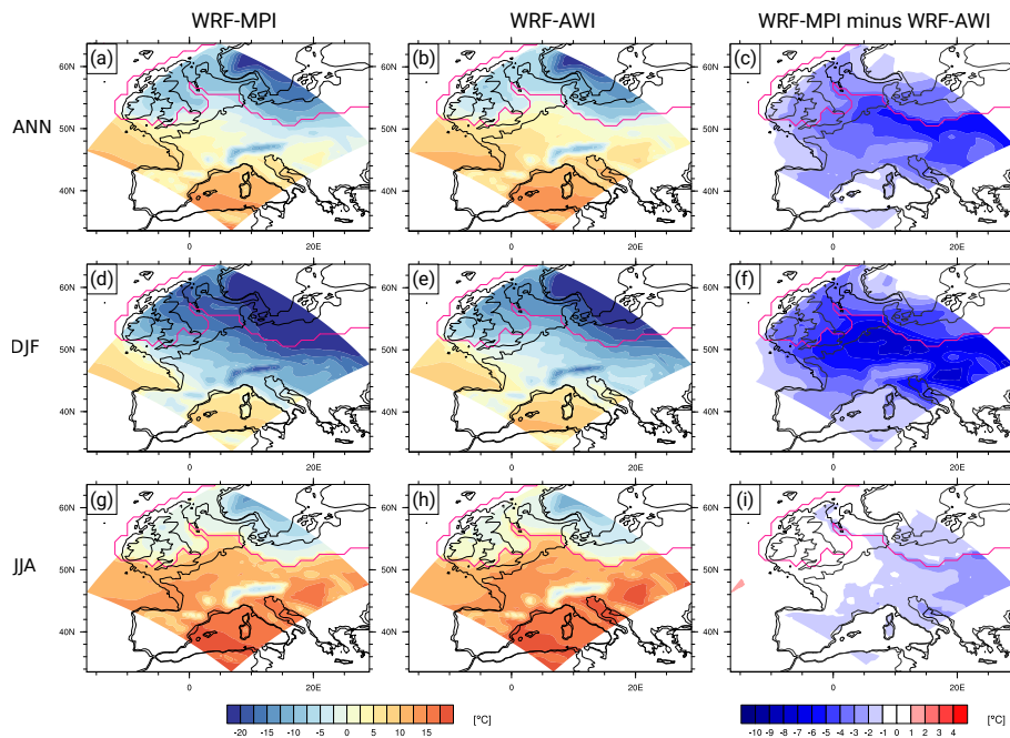
Figure 3. Distribution of 2 m air temperature in annual ( a-c ) and seasonal winter ( d-f ) and summer ( g-i ) means as simulated with the regional WRF model with MPI forcing ( a, d and g ) and with AWI forcing ( b, e and h ) and their differences ( c, f and i ). Black line: LGM coastline, pink line: LGM ice sheet.
