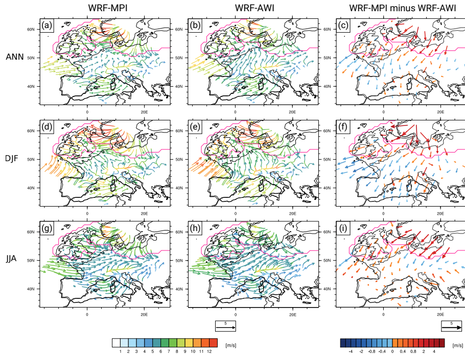
Figure 5. Distribution of 10 m wind speed in annual ( a-c ) and seasonal winter ( d-f ) and summer ( g-i ) means as simulated with the regional WRF model with MPI forcing ( a, d and g ) and with AWI forcing ( b, e and h ) and their differences ( c, f and i ). Black line: LGM coastline, pink line: LGM ice sheet.
