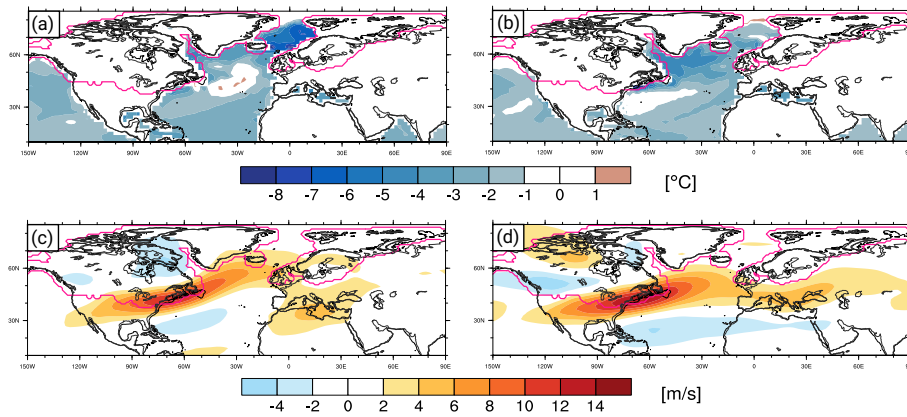
Figure 2. (a) Distribution of annual mean SST differences between the global MPI simulations under LGM and PI conditions. (b) as (a) but for the global AWI simulations. (c) and (d) as (a) and (b) but for the annual mean wind speed in 300 hPa.
