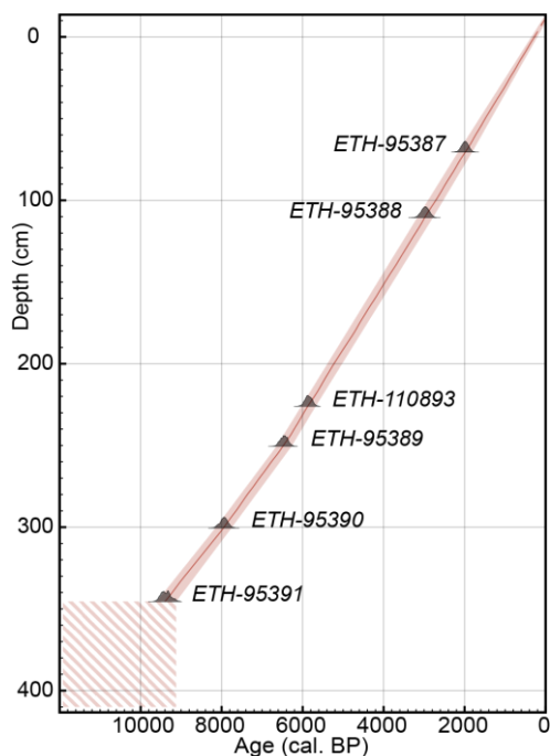
Figure 4: Age-depth model of core DA17-NG-ST07-73G based on six AMS 14C dates and on the comparison with Rumohr core DA17-NG-ST7-72R. The shading in pink illustrates the 2-sigma uncertainty range of the model. The hatched box in the bottom of the core indicates an interval containing reworked microfossils and is therefore of uncertain age (see pink shading on Fig. 3).
