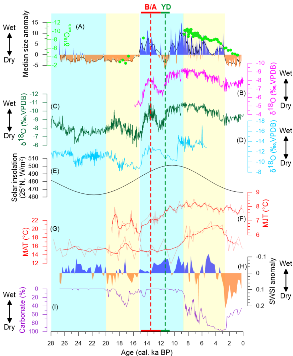
Figure 5. (A) Median size and \delta^{18}\text{O}_{\text{carb}} from Yilong Lake; Stalagmite \delta^{18}\text{O} records from (B) Sanbao Cave (Cheng et al., 2016), (C) Dongge Cave (Dykoski et al., 2005) and (D) Xiaobailong Cave (Cai et al., 2015); (E) Summer insolation curve for 25^\circ\text{N} ; (F) chironomid-mean July temperature (MJT) from Tiancai Lake (Zhang et al., 2019a); (G) brGDGT-derived mean annual temperature (MAT) from Qionghai Lake (Wang et al., 2020); (H) pollen-based reconstructed SWSI for Yilong region; (I) carbonate content of sediments from Yilong Lake.
