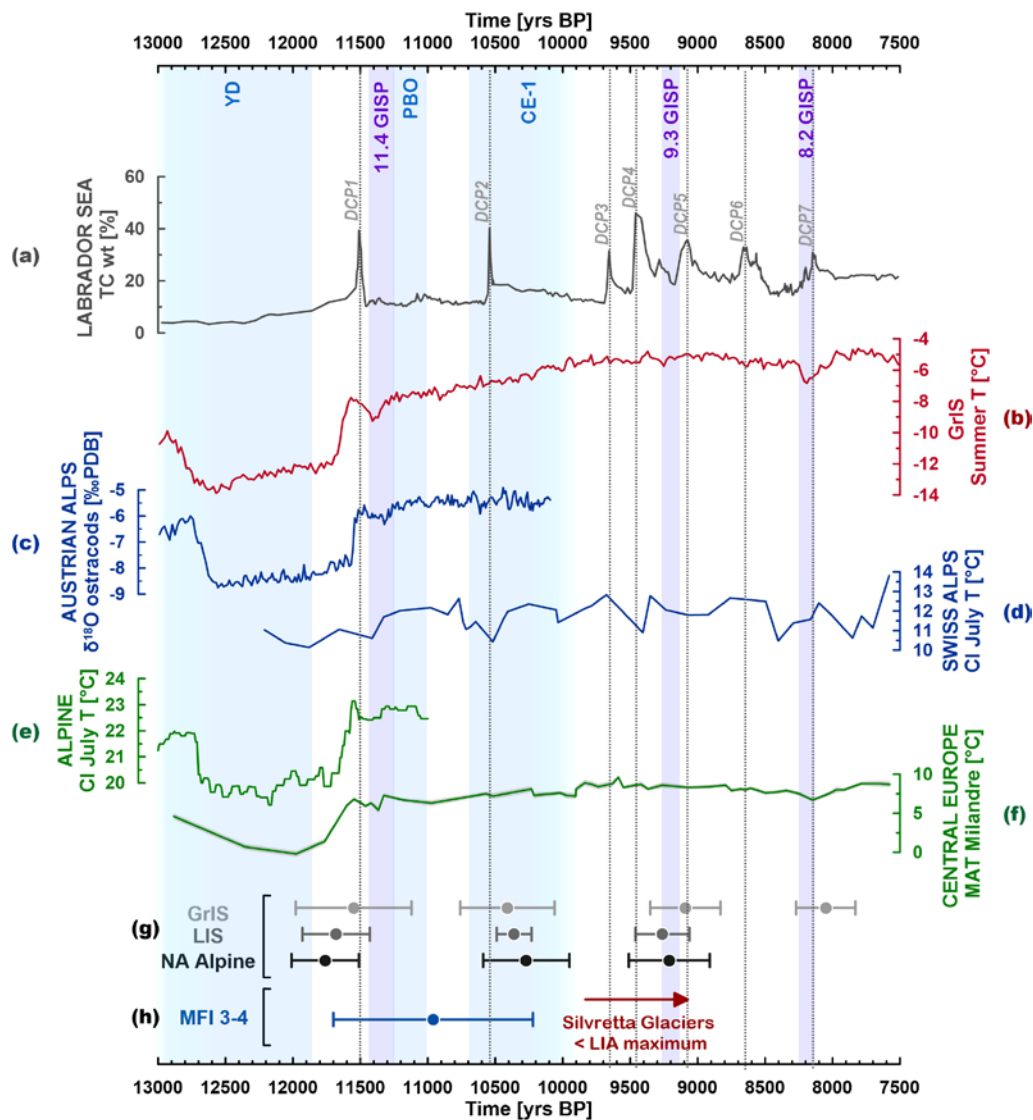
520 Figure 9: Proxy records capturing the YD-EH transition. (a) Detrital Carbonate Peaks (DCP) identified in marine sediment cores from the Labrador sea (Jennings et al., 2015); TC – Total Carbonate. (b) Mean summer temperature reconstructions (JJA) derived from nine Greenland ice cores (Buizert et al., 2018). (c) Ostracods record extracted from lake sediments of Mondsee (Austrian Alps) (Lauterbach et al., 2011). (d) Chironomid-inferred (CI) atmospheric July temperatures from lake sediments of Hinterburgsee in the Swiss Alps. (e) Stacked CI July temperatures in the European Alps (Heiri et al., 2014). (f) Mean Annual Temperatures (MAT) in Central Europe reconstructed based on speleothems from Milandre Cave, Switzerland (Affolter et al., 2019). (g) Arctic moraine record: GrIS – Greenland Ice Sheet moraines, LIS – Laurentide Ice Sheet (LIS) moraines, NA Alpine – North America Alpine mountain glacier moraines (Young et al., 2020). (h) Moraine Formation Interval (MFI) identified in this study. Purple bars highlight 525 Holocene cold events detected in Greenland ice cores (Rasmussen et al., 2007).
