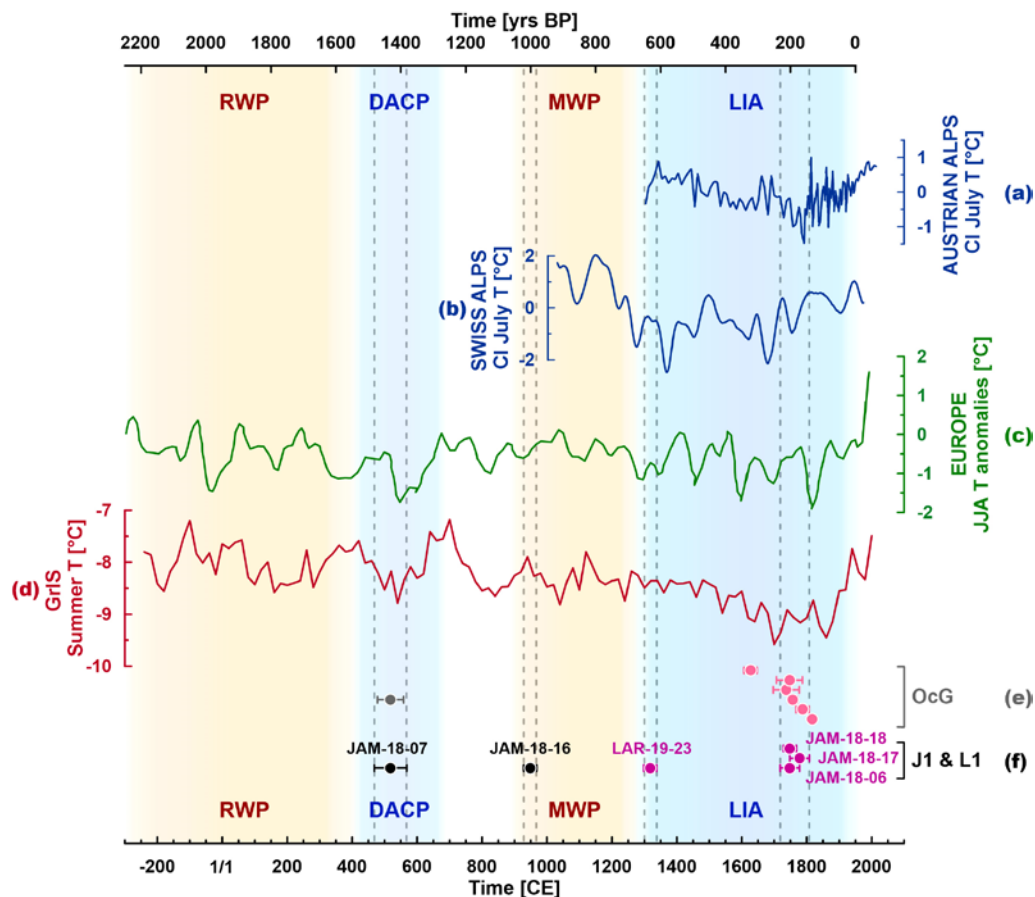
420 Figure 8: Youngest part of the ^{10}\text{Be} chronology from Jamtal and Laraintal correlated with climate proxy data from the Alps (local records in dark blue), Europe (green) and the Greenland Ice Sheet (GrIS in red) covering the past c. 2000 yrs. Proxy records indicate cooler climate conditions during the Dark Ages Cold Period (DACP) and during the Little Ice Age (LIA), synchronous with periods of moraine formation in the Silvretta region. Chironomid-inferred (CI) July temperatures from (a) Mutterbergersee in the Stubai Alps, Austria (Ilyashuk et al., 2019) approximately 70 km E of study site (north of the Alpine drainage divide) and (b) lake Silvaplana around 60 km SW of study site (Engadin, Switzerland; south of the Alpine drainage divide) (Larocque-Tobler et al., 2010a). (c) European summer temperature anomalies (reference period 1961-1990, 60-year low-pass filter) identified in tree-ring chronologies (Büntgen et al., 2011). (d) Mean summer temperature reconstructions (JJA) derived from nine Greenland ice cores (Buizert et al., 2018). (e) ^{10}\text{Be} ages of boulders sampled from the presumable LIA (Holocene composite moraine) from Ochsental (OcG) (Braumann et al., 2020) and from (f) Jamtal and Laraintal (this study). RWP – Roman Warm Period; MWP – Medieval Warm Period.
