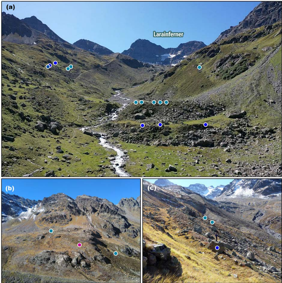
275 Figure 5: Photographs of Laraintal. (a) Terminal moraine section with sample locations marked with circles. (b) Left lateral valley flank with LAR-19-22 (cyan), LAR-19-23 (pink) and LAR-19-22 (cyan) from left to right. (c) Right lateral moraine set with LAR-19-15 in blue in the foreground, and LAR-19-13 and LAR-19-14 in the background (cyan). For the broader context of the individual sites, see Figure 1d.
