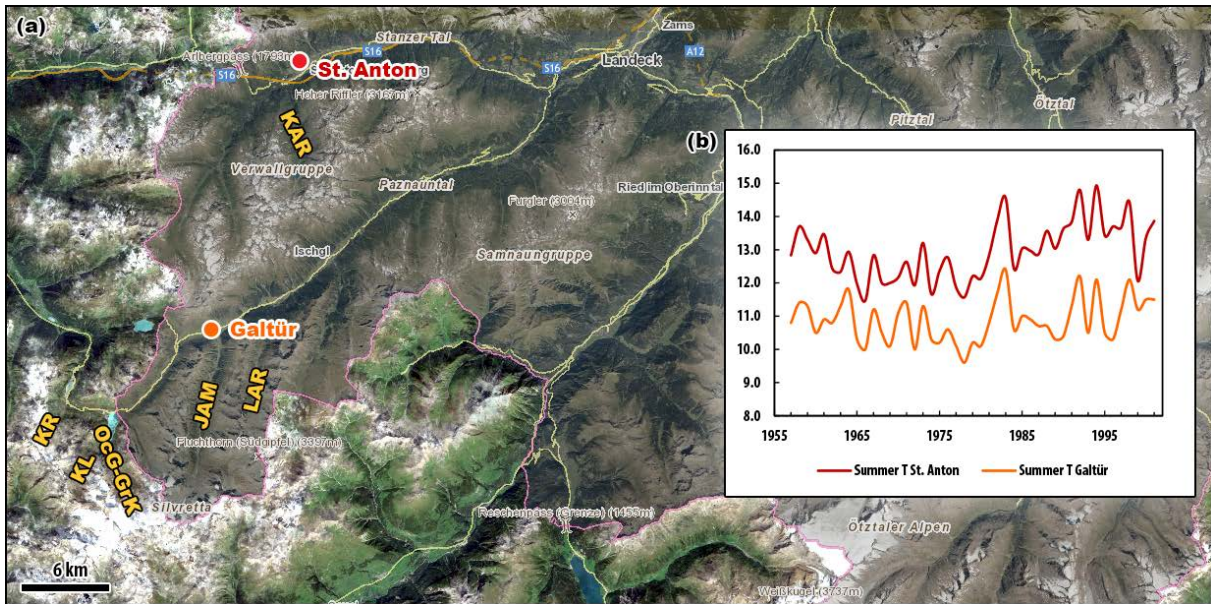
670 B1: Overview of Silvretta and Verwall regions addressed in local correlation of moraine records (section 5.2.2). (a) ^{10}\text{Be} moraine records generated in the following valleys: KAR – Kartell (Ivy-Ochs et al., 2006), KL – Kloistertal and KR – Kromertal (Moran et al., 2016b), OcG-GrK – Ochsental/Grüne Kuppe (Braumann et al., 2020), JAM – Jamtal and LAR – Laraintal (this study). Locations of meteorological stations in the Verwall region (St. Anton, station #14300) and in the Silvretta region (Galtür; homogenized HISTALP data), (Auer et al., 2007). Distance between the two stations amounts to approximately 20 km. Orthophoto accessed via https://maps.tirol.gv.at , © Land Tirol. (b) Summer (JJA) temperature time series (1957–2001) from the two stations that exhibit similar trends in the period between 1957–2001 (data provided by Austrian Weather Service ZAMG). 675
