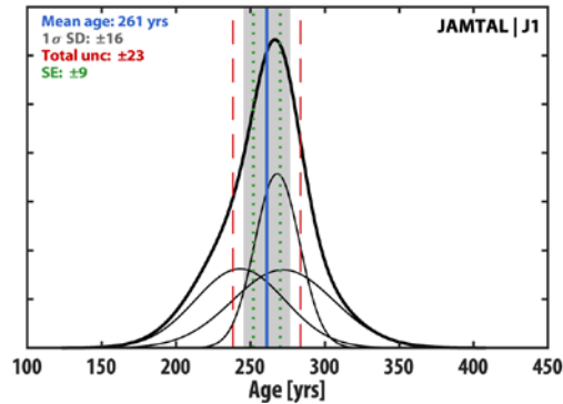
325 Figure 6: Kernel plot of LIA ages produced from boulders embedded in the historical moraine at Jamtal. The gray-shaded bar illustrates the 1 \sigma Standard Deviation (SD) of the landform age calculated from analytical uncertainties of individual samples. Red dashed lines add the production rate uncertainty and the uncertainty of the carrier concentration to the 1 \sigma SD and indicate the total uncertainty. Green dotted lines show the Standard Error (SE), which describes the dispersion of different sample means from the population mean.
