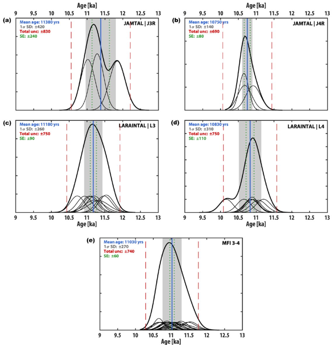
370 Figure 7: Kernel plots of Holocene moraine ages. Left column (a) and (c): inner dated EH moraines at Jamtal and Laraintal. Right 375 column (b) and (d): outermost dated EH moraines at Jamtal and Laraintal. (e) Synthesis of moraine ages across both valleys grouped to Moraine Formation Intervals (MFI) MFI 3-4 yielding an age of 11,030 \pm 740 yrs rounded to 11.0 \pm 0.7 ka ( n=19 ; outliers: JAM-18- 03 and LAR-18-03). Gray-shaded bars illustrate 1\sigma Standard Deviations (SD) of landform age uncertainties calculated from analytical uncertainties of individual samples. Red dashed lines add the production rate uncertainty (c. 6.3 %) and the uncertainty of the carrier concentration to the 1\sigma SD and indicate total uncertainties, which results in conservative uncertainty estimates. Green dotted lines indicate Standard Errors (SE).
