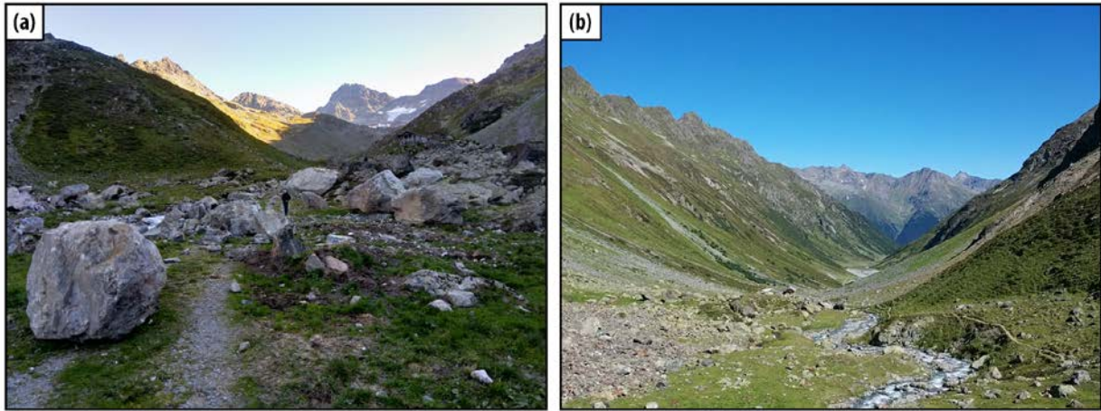
665 A4: Laraintal. (a) Fresh rockfall deposits (2019) in the Zollhütte area. Note person at the center of the photograph for scale. (b) Zollhütte area (L5); unweathered scree on the left side of the photograph; mass movement slab to the right of the hiking trail; fresh rockfall path behind the slab.
