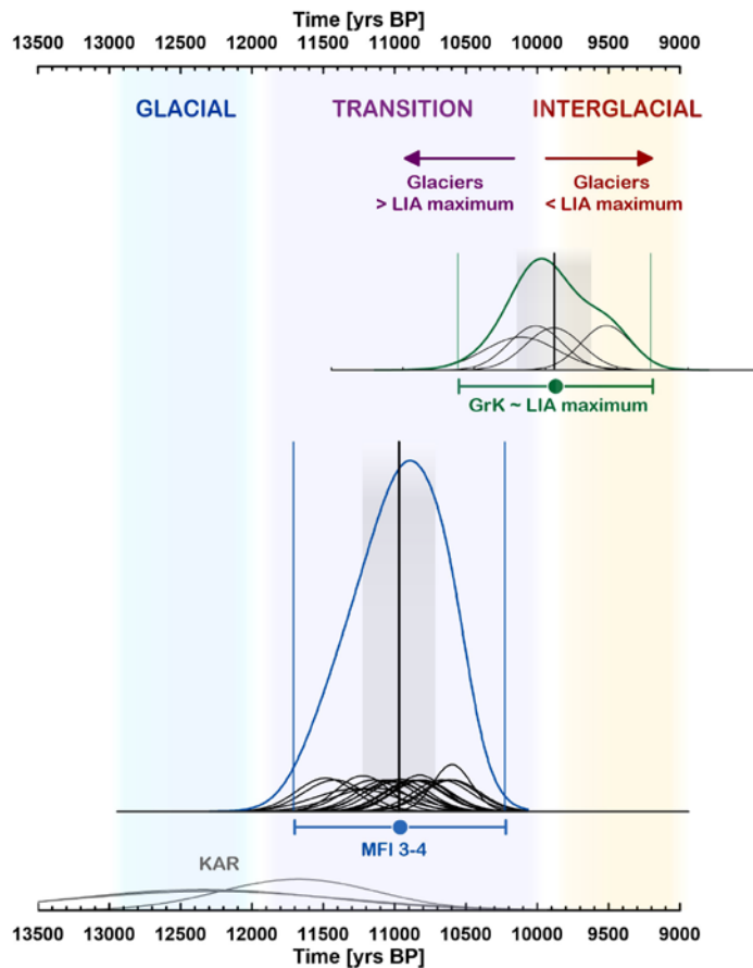
530 Figure 10: Glacier retreat during the transition from glacial to interglacial conditions evidenced in moraine chronologies from the Silvretta and Verwall regions. KAR – Kartell moraines (Ivy-Ochs, 2015; Ivy-Ochs et al., 2006), site is located approximately 15-20 km NE of Jamtal and Laraintal. MFI 3-4 described in this study. GrK – Grüne Kuppe moraine identified in the adjacent Ochsental suggesting LIA-like glacier extents around 10,000 years (Braumann et al., 2020).
