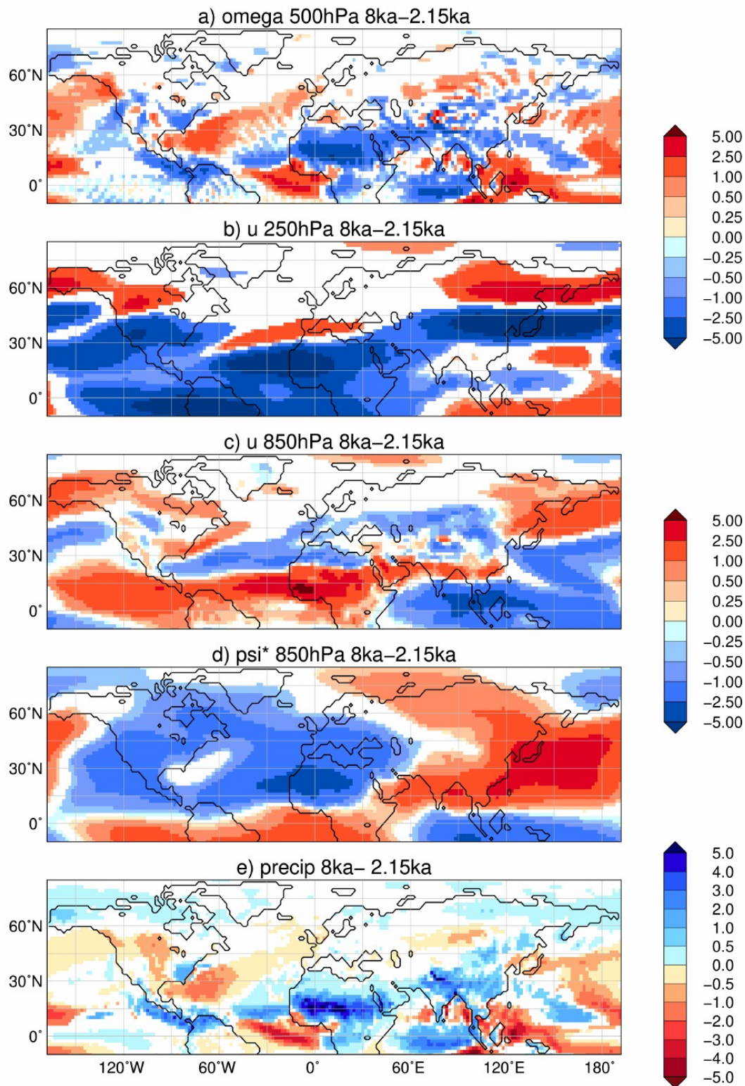
Figure 8: Simulated difference in June to August (JJA) mean climate in the model for the time-slice 8ka b2k compared to 2.15ka b2k, i.e. a) vertical velocity (omega) in 500hPa [ 10^{-2} m/s] with blue colour showing increased uplift during 8ka b2k; b) upper-tropospheric zonal wind (u) in 250hPa [m/s] with blue colours indicating enhanced easterly wind; c) low-level zonal flow (u) in 850hPa [m/s]; d) zonal anomaly in lower tropospheric streamfunction (psi*, in 10^7 m 2 /s) reflecting the change in standing waves, with blue colours indicating increased cyclonic circulation at 8ka b2k compared to 2.15ka b2k; and e) mean seasonal precipitation [mm/d] with blue colours showing enhanced precipitation during 8ka b2k. Only significant changes are shown (t-test, 99% confidence interval).
