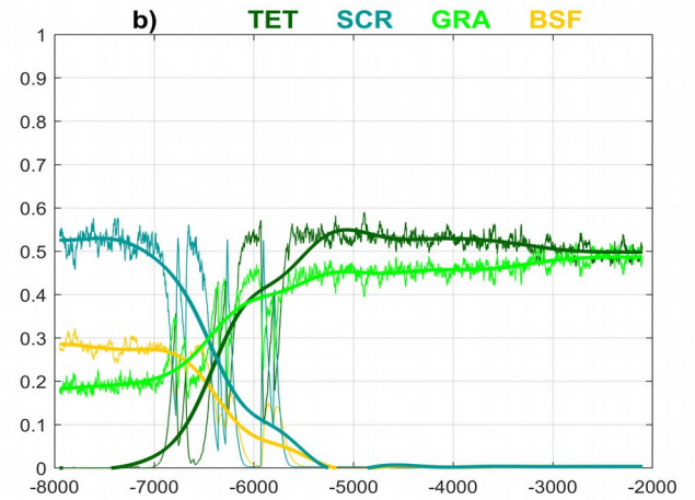
Figure 13: Examples of rapid transitions between simulated PFTs in a grid cell in East Siberia (left, region 2 in Fig. 12) and in South Asia (right, region 4 in fig. 12). The PFTs are EET: extratropical evergreen trees, EDT: extratropical deciduous trees, TET: tropical evergreen trees, SCR: shrubs (in this location, rain-green shrubs), GRA: grass, BSF: bare soil fraction. The thin lines are annual values of fractional vegetation coverage, and the thick lines are filtered time series using a Butterworth filter of order 5 with a low-pass filter of 500 years.
