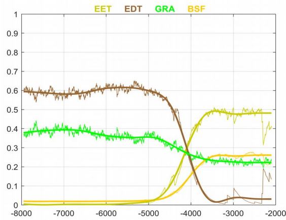
Figure 13: Examples of rapid transitions between simulated PFTs in a grid cell in East Siberia (left, region 2 in Fig. 12) and in South Asia (right, region 4 in fig. 12). The PFTs are EET: extratropical evergreen trees, EDT: extratropical deciduous trees, TET: tropical evergreen trees, SCR: shrubs (in this location, rain-green shrubs), GRA: grass, BSF: bare soil fraction. The thin lines are annual values of fractional vegetation coverage, and the thick lines are filtered time series using a Butterworth filter of order 5 with a low-pass filter of 500 years.
