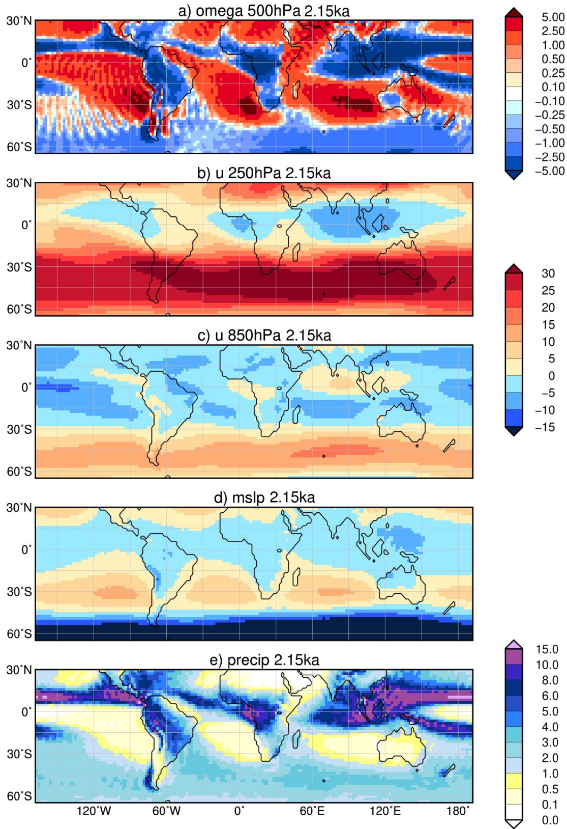
Figure B3: Simulated SON mean climate at 2.15ka b2k, i.e. a) vertical velocity (omega) in 500hPa [ 10^{-2} m/s] with blue colour showing uplift; b) upper-tropospheric zonal wind (u) in 250hPa [m/s] with blue colours indicating easterly wind; c) low-level zonal flow (u) in 850hPa [m/s]; d) mean sea level pressure anomaly [hPa] to standard atmospheric mean pressure (here 1013.25hPa), with blue colours indicating low-pressure systems; and e) mean seasonal precipitation [mm/d].
