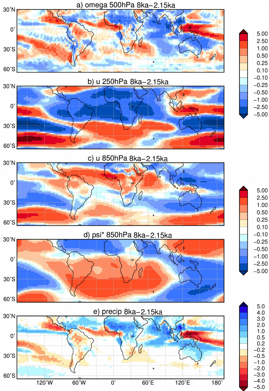
Figure 10: Simulated difference in September to November (SON) mean climate in the model for the time-slice 8ka b2k compared to 2.15ka b2k, i.e. a) vertical velocity (omega) in 500hPa [10^{-2} \text{ m/s}] with blue colour showing increased uplift during 8ka b2k; b) upper-tropospheric zonal wind (u) in 250hPa [\text{m/s}] with blue colours indicating enhanced easterly wind; c) low-level zonal flow (u) in 850hPa [\text{m/s}] ; d) zonal anomaly in lower tropospheric streamfunction (psi*, in 10^7 \text{ m}^2/\text{s} ) reflecting the change in standing waves, with blue colours indicating increased cyclonic circulation at 8ka b2k compared to 2.15ka b2k; and e) mean seasonal precipitation [\text{mm/d}] with blue colours showing enhanced precipitation during 8ka b2k.
