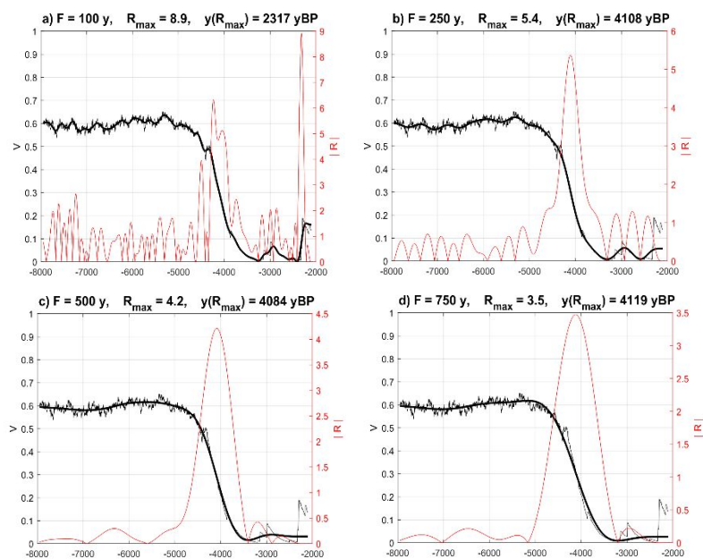
Figure C1: effect of filtering on R_{\max} .
