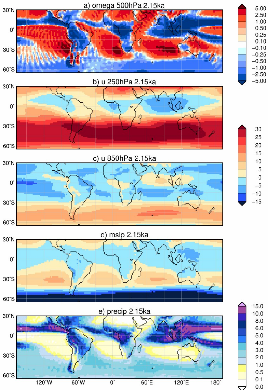
Figure B3: Simulated SON mean climate at 2.15ka b2k, i.e. a) vertical velocity ( \omega ) in 500hPa [ 10^{-2} m/s] with blue colour showing uplift; b) upper-tropospheric zonal wind ( u ) in 250hPa [m/s] with blue colours indicating easterly wind; c) low-level zonal flow ( u ) in 850hPa [m/s]; d) mean sea level pressure anomaly [hPa] to standard atmospheric mean pressure (here 1013.25hPa), with blue colours indicating low-pressure systems; and e) mean seasonal precipitation [mm/d].
