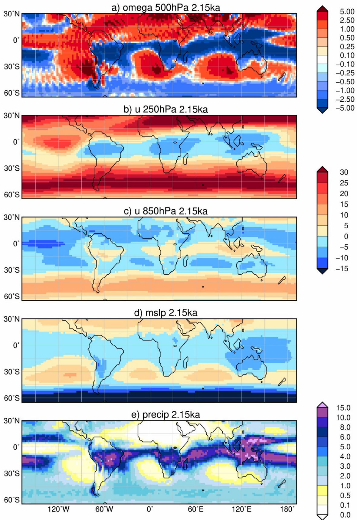
Figure B4: Simulated DJF mean climate at 2.15ka b2k, i.e. a) vertical velocity (omega) in 500hPa [ 10^{-2} m/s] with blue colour showing uplift; b) upper-tropospheric zonal wind (u) in 250hPa [m/s] with blue colours indicating easterly wind; c) low-level zonal flow (u) in 850hPa [m/s]; d) mean sea level pressure anomaly [hPa] to standard atmospheric mean pressure (here 1013.25hPa), with blue colours indicating low-pressure systems; and e) mean seasonal precipitation [mm/d].
