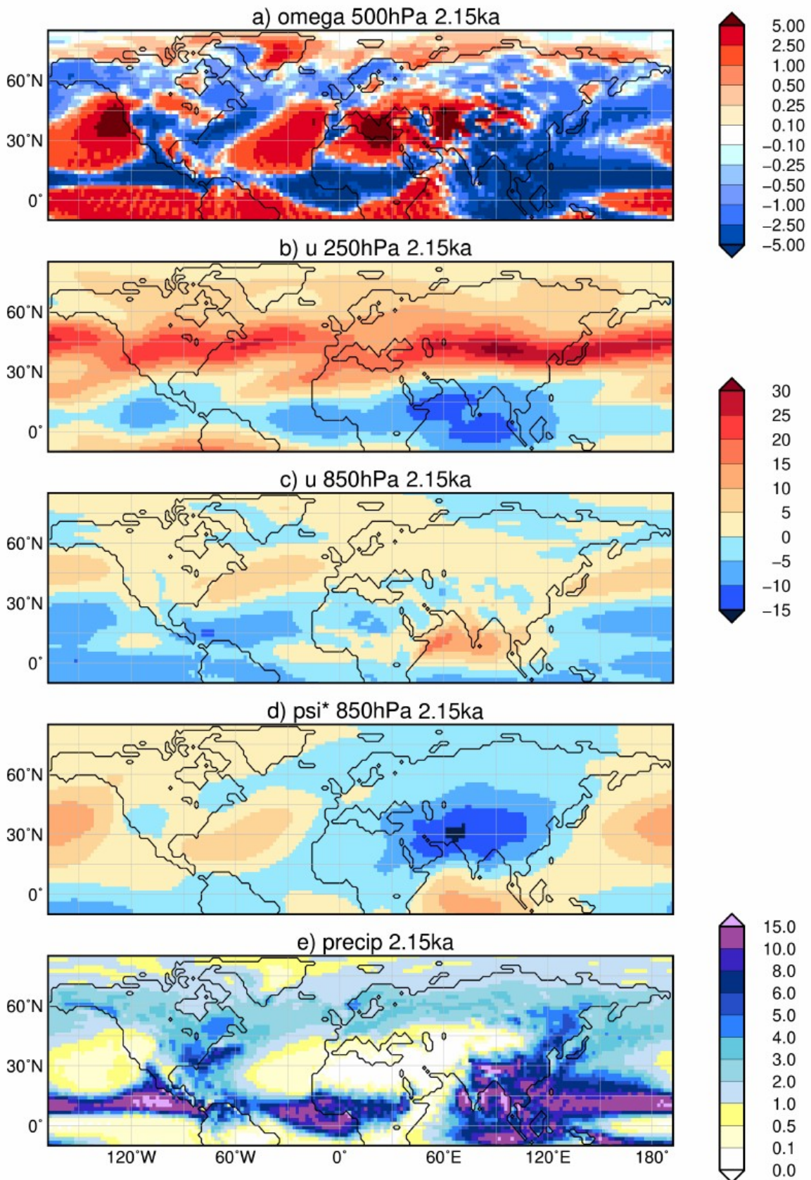
Figure B2: Simulated JJA mean climate at 2.15ka b2k, i.e. a) vertical velocity ( \omega ) in 500hPa [ 10^{-2} m/s] with blue colour showing uplift; b) upper-tropospheric zonal wind ( u ) in 250hPa [m/s] with blue colours indicating easterly wind; c) low-level zonal flow ( u ) in 850hPa [m/s]; d) zonal anomaly in lower tropospheric streamfunction ( \psi^* , in 10^7 m 2 /s) reflecting the standing waves, with blue colours indicating cyclonic circulation; and e) mean seasonal precipitation [mm/d]
