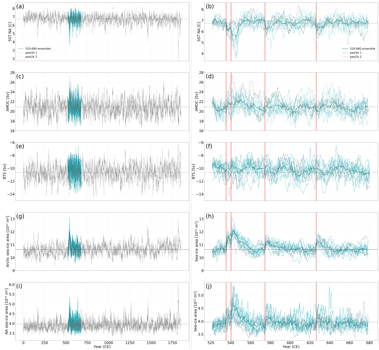
Figure A6. Time series for a/b) NA SST, c/d) AMOC, e/f) BTS, g/h) Arctic sea-ice area and i/j) NA sea-ice area for 1-1850 CE (left panels) and 521-680 CE (right panels). The red lines indicate the large volcanic eruptions in the study period, and the straight gray line is the mean of the past2k "run 0".
