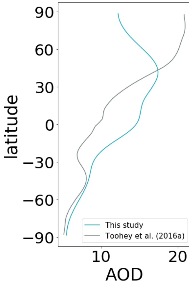
Figure A5. Comparison for accumulated AOD for 536-550 CE for the volcanic forcing from this study (eVolv2k(EVA), Toohey and Sigl, 2017) and from Toohey et al. (2016a) (their Fig. 2d, based on MAECHAM-HAM).
