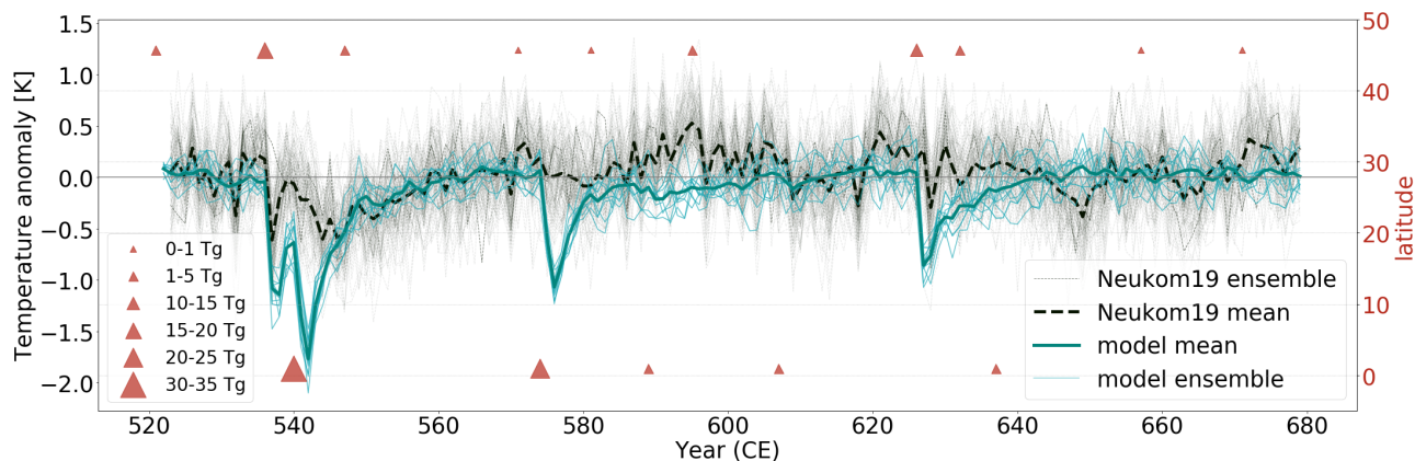
Figure A3. Model - proxy reconstruction comparison for the entire Northern Hemisphere with PAGES2k data (Neukom et al., 2019). Mean anomalies are calculated for the 1-1850 CE reference period. The red triangles represent the volcanic eruptions from the model forcing according to their latitude (tropical or NH extratropical), and the size of the triangle corresponds to the estimated range of sulphur [Tg S] injected into the stratosphere (Toohey and Sigl, 2017).
