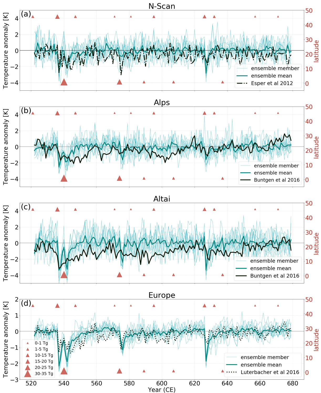
Figure A2. Model - tree ring comparison for a) Northern Scandinavia (N-Scan) (Esper et al., 2012b), b) the Alps and c) the Altai (Büntgen et al., 2016) and Europe (Luterbacher et al., 2016). Mean anomalies are calculated for the 1-1850 CE reference period. The red triangles represent the volcanic eruptions from the model forcing according to their latitude (tropical or NH extratropical), and the size of the triangle corresponds to the estimated range of sulphur [Tg S] injected into the stratosphere (Toohey and Sigl, 2017).
