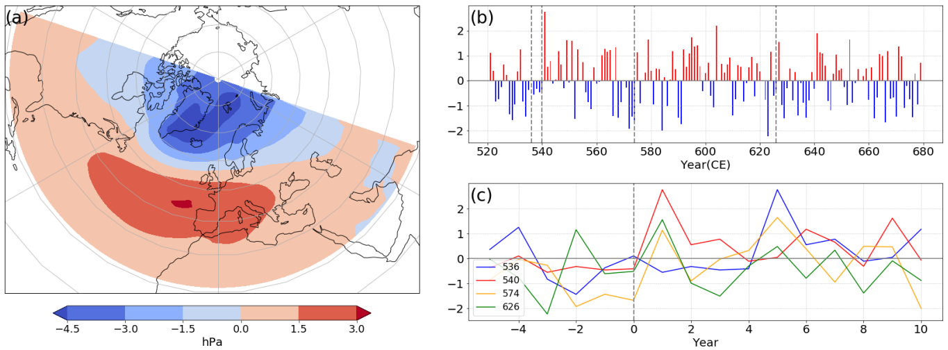
Figure A4. NAO DJF for (a) the climatological NAO signal for 1-1850 CE past2k "run 0", and the response as (b) a time series of the ensemble mean NAO index and (c) an epoch analysis of the NAO index for the four large eruptions during 520 to 680 CE. The eruption years are indicated with a dashed vertical black line in (b). DJF year 0 corresponds to December of the year before the eruption, and January to February of the year of the eruption.
