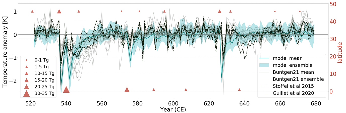
Figure 6. Model–tree ring comparison for the NH. The model 2 m air temperature anomalies are taken for land only, JJA and 40 to 75 °N. Climate model mean and the spread of the model ensemble; tree ring data for NH1 (Stoffel et al., 2015), N-VOLCv2 NH reconstruction (Guillet et al., 2020), and the mean and the ensemble of Buntgen et al. (2021). Anomalies are wrt 1-1850 CE except for the Guillet et al data which are wrt 500-1850 CE.
