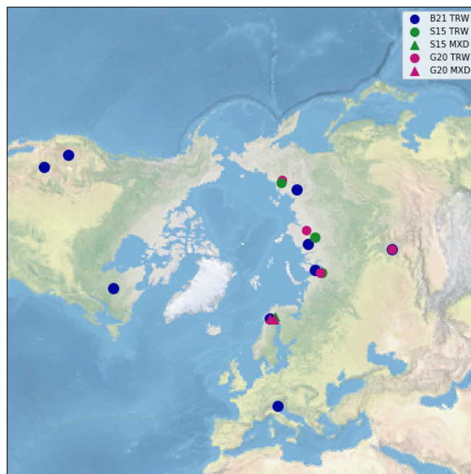
Figure A1. Locations of the (Stoffel et al., 2015, green dots), (Guillet et al., 2020, purple dots), and (Büntgen et al., 2021, blue dots) tree ring sites. For more information see also Table 2. Tree ring width data is represented by the circles and maximum latewood density by triangles.
