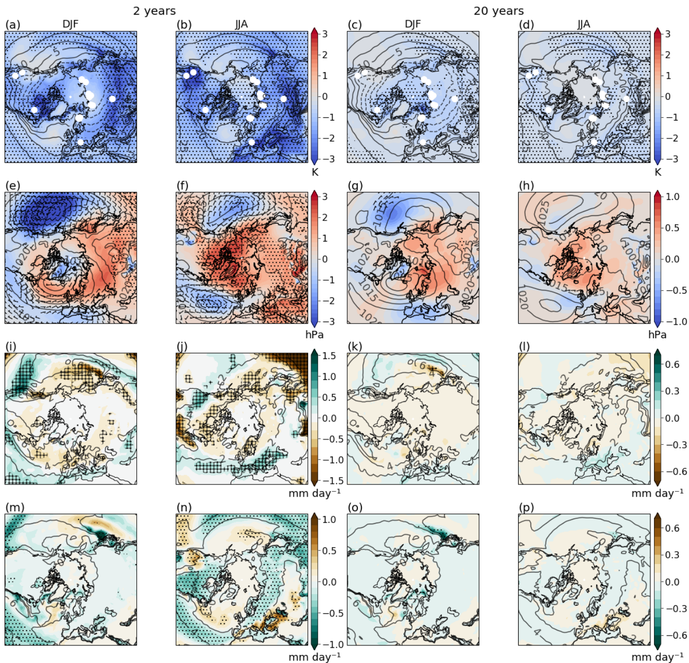
Figure 3. NH maps of boreal winter (DJF) and summer (JJA) 2 m air temperature (a-d), sea level pressure and 10 m wind (e-h), precipitation (i-l), and evaporation (m-p) for 2 years and 20 years after the eruptions, poleward of 30°N. The maps represent the ensemble mean of the 2 and 20 year mean after the four major eruptions in the study period. The two years after the eruption are year 1 and year 2 after the eruption for DJF, and the year of the eruption and one year after for JJA, respectively. All variables are given as anomalies wrt 1-1850 CE. The 1-1850 CE climatology is given as contours and the tree ring locations are represented by white dots in the 2 m air temperature maps. The ensemble standard deviation 1\sigma ( 2\sigma ) for 2 m air temperature, SLP, evaporation and precipitation are hatched (stippled). Note the different scales for the 2 year and 20 year maps and that wind anomalies are shown only for 0.5 and 1.0 m/s intervals.
