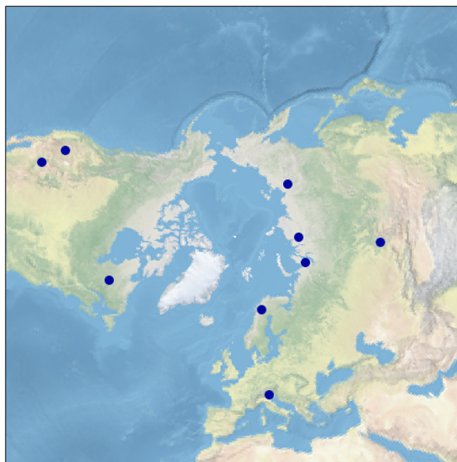
Figure A1. Locations of the tree-ring sites used in this study from Stoffel et al. (2015) and Büntgen et al. (2016); circles are TRW and triangles MXD data Büntgen et al. (2021).
