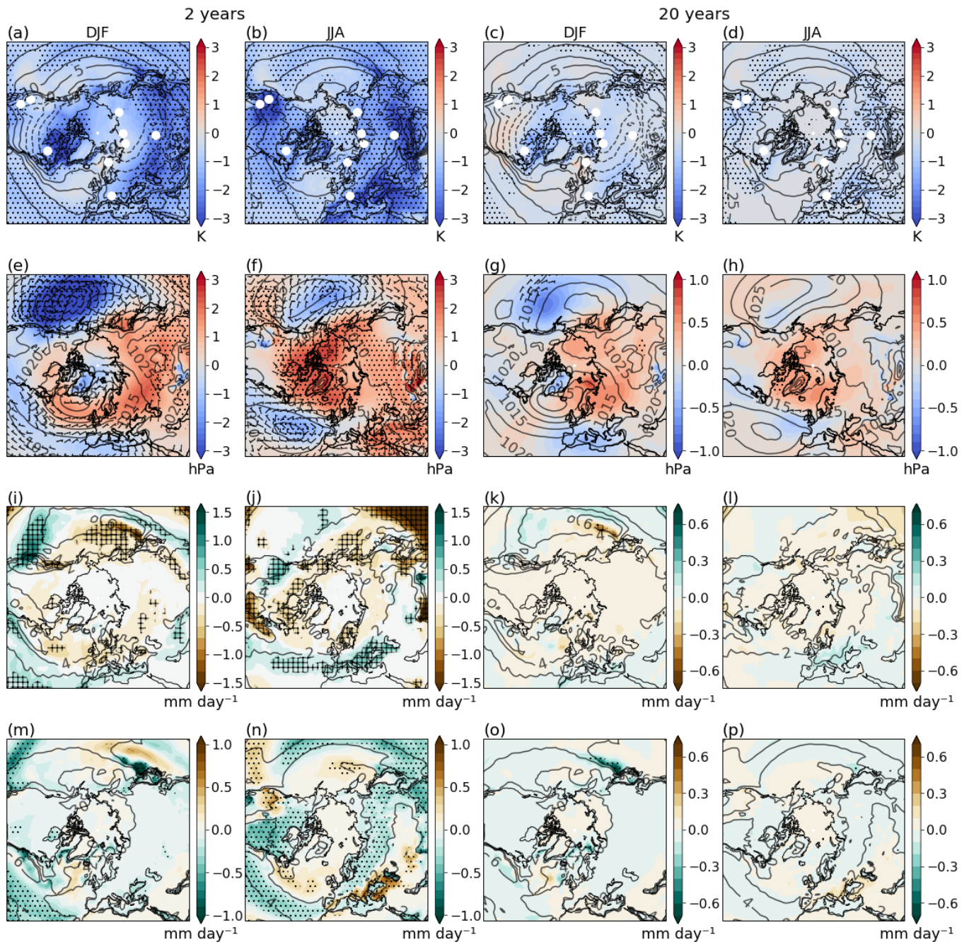
Figure 3. NH maps of boreal winter (DJF) and summer (JJA) (a–d) 2m air temperature, (e–h) sea level pressure and 10 m wind, (i–l) precipitation, precipitation (di–l) evaporation, and evaporation (em–p) March and September sea ice extent and sea ice area for 2 years and 20 years after the eruptions, poleward from of 30°N. The maps represent the ensemble mean of the 2 and 20 year mean after the four major eruptions in the study period. The two years after the eruption are year 1 and year 2 after the eruption for DJF, and the year 0 of the eruption and +one year after for JJA, respectively. All variables are given as anomalies wrt 0-1850 CE, except for sea ice extent. The 0-1850 CE climatology is given as contours and the tree-ring locations are represented by white dots (TRW) and triangles (MXD) in the 2 m air temperature maps. The 2 \sigma (ensemble standard deviation) 1 \sigma (14) standard deviations for 2m air temperature, SLP, evaporation (and precipitation) are stippled (hatched (stippled)). Note the different scales for the 2 year and 20 year maps and that wind anomalies are shown only for 0.5 and 1.0 m/s intervals.
