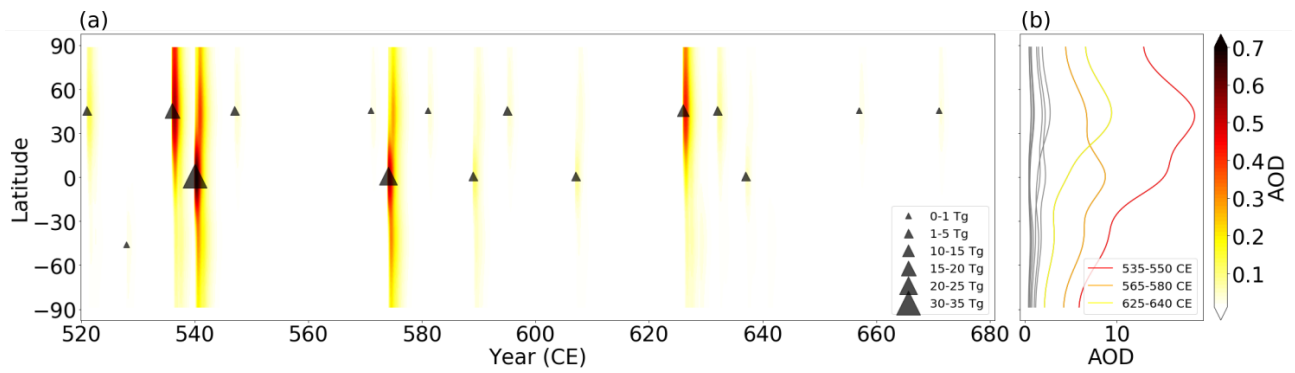
Figure 1. a) Global-zonal-Zonal mean volcanic forcing (Aerosol Optical Depth, AOD) for the study period (520-680 CE) and b) zonal mean accumulated AOD (520-680 CE) in 15 year bins from the reconstructed volcanic forcing of Toohy and Sigl (2017) . The three 15 year periods with the highest volcanic forcing are highlighted in color and labeled. The triangles in (a) highlight the zonal locations and different strength in terms of stratospheric sulfur injection of all volcanic eruptions as specified in the legend ( T_g = 10^{12} g).
