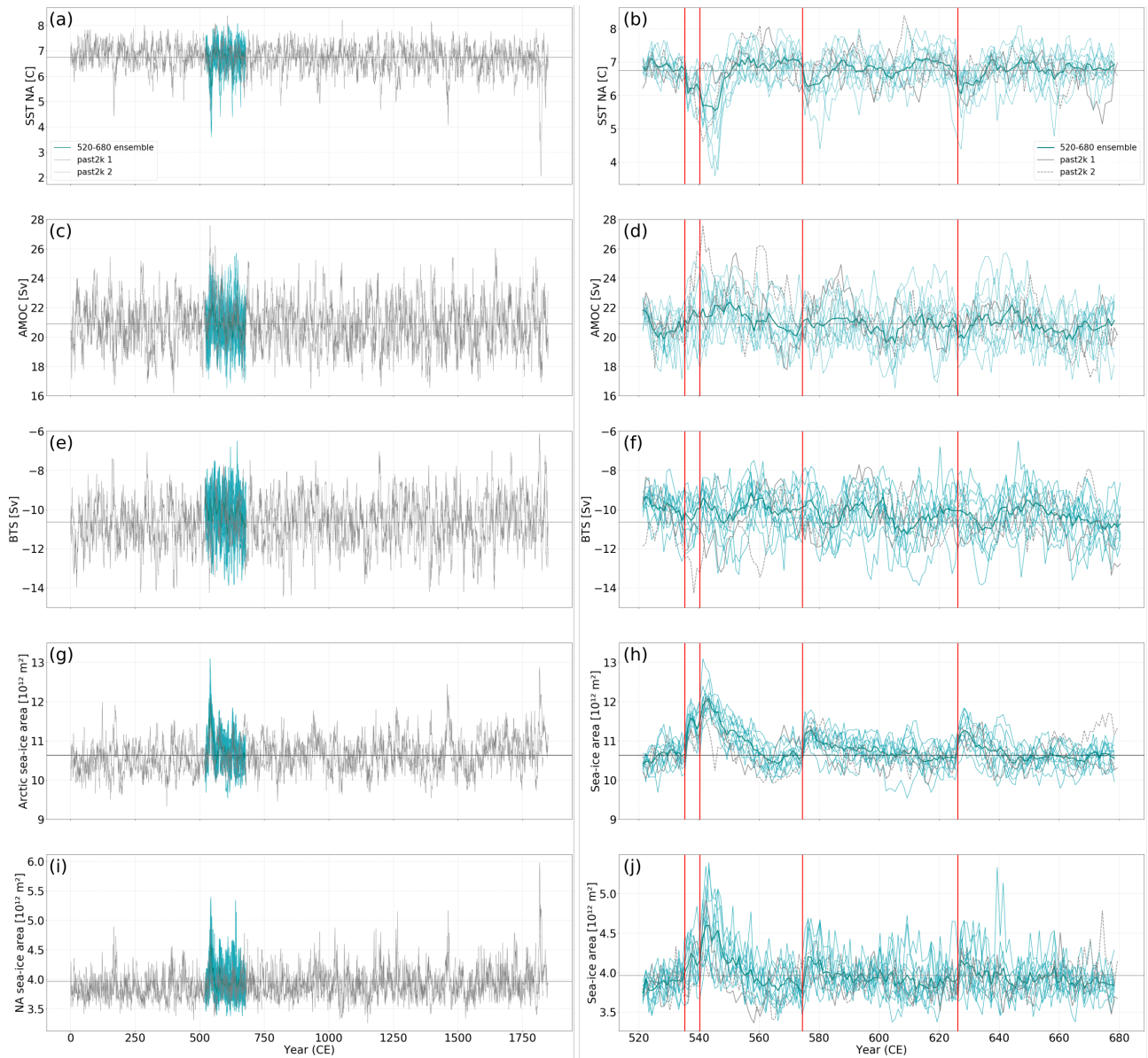
Figure A6. Time series for a/b) NA SST, c/d) AMOC, e/f) BTS, g/h) Arctic sea-ice area and i/j) NA sea-ice area for 0-1850 CE ( a-eleft panels ) and 521-680 CE ( f-right panels ). The red lines indicate the large volcanic eruptions in the study period, and the straight gray line is the mean of the past2k "run 0".
