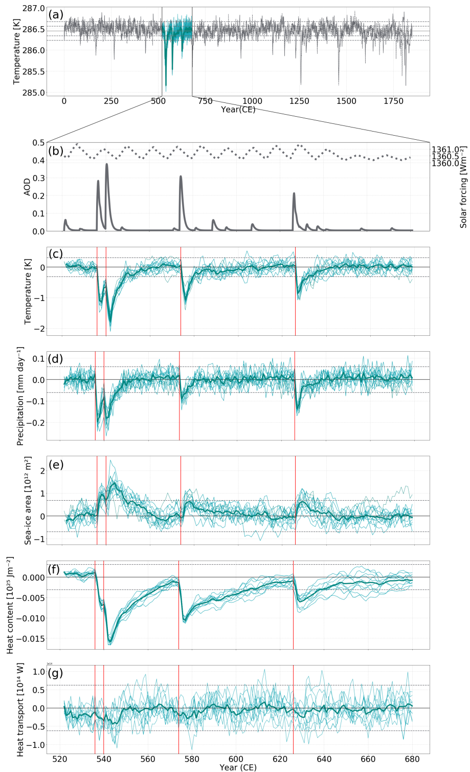
Figure 2. Time series of a) NH 2m air temperature for the two past2k and the MPI-ESM 521-680 CE ensemble runs experiments , b) global AOD volcanic forcing and solar forcing. Time series for the MPI-ESM 521-680 CE ensemble runs of c) NH 2m air temperature, d) NH total precipitation, e) Arctic sea-ice area, f) global ocean heat content for the upper 700 m, and g) Atlantic ocean heat transport at 60°N. All variables are given as anomalies wrt 0-1850 CE. The timing of the volcanic eruptions in the study period (520-680 CE) are is represented by a red line. Ensemble runs are blue and the ensemble mean is the thick blue line. The grey dashed lines indicate the 2\sigma of the control run.
