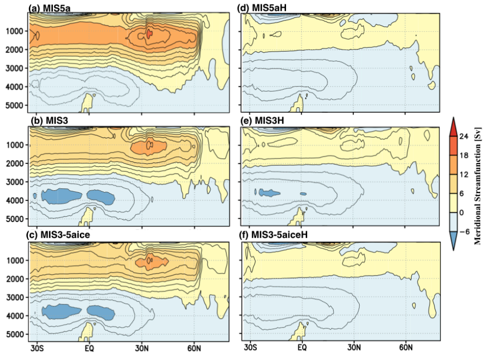
725 Climatology of the Figure 4: Climatology of the meridional streamfunction [ \text{Sv} = 10^6 \text{ m}^3 \text{ s}^{-1} ] in the Atlantic. (a) MIS5a, (b) MIS3, (c) MIS3-5aice, (d) MIS5aH, (e) MIS3H, and (f) MIS3-5aiceH. The last 100 years are used for analysis.
