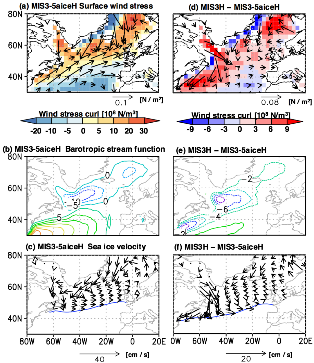
Figure 10: Comparison of surface wind and wind-driven oceanic components between MIS3H and MIS3-5aiceH. Annual mean climatology values of (a, d) surface wind stress, (b, e) barotropic streamfunction ( \text{m}^2/\text{s} ) and (c, f) sea ice velocity ( \text{cm}/\text{s} ) are shown. In (a), (b) and (c), results from MIS3-5aiceH are shown. In (d), (e) and (f), the differences between MIS3H and MIS3-5aiceH are shown. Blue contour lines in (c) and (f) show sea ice edges (15% concentration) of MIS3-5aiceH and MIS3H, respectively. The average over the last 100 years of hosing (years 401–500) is shown.
