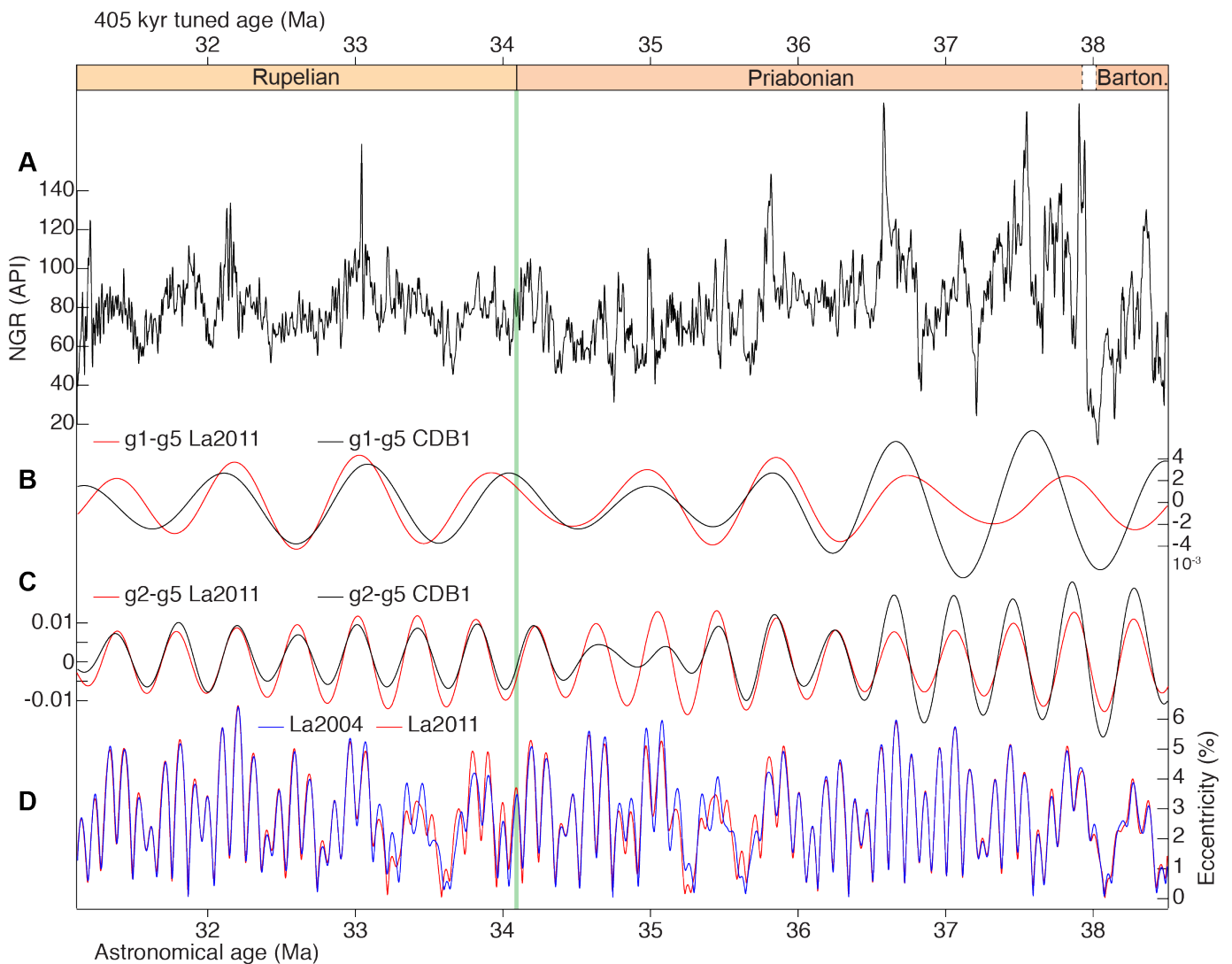
320 Figure 5_REVISIED: Astronomical calibration of CDB1 core, along with filtering at 405 kyr (g2–g5) and ~1 Myr (g1–g5) bands. (A) NGR data are tuned to a single 405 kyr sinusoid function, and then anchored at the Eocene-Oligocene boundary at 34.10 Ma. The 34.10 Ma is the age showing the best phase relationship between the tuned NGR and La2004 orbital eccentricity curve (Laskar et al., 2004) at the 405 kyr cyclicity (Fig. S9, see Sect. 4.1 for detail). (B) Bandpass filtering at ~1 Myr band. (C) Bandpass filtering at 400 kyr band. (D) Raw La2004 and La2011 orbital eccentricity data (Laskar et al., 2004, 2011). 325
