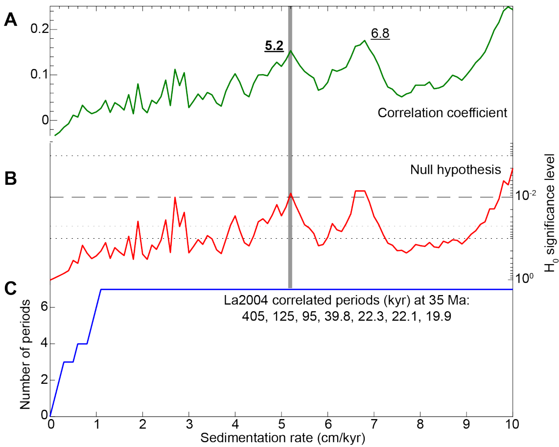
Figure 4_NEW: Statistical testing for astronomical forcing hypothesis of NGR variations, and optimal sedimentation rate for orbitally-forced NGR time series using the COCO technique (Li et al., 2018; see Methods). (A) Pearson correlation coefficient. (B) Null hypothesis H_0 . (C) Number of La2004 astronomical parameters used in the correlations (indicated). Note there are two optimal sedimentation rates at 5.2 and 6.8 cm/kyr, which have significant H_0 levels above 10^{-2} . The optimal sedimentation rate at 5.2 cm/kyr (vertical grey bar) fits the manual mean sedimentation rate (see Fig. 2B).
