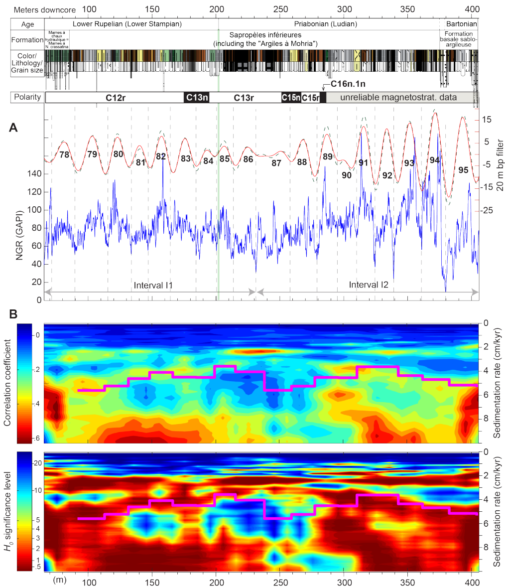
100 Figure 2_REVISÉD: (A) Integrated cyclo-magnetostratigraphy of the CDB1 drill-core. Paleomagnetic data are provided in the Supplementary Information. For sediment color, lithology and grain size, see Bauer et al., 2016. On the natural gamma-ray (NGR) data (10 cm resolution) a gaussian bandpass filter ( 0.05 \pm 0.015 cycles/m in solid line, 0.05 \pm 0.02 cycles/m in dashed line) is applied to extract the prominent cyclicity of a ~20 m wavelength, interpreted as reflecting the 405 kyr eccentricity periodicity. The numbering scheme for the 405 kyr eccentricity cycles follows the approach of Hinnov and Hilgen (2012), where eccentricity 105 maxima are counted back in time. Intervals I1 and I2 correspond to those used for time-series analysis in depth domain (Fig. 3). (B) Statistical evocative COCO outputs (see Methods). Upper panel: correlation coefficient, lower panel: Null hypothesis H_0 . Stair like curve in pink is the sedimentation rate inferred from the 405 kyr tuning of the 20 m wavelength shown in 'A'. The eCOCO parameters are 0 to 10 cm/kyr with an increment of 0.1 cm/kyr for testing sedimentation rates, window = 80 m, step = 1 m, 1000 Monte Carlo simulations. Note that the manual sedimentation rate tracks the statistically inferred eCOCO sedimentation rate, 110 except for the interval at roughly 240-280 m, where the significance is very low. This is likely due to the poorly preserved cyclicities at the transition between 405 kyr cycles 86 and 87 and cycle 88 (see Fig. 3). For the estimated optimal mean sedimentation rate over all whole studied interval, see Fig. 4.
