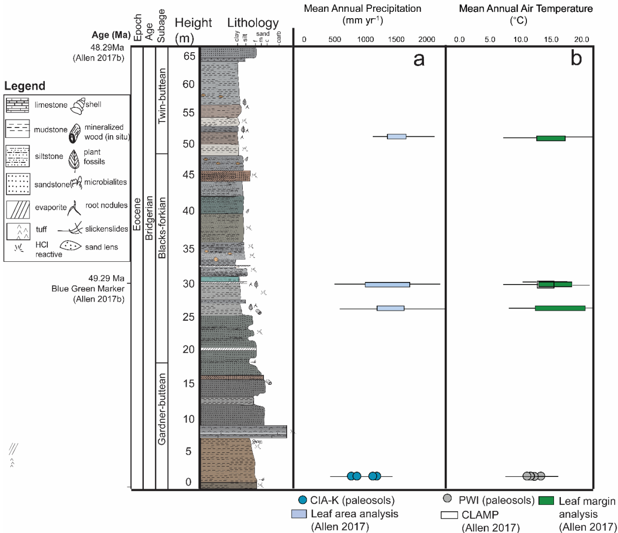
970 Figure 6: Stratigraphic column with climate proxies. (a) Reconstructed mean annual precipitation (mm yr -1 ), and (b) 975 mean annual air temperature (°C). The boxes are ranges reconstructed for physiognomic proxies, and the circles are values reconstructed using paleosols. The lines for both are established errors for the proxies used, based on the initial proxy calibrations. Errors were calculated for each estimate, and the error bars span the total range of calculated error. More information on error can be found within these proxy calibrations (e.g., Wilf 2000; Sheldon et al., 2002; Spicer et al., 2009; Gallagher & Sheldon 2013).
