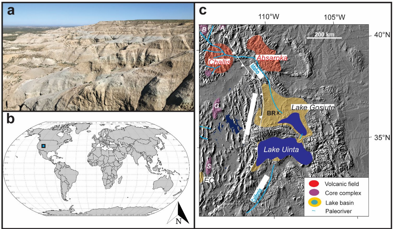
945 Figure 3: Map and profile of Blue Rim escarpment. (a) Landscape image of the escarpment from the uppermost strata. (b) Location of Blue Rim escarpment (blue square) at present, in context of the present tectonic configuration of the world using a Robinson projection map. (c) Shaded relief map of the North American Cordillera showing the paleogeographic position of the Blue Rim (BR) relative to major paleorivers, lake basins, and tectonic elements. EC refers to early Bridgerian Elderberry Canyon local fauna of Emry (1990). Core complexes occur near the Cordilleran paleodivide: B – Bitterroot; A – Anaconda; W 950 – Wildhorse; G – Albion-Raft River-Grouse Creek; S – Snake. Note that the Bridger Formation at Blue Rim represents the topsets of the Sand Butte delta (cf. Smith et al., 2008). Paleorivers summarized from Henry et al. (2012), Dickinson et al. (2012) and Chetel et al. (2011).
