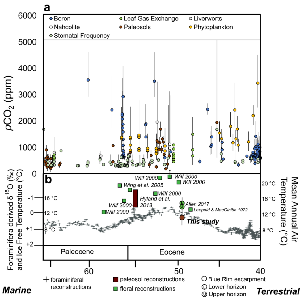
1015 Figure 11: Paleoclimate reconstructions from Blue Rim escarpment in the context of the evolution of climate from 66 to 40 Ma. (a) p\text{CO}_2 from 66 to 40 Ma based on multiple proxies compiled on paleo- \text{CO}_2 .org (McElwain 1998; Ekart et al., 1999; Pearson & Palmer 2000; Royer et al., 2001; Greenwood et al., 2003; Royer 2003; Pagani et al., 2005; Lowenstein & Demicco 2006; Fletcher et al., 2008; Zachos et al., 2008; Franks & Beerling 2009; Retallack 2009; Bijl et al., 2010; Smith et al., 2010; Grein et al., 2011; Pagani et al., 2011; Hyland & Sheldon 2013; Hyland et al., 2013; Huang et al., 2013; Franks et al., 2014; Maxbauer et al., 2014; Jagmiecki et al., 2015; Anagnostou et al., 2016; Barclay & Wing 2016; Liu et al., 2016; Kowalczyk et al., 2018; Witkowski et al., 2018; Zhang et al., 2018; Milligan et al., 2019; Steinhorsdottir et al., 2019; Haynes et al., 2020; Henehan et al., 2019; Henehan et al., 2020). (b) marine \delta^{18}\text{O} and ice-free temperature reconstructions based on foraminiferal data (Zachos et al., 2008) and mean annual air temperatures reconstructed from physiognomic (green) and paleosol (brown) proxies in the Paleocene and Eocene. Error bars are from the paleo- \text{CO}_2 .org site and associated citations, and how they were calculated can be found in these sources. 1020 1025
