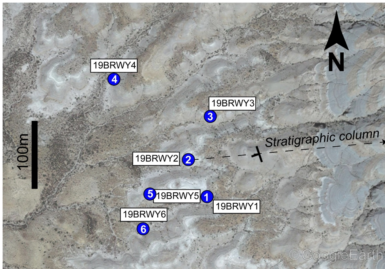
985 Figure 7: Lateral extent of paleosols. Included are paleosols 19BRWY1-6, atop image of Blue Rim escarpment topography, with a 100 m scalebar. Paleosol numbers are noted in white text on blue circles. Image taken in Google earth V 9.123.0.2 (July 2019). Wyoming, USA. 41°48'02" N, 109°35'36" W, eye altitude 2625 m. © Google Earth.
