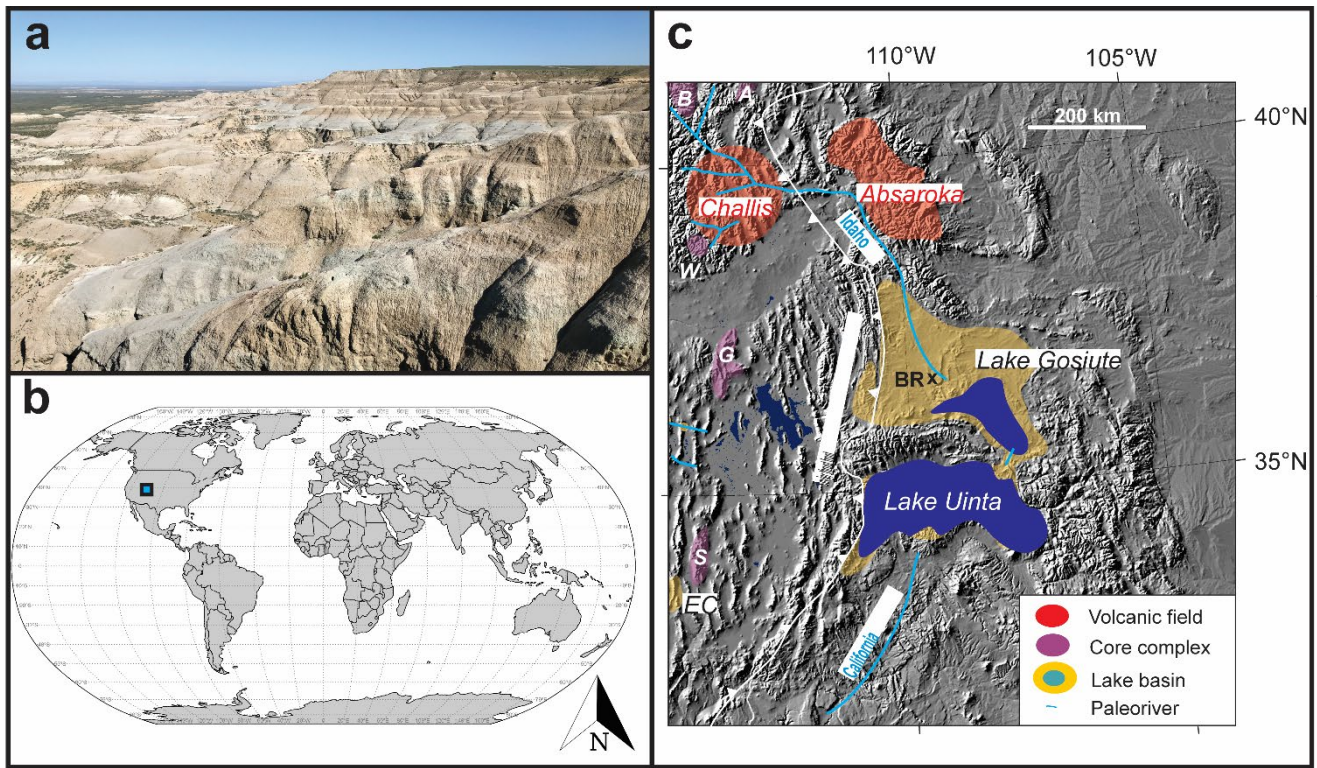
Figure 3: Map and profile of Blue Rim escarpment. (a) Landscape image of the escarpment from the uppermost strata. (b) 940 Location of Blue Rim escarpment (blue square) at present, in context of the present tectonic configuration of the world using a Robinson projection map. (c) Shaded relief map of the North American Cordillera showing the paleogeographic position of the Blue Rim (BR) relative to major paleorivers, lake basins, and tectonic elements. EC refers to early Bridgerian Elderberry Canyon local fauna of Emry (1990). Core complexes occur near the Cordilleran paleodivide: B – Bitterroot; A – Anaconda; W 945 – Wildhorse; G – Albion-Raft River-Grouse Creek; S – Snake. Note that the Bridger Formation at Blue Rim represents the topsets of the Sand Butte delta (cf. Smith et al., 2008). Paleorivers summarized from Henry et al. (2012), Dickinson et al. (2012) and Chetel et al. (2011).
