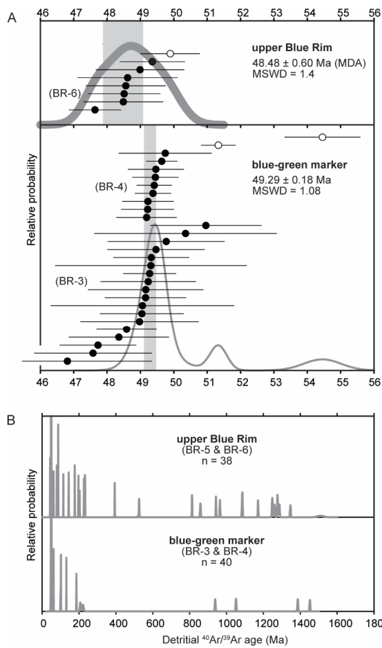
Figure 8: ^{40}\text{Ar}/^{39}\text{Ar} geochronology: a) Relative probability plots of Eocene-aged sanidine from the volcanoclastic-lacustrine blue-green marker and an overlying pumice-bearing volcanoclastic sandstone (sample BR-6); b) Relative probability plot of ^{40}\text{Ar}/^{39}\text{Ar} ages for detrital feldspar grains from the middle and upper Blue Rim, showing Phanerozoic and late Paleozoic ages characteristic of the Idaho paleoriver (cf. Chetel et al., 2011).
