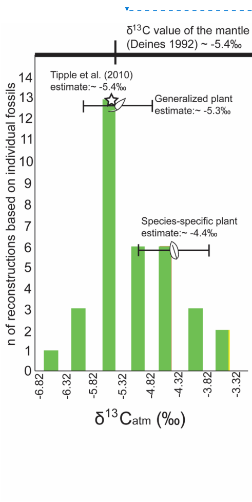
1140 Figure 9: δ 13 C atm as reconstructed from δ 13 C leaf of the Blue Rim fossil flora. Reconstructions utilized the generalized relationship between δ 13 C atm and δ 13 C plant (Arens et al. 2000; n = 34; Equation 8). The species-specific mean and standard deviation are shown (based on Lygodium and Populus fossils, n = 8), as are the generalized plant mean and standard deviation. The Tipple et al. (2010) foraminiferal reconstruction is denoted in a star, and the δ 13 C value of the mantle is shown above (Deines 1992).
