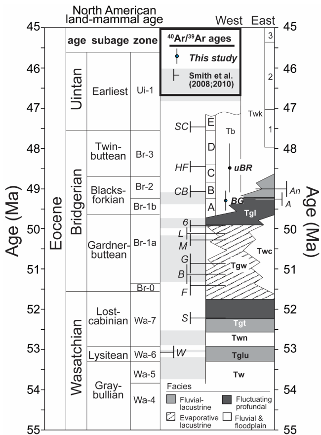
1060 Figure 1: Age model of the Eocene Wyoming. North American Land Mammal Age (NALMA) is shown for context. Upper Blue Rim is shown as “uBR” and the blue-green marker is depicted as “BG,” and both are shown with dots and error bars. Dates from Smith et al. (2008; 2010) are shown in perpendicular lines. The abbreviations included are designated as follows. Green River Formation: Tglu Luman Member, Tgt Tipton Member, Tgl Laney Member. Wasatch Formation: Tw “Main body,” Twn Niland Tongue, Twc Cathedral Bluffs Member, Tb Bridger Formation, Twk Washakie Formation. Tuff beds as measured in Smith et al. (2008; 2010) are denoted as: W Willwood, S Scheggs, R Rife, F , Firehole, B Boar, G Grey, M Main, L Layered, 6 Sixth, A Analcite, CB Church Butte, HF Henrys Fork, and SC Sage Creek.
