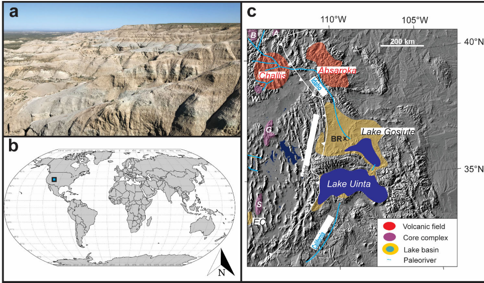
Figure 3: Map and profile of Blue Rim escarpment.
