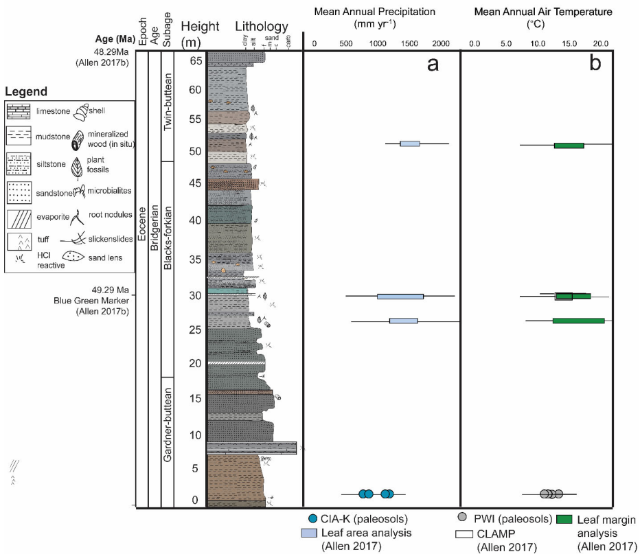
1110 Figure 6 Stratigraphic column with climate proxies. (a) Reconstructed mean annual precipitation (mm yr -1 ), and (b) mean annual air temperature (°C). The boxes are ranges reconstructed for physiognomic proxies, and the circles are values reconstructed using paleosols. The lines for both are established errors for the proxies used, based on the initial proxy calibrations. Errors were calculated for each estimate, and the error bars span the total range of calculated error. More information on error can be found within these proxy calibrations (e.g., Wilf 2000; Sheldon et al., 2002; Spicer et al., 2009; Gallagher & Sheldon 2013).
