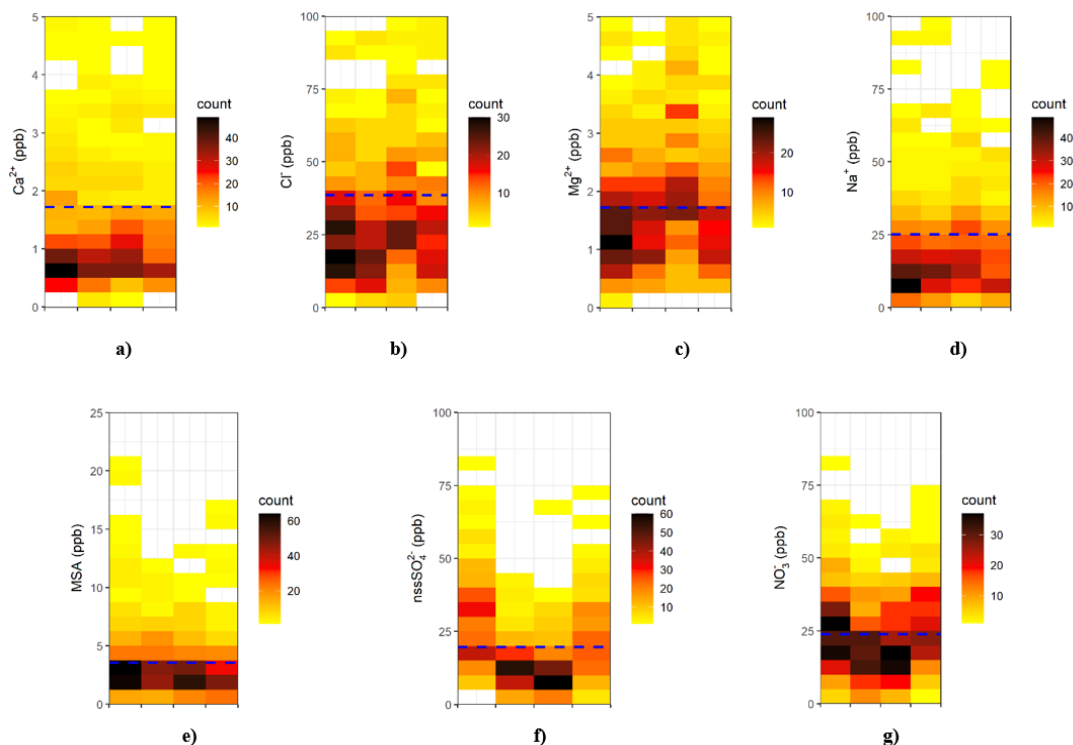
278 Figure 3: Seasonal variability of \text{Ca}^{2+} (a), \text{Cl}^- (b), \text{Mg}^{2+} (c), \text{Na}^+ (d), MSA (e), \text{nssSO}_4^{2-} (f) and \text{NO}_3^- (g) concentrations in the 279 GV7(B) ice core. Concentration bins are 3 “months” in width (JFM, AMJ, JAS, OND) and 5 ppb in height except for MSA levels 280 (1 ppb) and Calcium and Magnesium (0.25 ppb). Dashed blue lines show the average concentration of each ion in the investigated 281 time interval.
