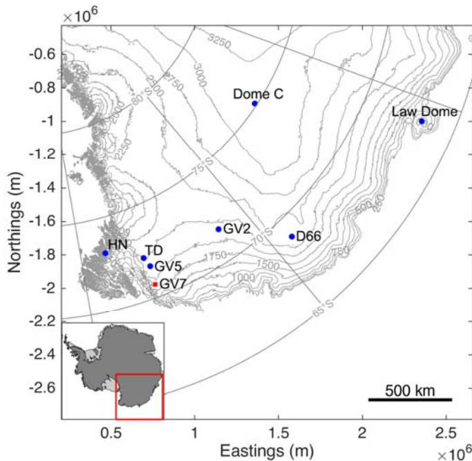
129 Figure 1: GV7 (70°41'17.1" S, 158°51'48.9" E; 1950 m a.s.l.) drilling site (red square). Hercules Nevé (HN), Talos Dome (TD), 130 GV5, GV2, D66, Dome C and Law Dome ice core drilling sites are also shown (Greene et al., 2017; Fretwell et al., 2013).
