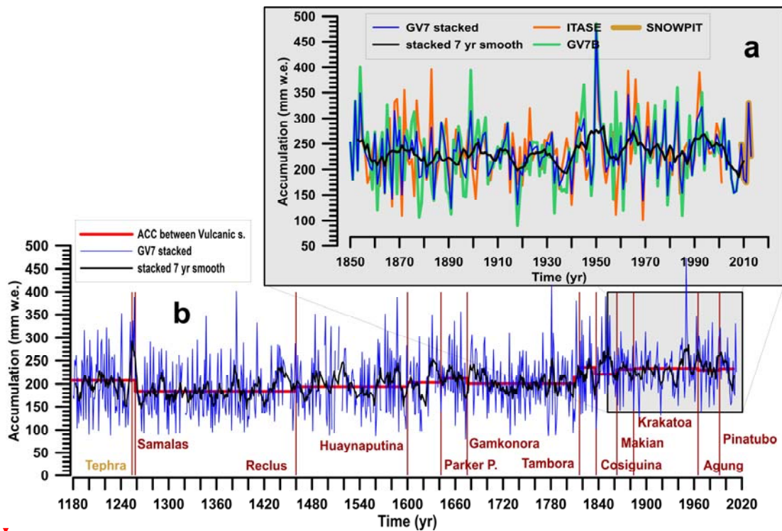
390 Figure 6: a) Time series from 1840 to 2020 CE of the GV7 snowpit (2008–2013 CE, gold line); the ITASE core (1849–2001 CE, orange line) and the GV7(B) core (1179–2009 CE, green line). Blue and black lines highlight the stacked record, obtained 391 integrating the snowpit, ITASE and GV7(B) core records, and its smoothing at 7 years, respectively. b) GV7 stacked time record 392 (1179–2013 CE) with seven-years smoothing average (black line). Red vertical bars highlight volcanic eruption horizons and red 393 line shows average accumulation rate between different volcanic events. 394
