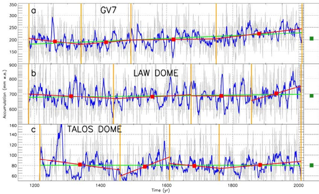
398 Figure 7: a) GV7 stacked record (gray line) with its seven yr smoothing average (blue line); green line represents trend for the 399 1179-2013 CE record. Yellow vertical bars show breaking points (1183 CE, 1341 CE, 1492 CE, 1750 CE and 2010 CE) calculated 400 following Tomé and Miranda (2004). Red lines and filled squares show partial trends and mean accumulation (with standard 401 deviation error bars) for each sub-period defined by breaking points. Green filled square with error bar highlights mean 402 accumulation at the site and its standard deviation, respectively, for the whole period (1179-2013 CE). b) Same as a) but for Law 403 Dome ice core for the period 1179-2013 CE with breaking points at 1182 CE, 1439 CE, 1674 CE, 1857 CE and 2007 CE. c) Same as 404 a) but for Talos Dome ice core for the period 1216-2010 CE with breaking points at 1216 CE, 1459 CE, 1609 CE, 1759 CE and 405 2007 CE.
