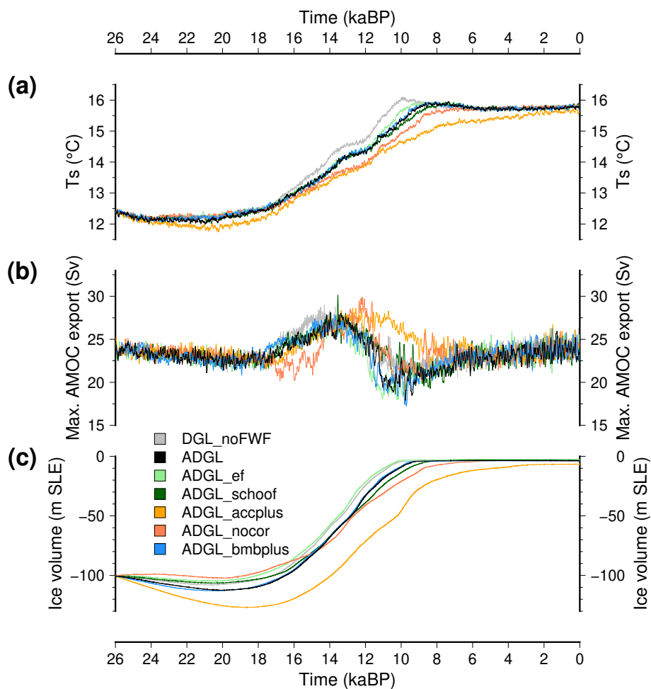
Figure 11. Time evolution of a selection of large-scale climate variables for different sensitivity experiments: (a) global mean surface temperature, (b) maximum of the Atlantic stream function and (c) simulated Northern Hemisphere ice volume. The model that does not account for the freshwater release to the ocean due to ice sheet melting is shown in grey (DGL_noFWF). The other lines are accelerated simulations (factor of acceleration of 5) and they similarly do not account for the freshwater flux to the ocean. The accelerated reference experiment is in blue (ADGL). The dark green line is in experiment in which we use the Schoof (2007) formulation of the flux at the grounding line (ADGL_schoof) instead of Tsai et al. (2015). The light green line is an experiment for which we use a larger enhancement factor (3.5 instead of 1.8, ADGL_ef). The light orange line is a version of the model with a lower c_{rad} coefficient (-50 instead of -40 W m -2 , ADGL_acplus) which induces a more positive surface mass balance. The dark orange is for an experiment in which with do not apply the spatial correction of the c_{rad} parameter (ADGL_nocor). The blue line is for an experiment with increase sub-shelf melting rate (ADGL_bmbplus).
