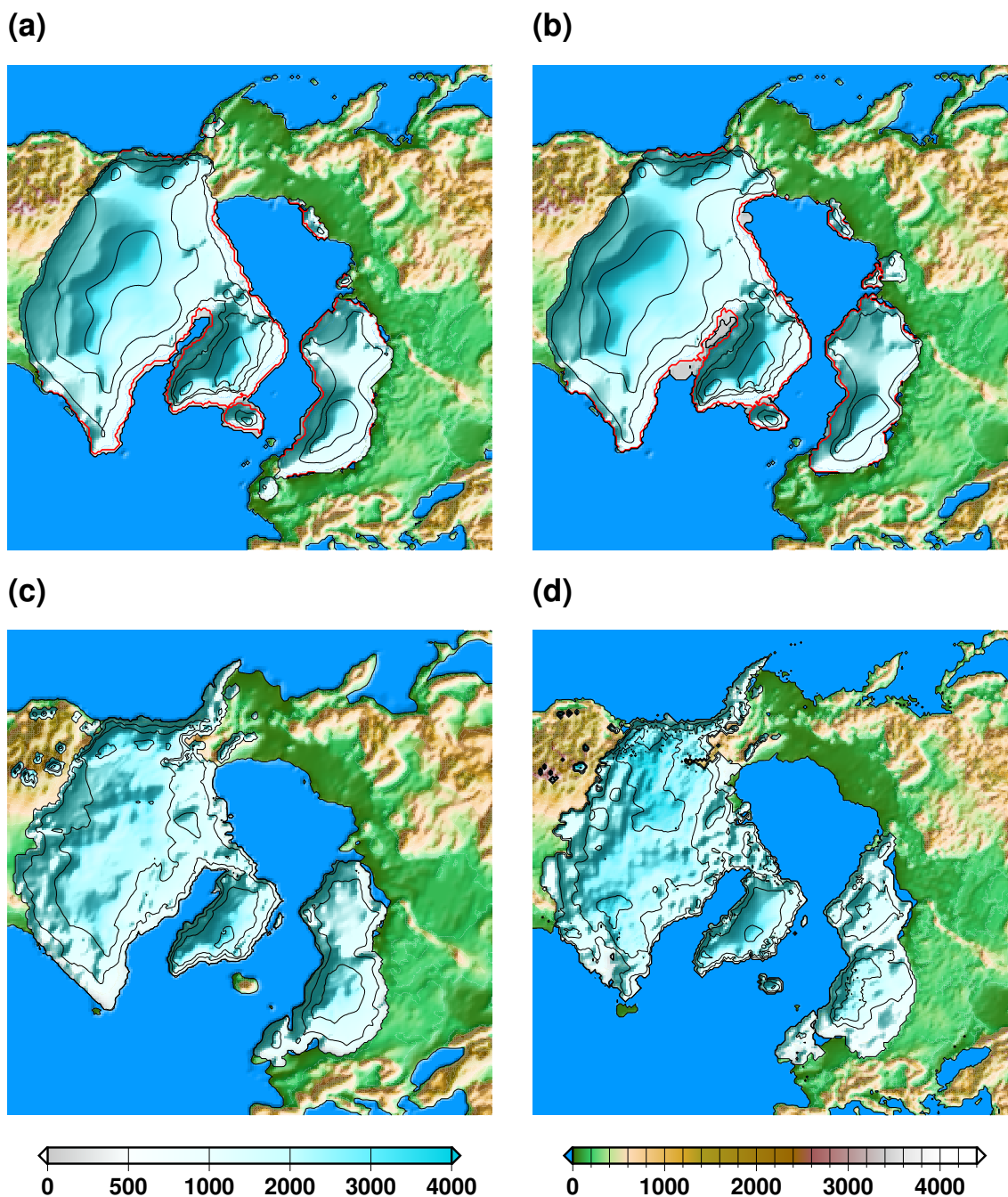
Figure 2. Surface elevation above contemporary sea level: (a) after the glacial spin-up, (b) in the reference deglaciation experiment DGL at 21 kaBP, (c) in the GLAC-1D reconstruction and (d) in the ICE-6G_C reconstruction. The colour scale is different for ice-free and ice-covered regions. The simulated ice sheet grounding line is represented by the red line while the black lines represent isocontours of ice sheet surface elevation (separated by 1000 metres).
