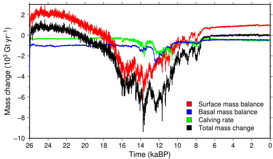
Figure 10. Time evolution of the different contributions to ice sheet mass changes. The total mass change is the sum of the surface mass balance, the basal mass balance and the calving rate.
