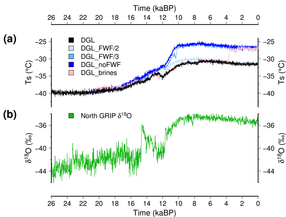
Figure 6. (a): Simulated surface temperature at the location of the North GRIP deep ice core. The reference model DGL is in black while the experiments with reduced freshwater flux to the ocean from ice sheet melting are depicted with a blue shading (dark blue for no freshwater flux). The experiments with enhanced brine formation is in pink. Here, we use a 10-yr running mean for the model results to smooth interannual variability. (b): The isotopic content in \delta^{18}\text{O} measured at North GRIP (Andersen et al., 2004), which is often considered as representative of local temperature changes.
